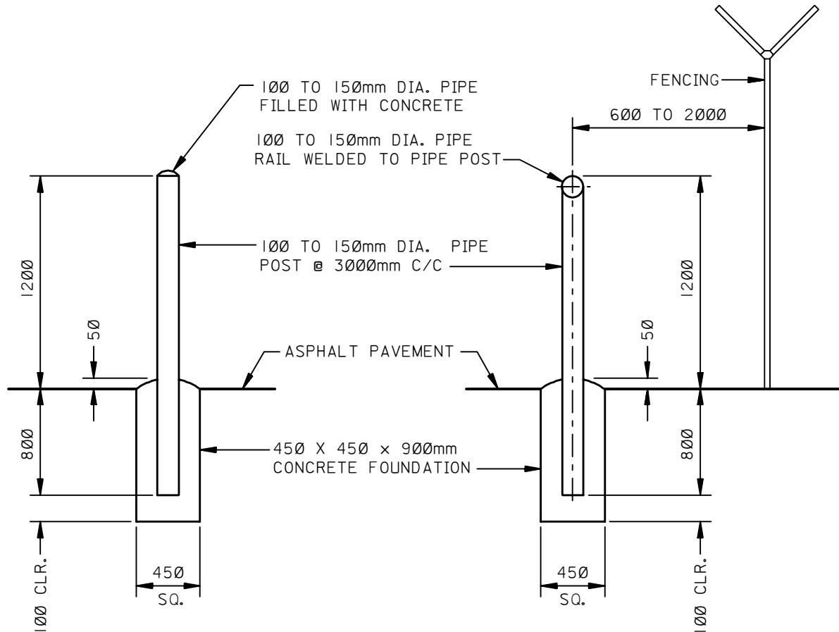
GUARD POST DETAILS
