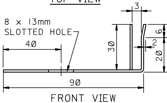
JAMB & HEAD ANCHOR TYPE A
