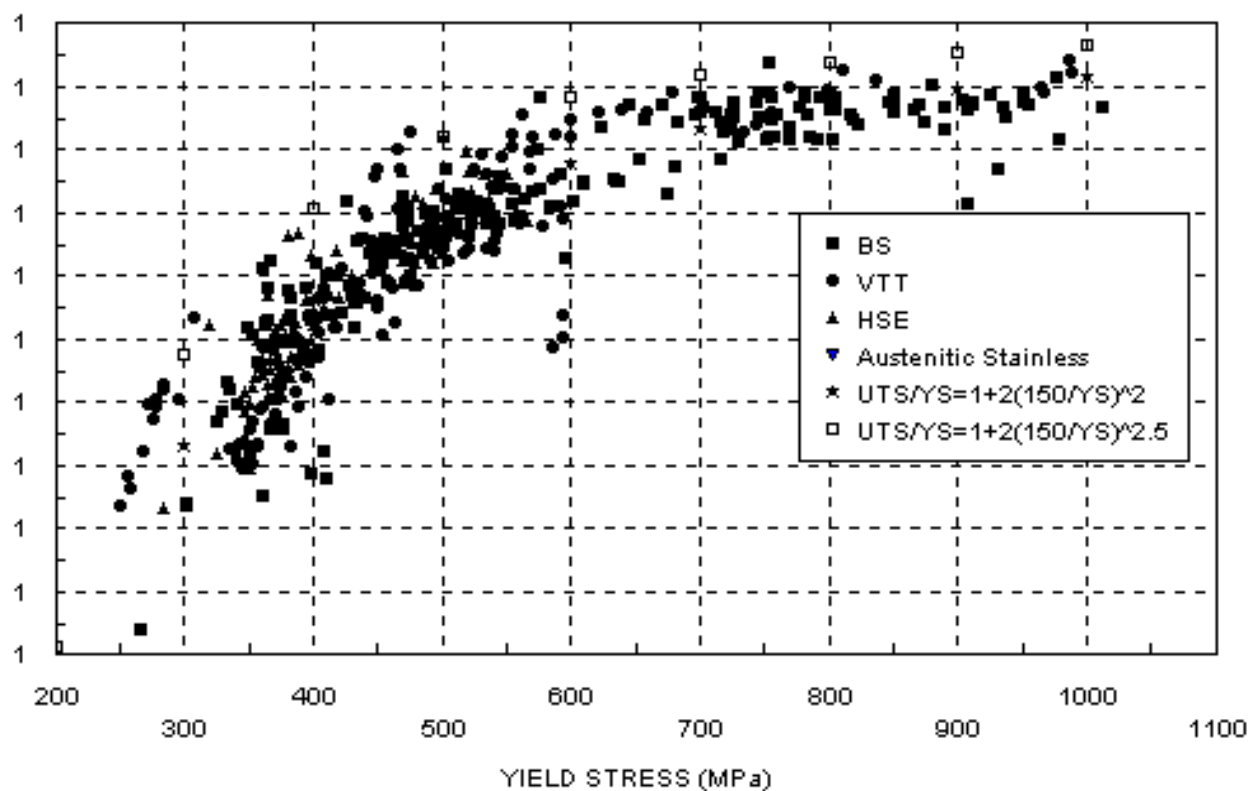
Fig. 1. Prediction of YS/UTS from Yield Stress
