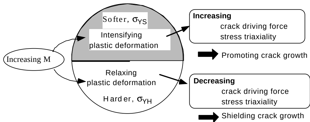
Fig. 3.16 : Schematic illustration of the strength mismatch effect on fracture behaviour for interface /sub-interface (HAZ) cracks.
