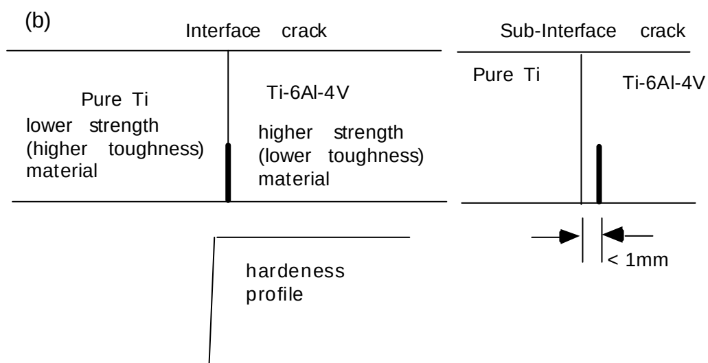
Fig. 3.1. Schematic illustrations of the specimens and hardness (strength) profiles : (a) bimaterial specimens tested at AEA, (b) bimaterial specimens (made of two Ti alloys) tested at GKSS.
