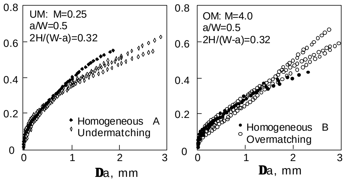
Fig. 3.9 : Uniqueness of d_5 - R curves for highly mismatched bimaterial joints in bending. The corresponding J -resistance curves are shown in Figs. 3.7.
