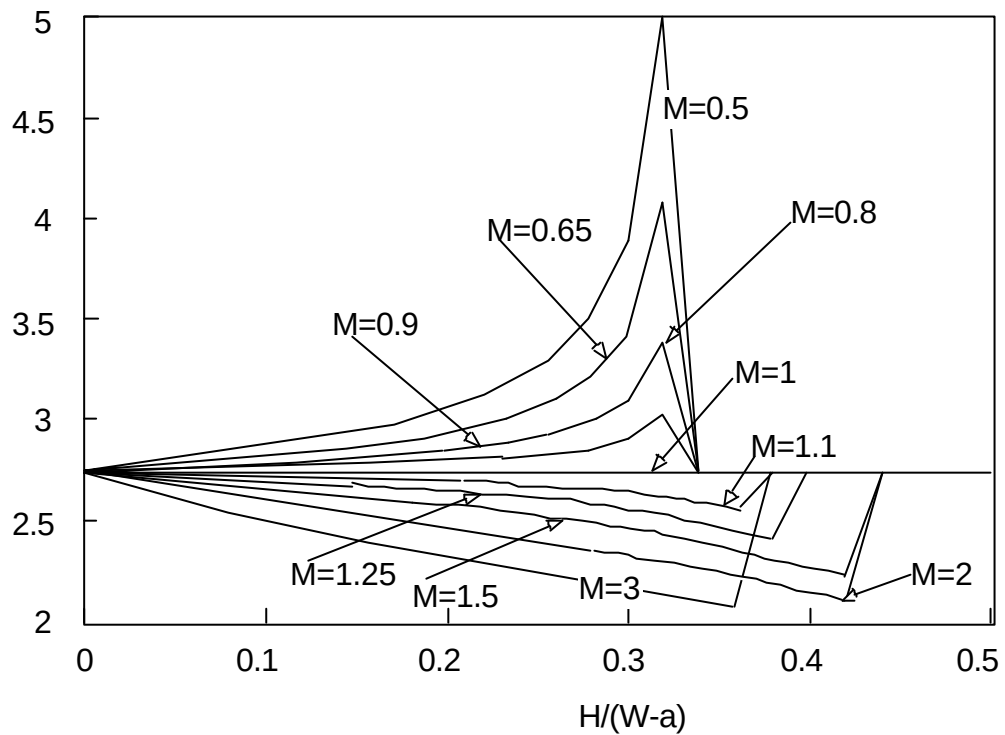
Fig. 3.6: Mismatch-corrected plastic h -factor for SENB specimens with a/W=0.5 , proposed by Horner and Eripret [1].
