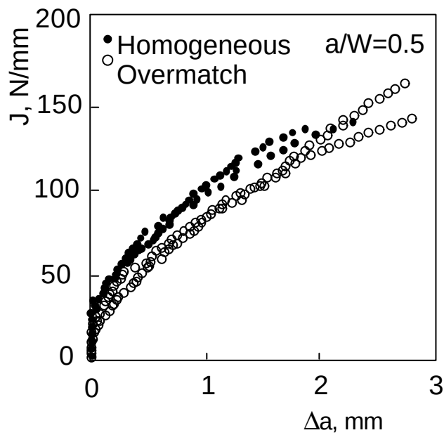
Fig. 3.7: Effect of mismatch-corrected J estimation scheme for highly overmatched specimens [1].
