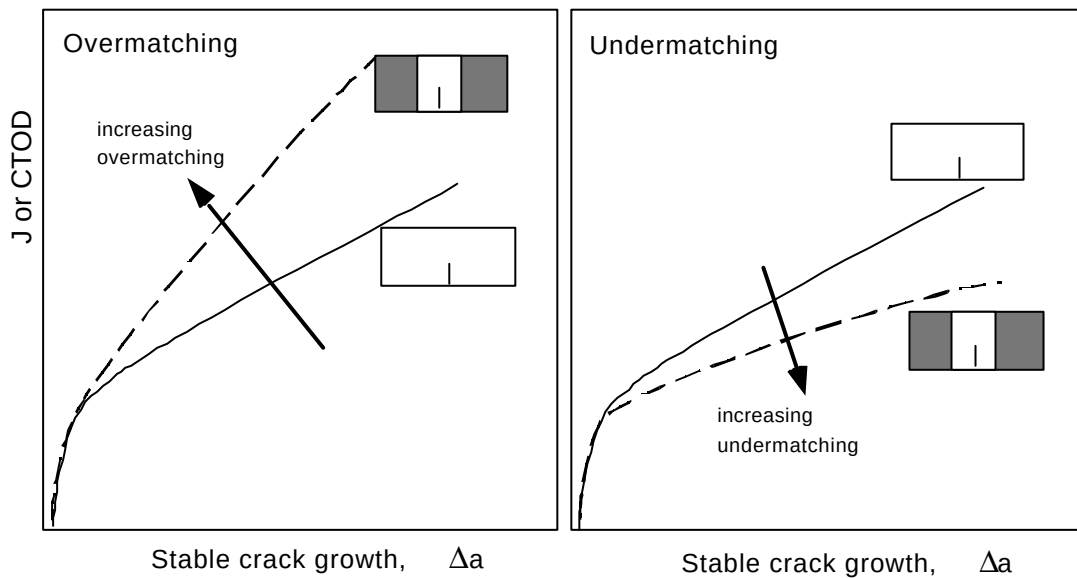
Fig. 3.2: Schematic diagrams of the strength mismatch effect of toughness resistance curves of bimaterial joints.
