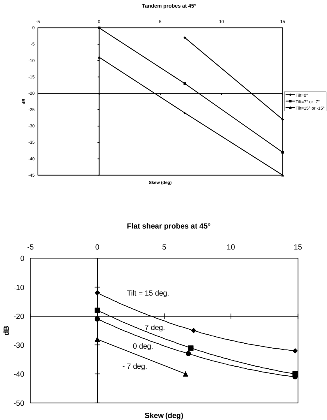
Figure 13.1: Combined effect of tilt and skew angles on the defect response in amplitude. Defects are smooth planar cracks with sharp crack tip. D=25 mm. Position in depth of the defect: 100 mm ( L=100 mm) in the vessel wall (PISC II parametric study)
