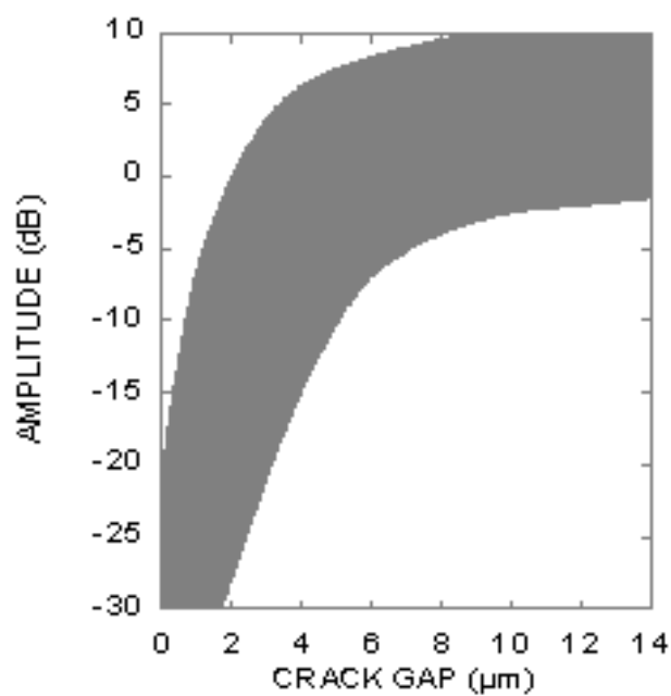
Figure 13.4: Relation between crack with (e.g. crack opening at half depth) and the amplitude response (from: Shibaura Inst. of Tech./ NPE test centre / Hitachi, Ltd, Japan)
