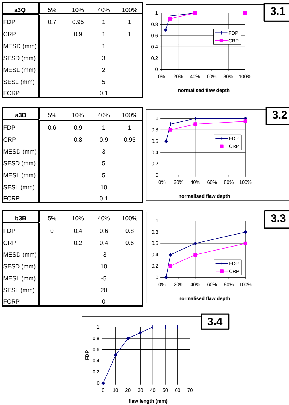
Figure 3: Inspection effectiveness for UT of large diameter piping with wall thickness less than 30 mm. Qualified procedure (a3Q), good practice (a3B), and low capability (b3B). 3.4 refers to the defect length (good practice a3B)
