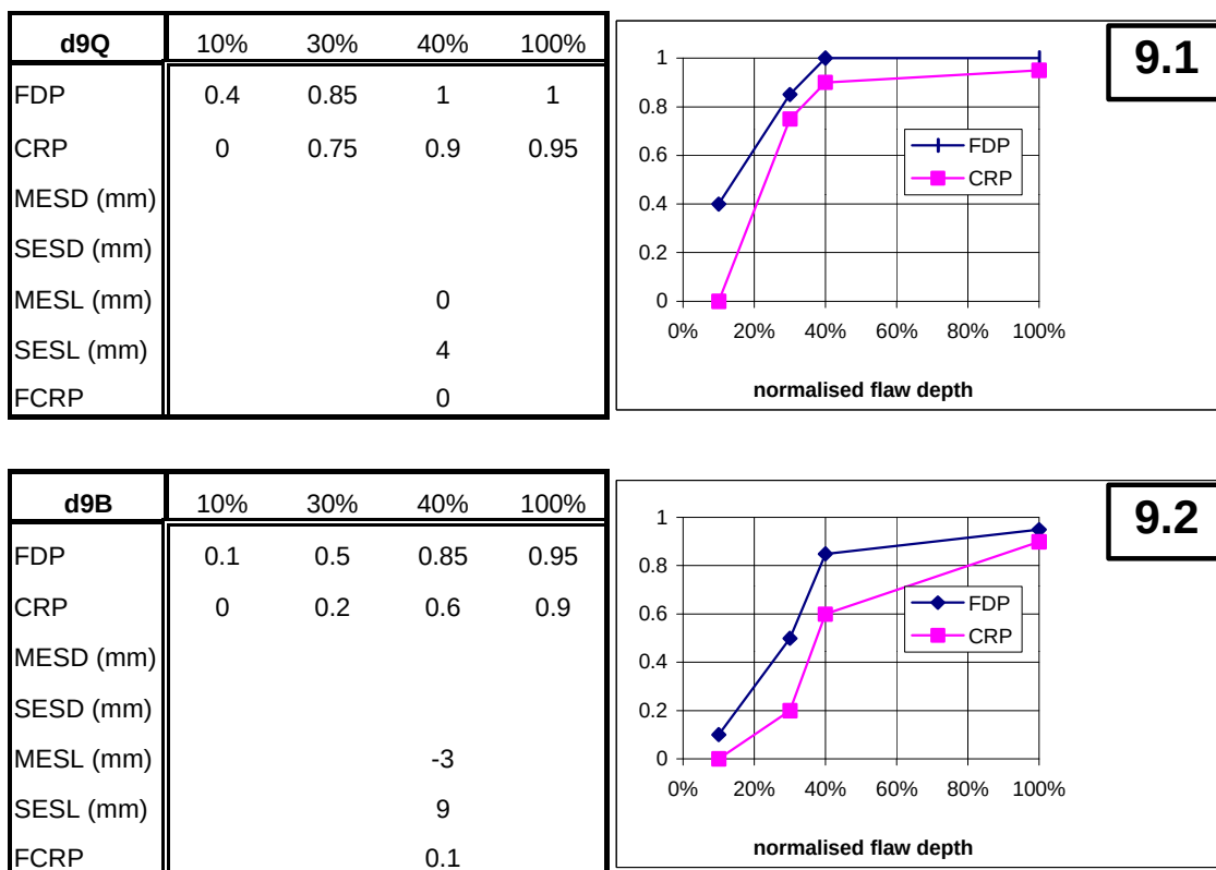
Figure 9.1-2: Inspection effectiveness for ET of austenitic steel tubes (steam generator). Cracks and planar defects only (PPD)
