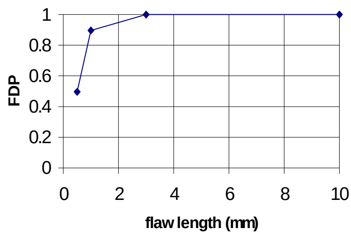
Figure 11.1 Effectiveness of ET inspection of thin plates
