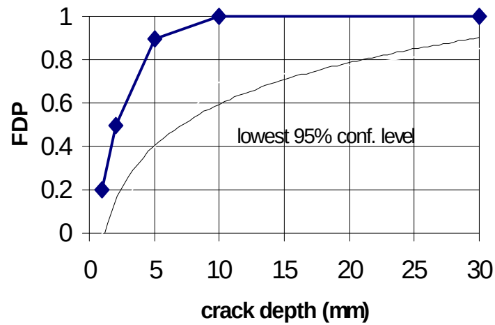
Figure 12.3: Surface crack detection performance vs. defect size in depth for ET used as surface inspection technique in ideal condition. Lowest 95% confidence level is the one of the less performant trial in the UCL project.
