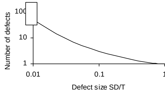
Figure 14.3: Approximate fabrication defect presence for 15m of weld in PISC assemblies (pressure vessels)
