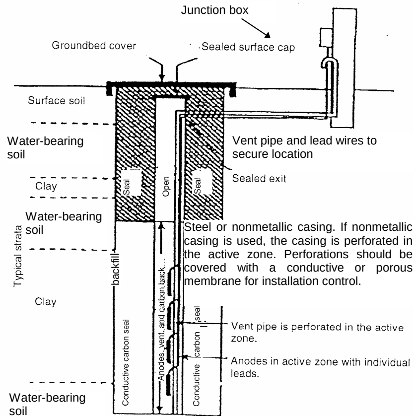
FIGURE A4: Environmentally Addressed System
