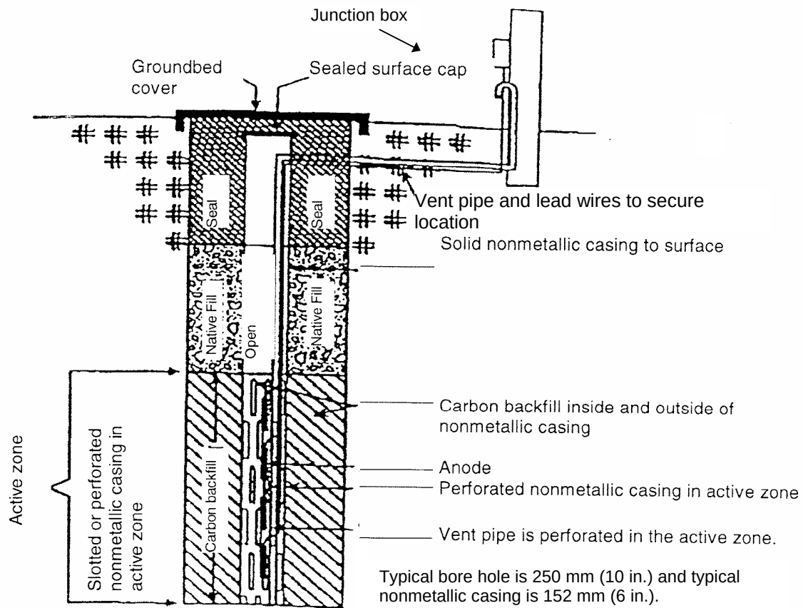
FIGURE A5: Typical Replaceable Closed Hole
