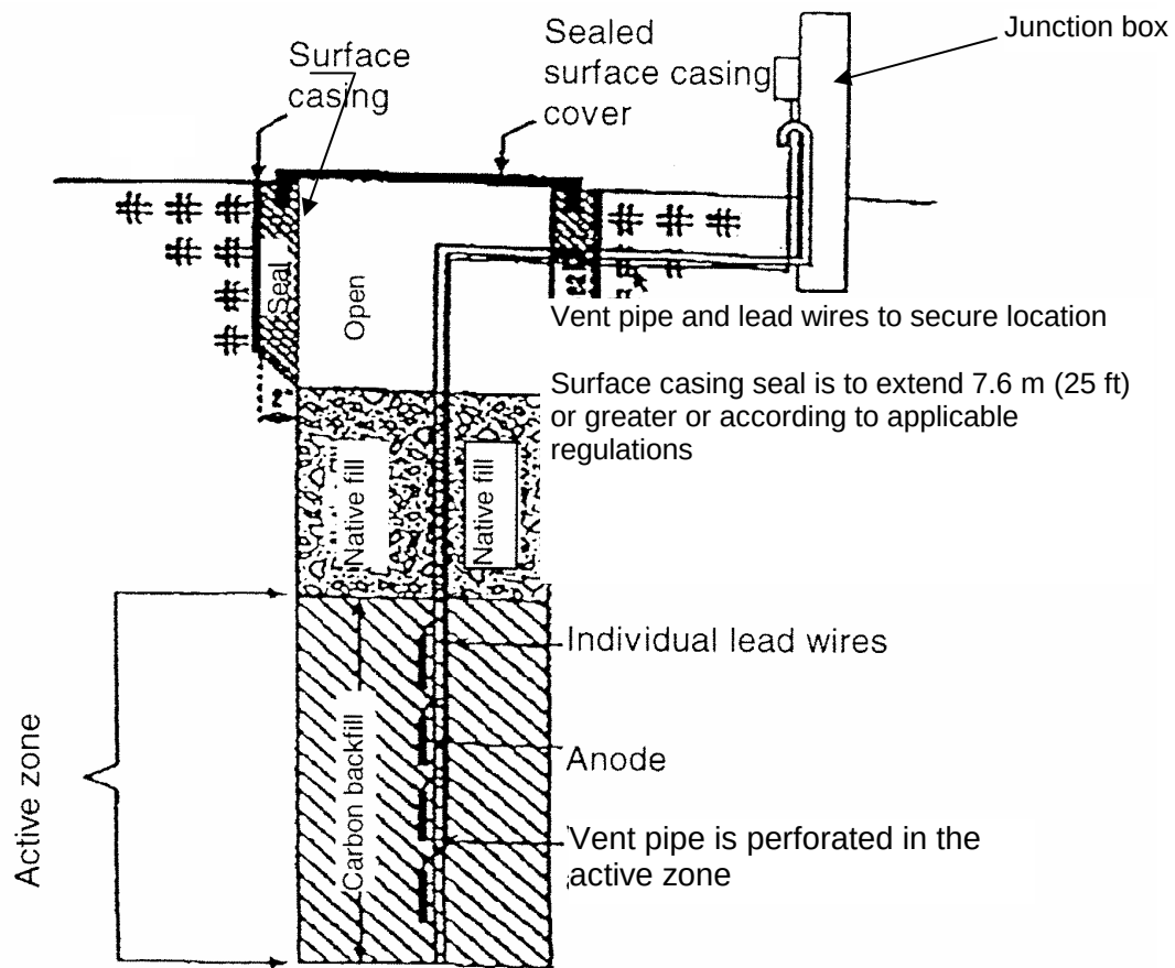
FIGURE A2: Closed Hole with Surface Casing
