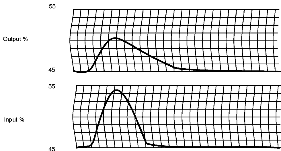
Figure 18 — Good test, pulse width satisfactory
