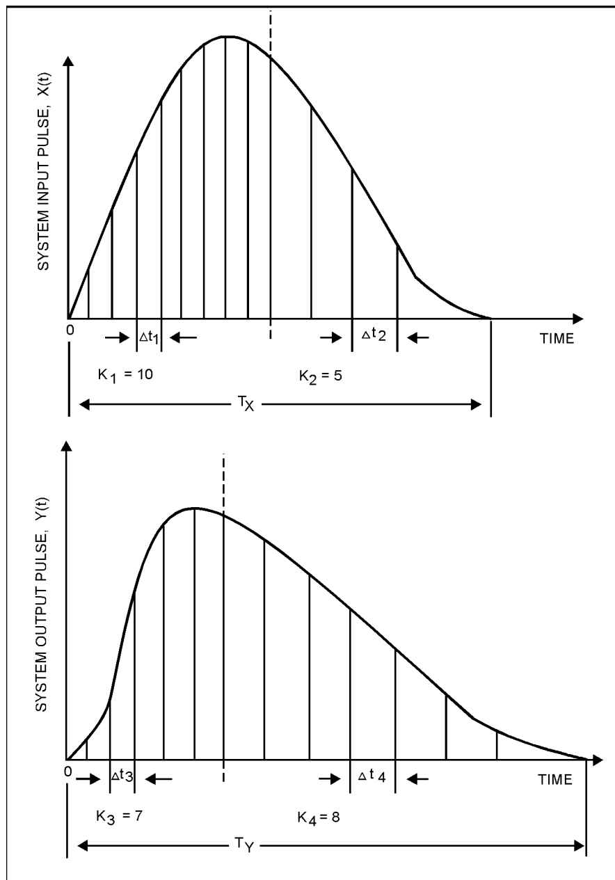
Figure 22 — Typical input and output pulses and their dissection.
