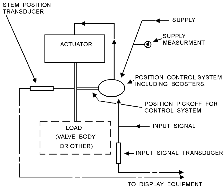
Figure 10 — Recommended loading test configuration
