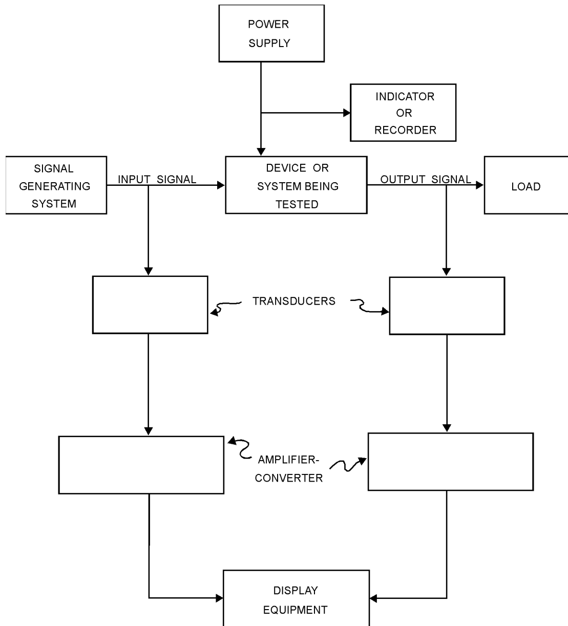
Figure 11 — Generalized dynamic test setup
