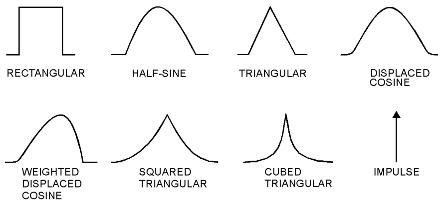
Figure 16 — Pulse input wave shapes
