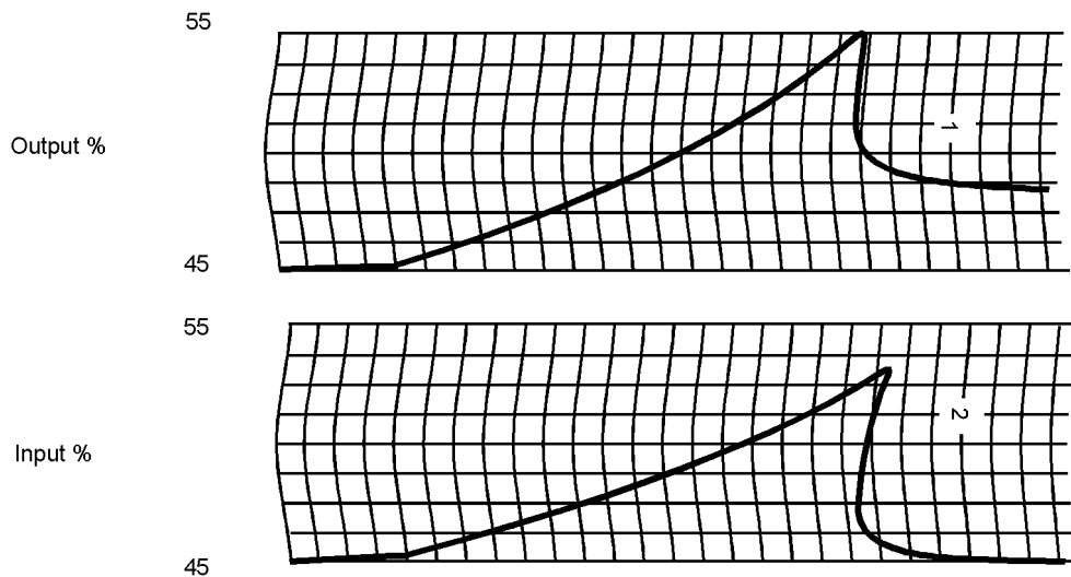
Figure 21 — Good ramp test for reset action
