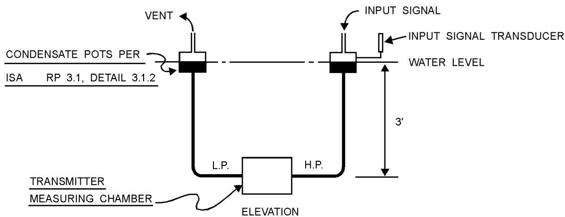
Figure 8 — Recommended wet test setup
