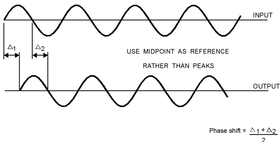
Figure 15 — Determination of phase shift
