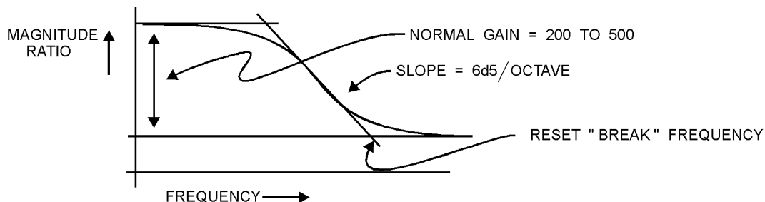
Figure 9 — Magnitude ratio response
