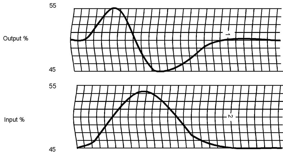
Figure 20 — Good pulse signal for rate characterization test
