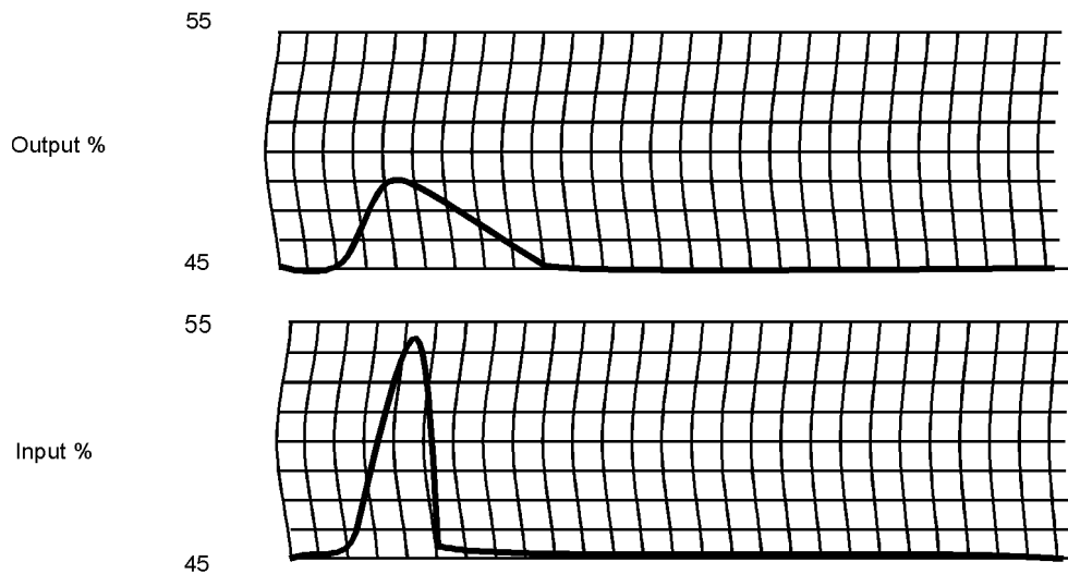
Figure 19 — Poor test, pulse width too narrow
