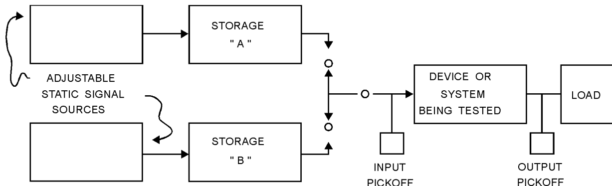
Figure 14 — Step signal generating circuit
