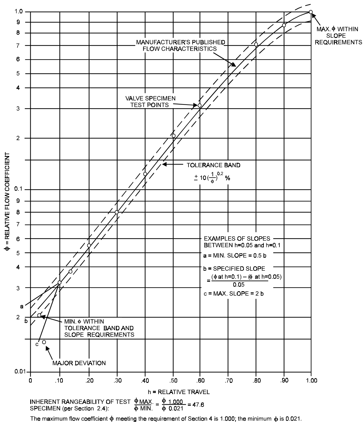
Figure 1 — Example of globe valve specimen compared to manufacturer-specified flow characteristic
