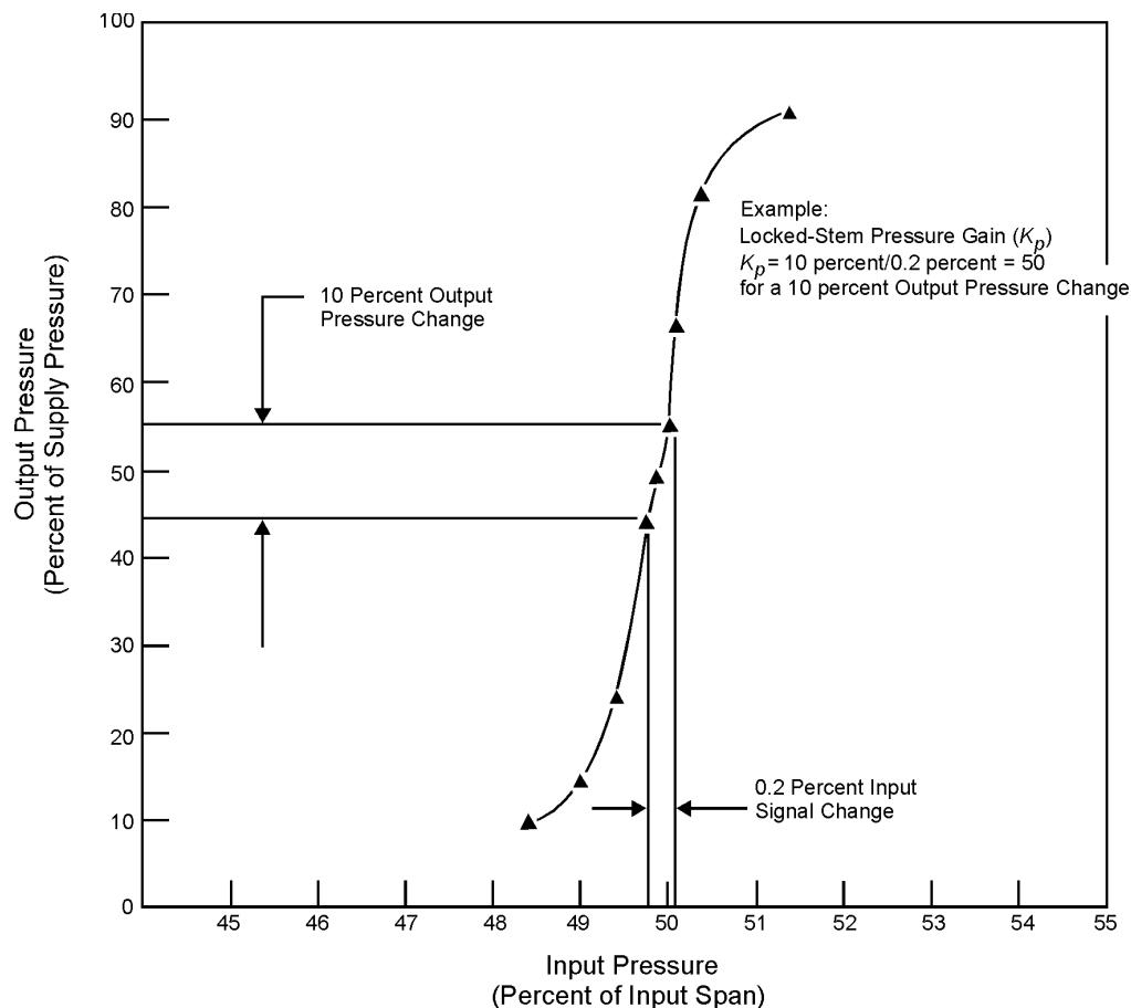
Figure 10 — Locked-stem pressure gain (single-acting)
