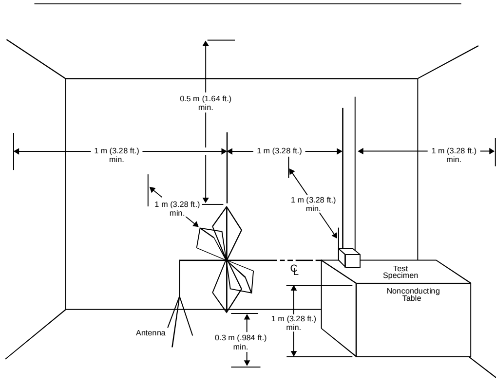
Figure 5 — Test arrangement for electromagnetic susceptibility
