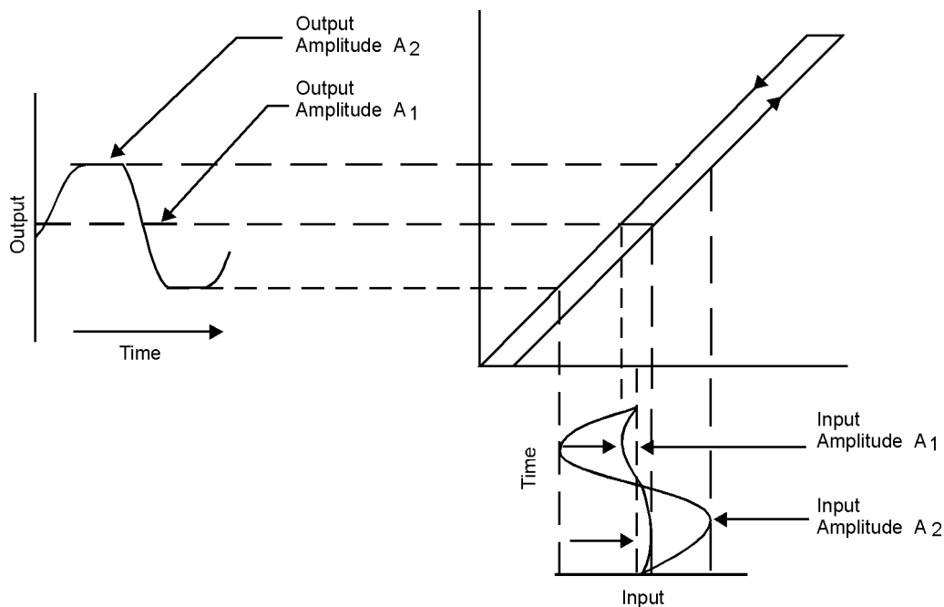
Figure 13 — Steady-state characteristic of element exhibiting dead band and effect on output
