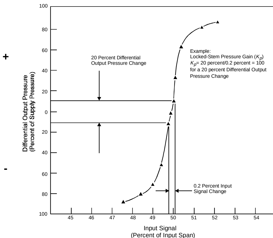
Figure 11 — Locked-stem pressure gain (double-acting)
