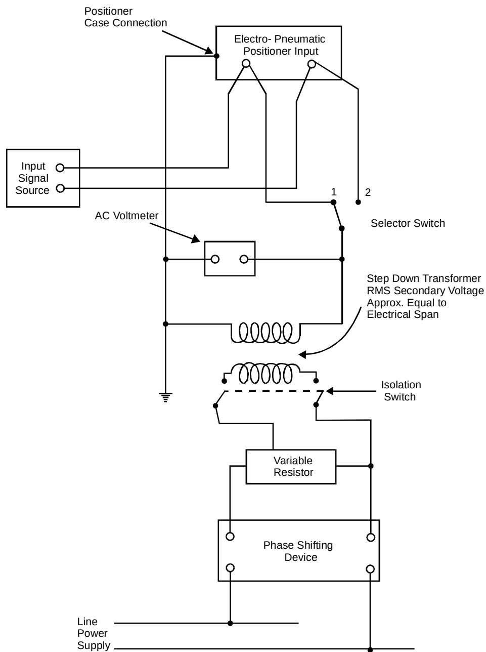
Figure 7 — Test circuit for common mode interference influence
