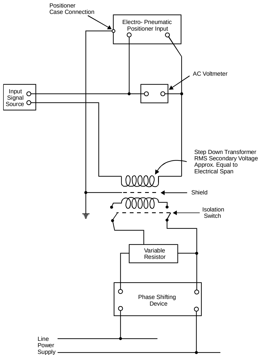
Figure 6 — Test circuit for normal mode interference influence
