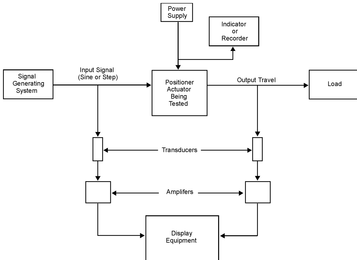
Figure 12 — Schematic of simple dynamic response test system
