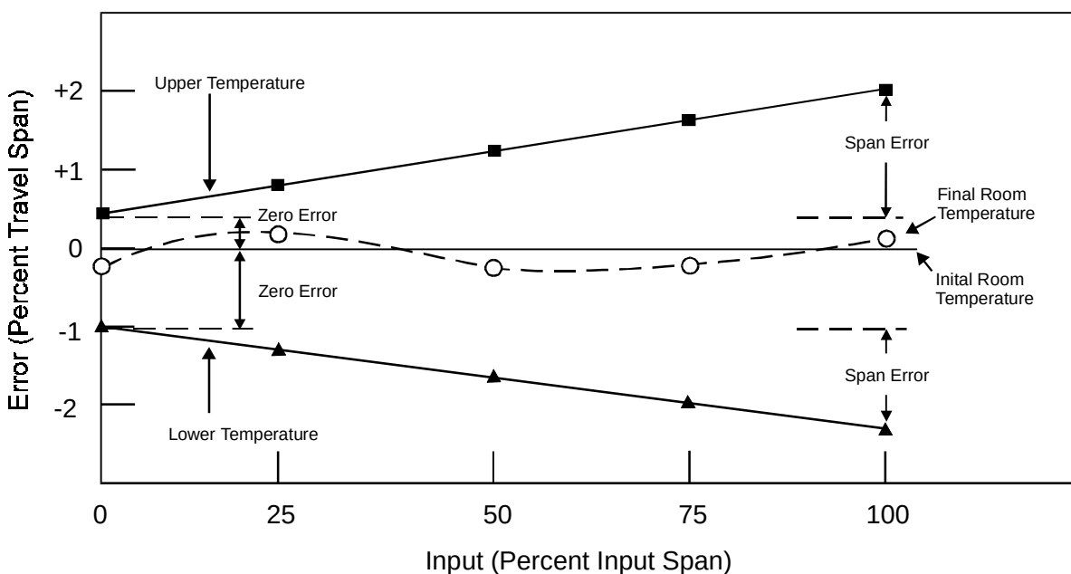
Figure 3 — Ambient temperature influence
