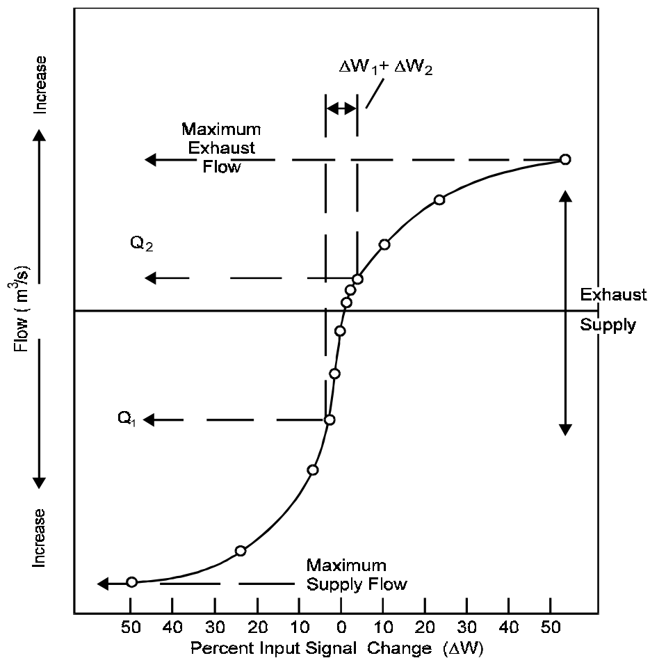
Figure 9 — Flow characteristic curve
