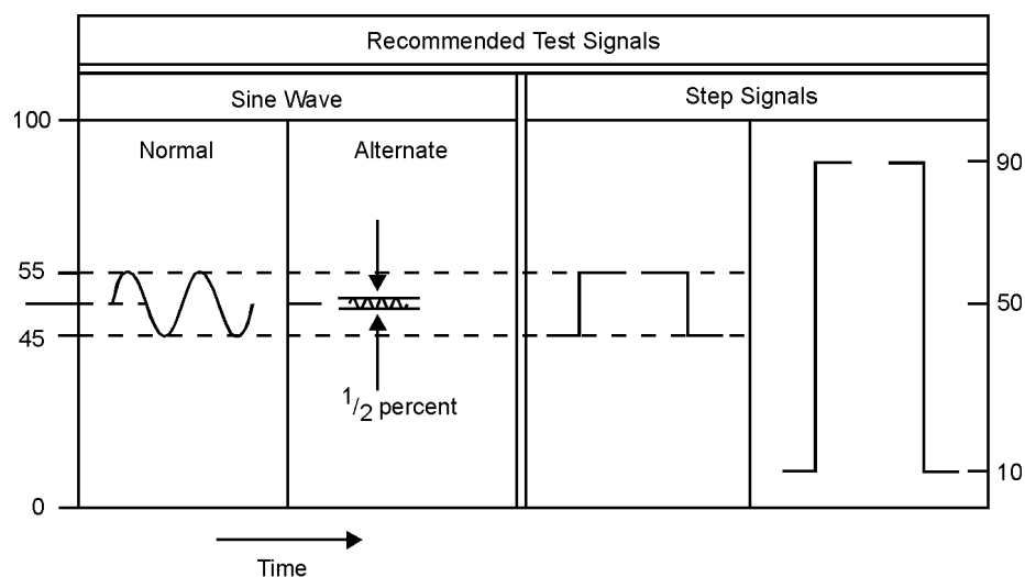
Figure 15 — Recommended test signals
