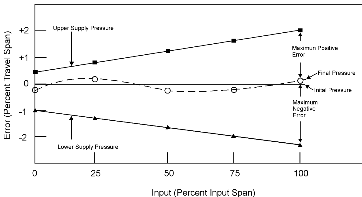
Figure 2 — Supply pressure influence
