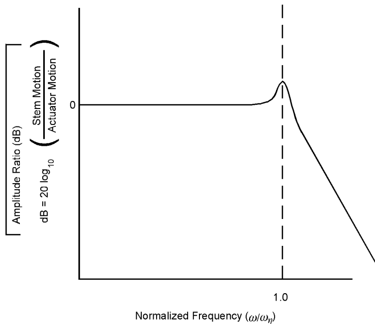
Figure 4 — Relative stem motion for typical linear actuator
