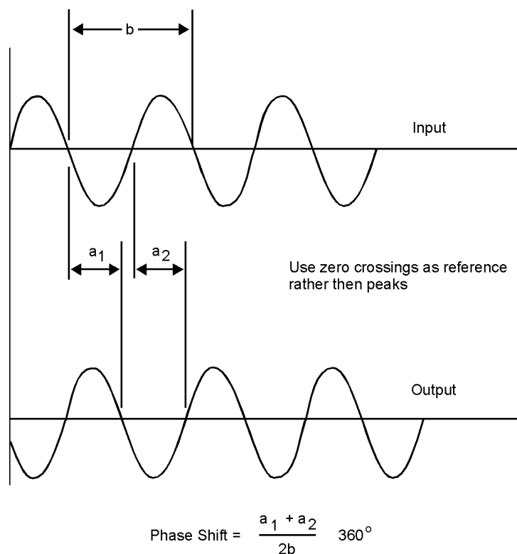
Figure 17 — Determination of phase shift for distorted output
