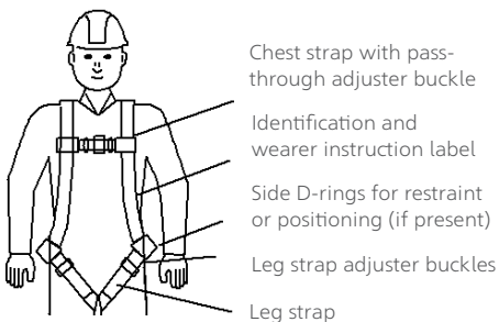
Figure D. Full-Body Harness (Front)
