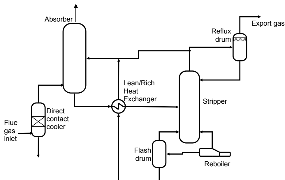
Figure 5.2 : Schematic diagram of Post-combustion capture process
