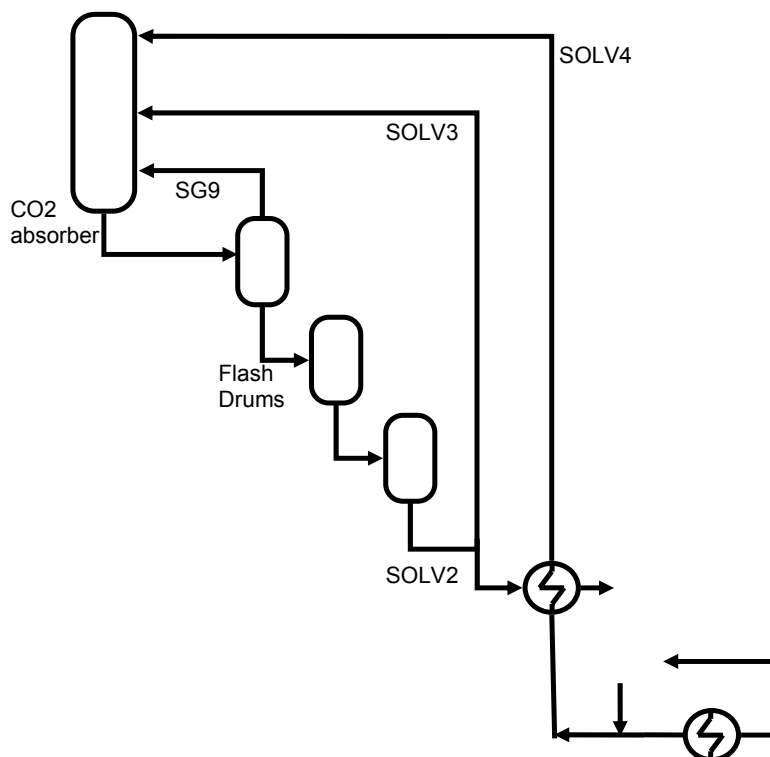
Figure 9.3 : Solvent loop, co-capture
