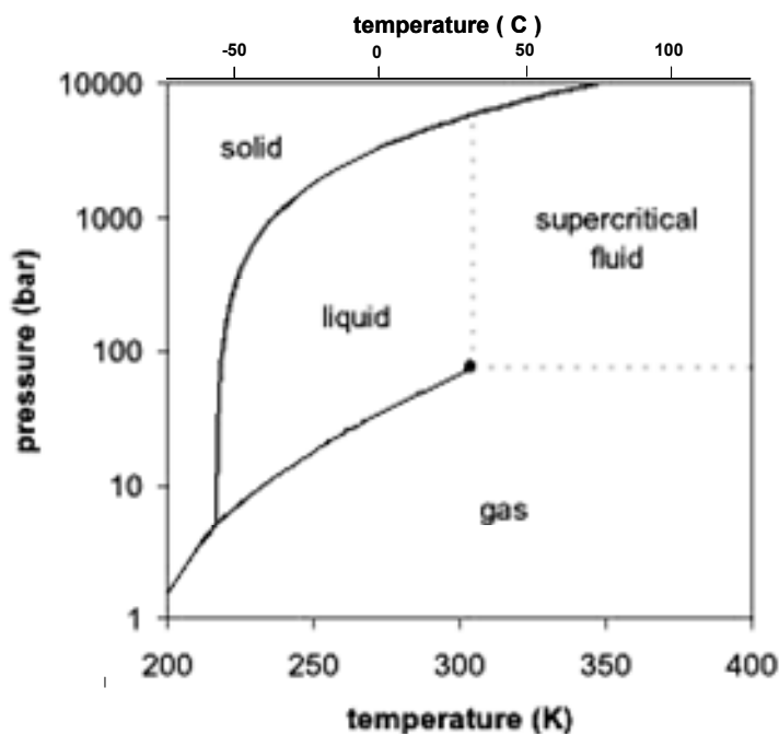
Figure 6.1 : CO 2 phase diagram
