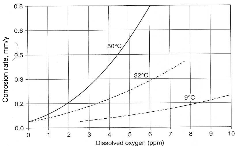
Figure 6.4 : Effect of oxygen concentration on the corrosion rate at different temperatures
