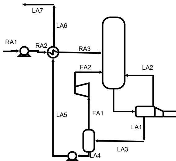
Figure 8.2 : Amine loop
