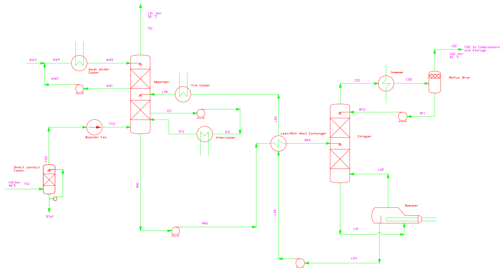
Figure 7: Post-combustion capture plant layout for flue gas from natural gas combustion
