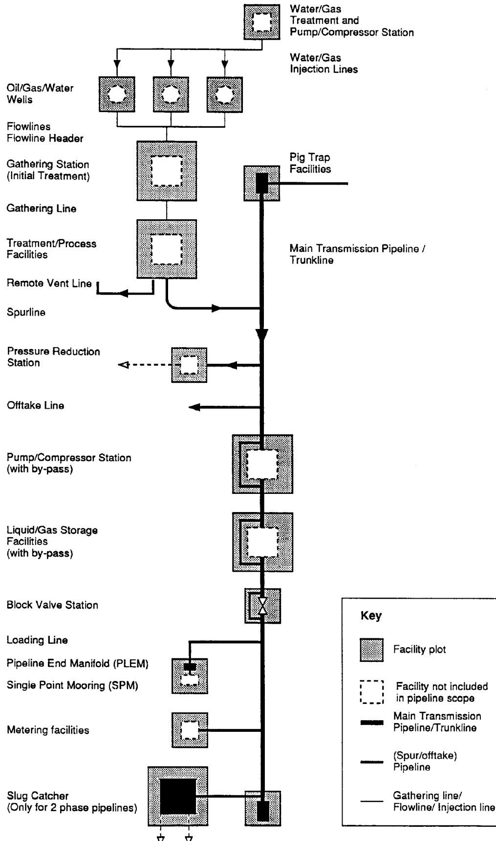
FIGURE 1 DIAGRAMMATIC REPRESENTATION OF PIPELINE SCOPE BOUNDARIES
