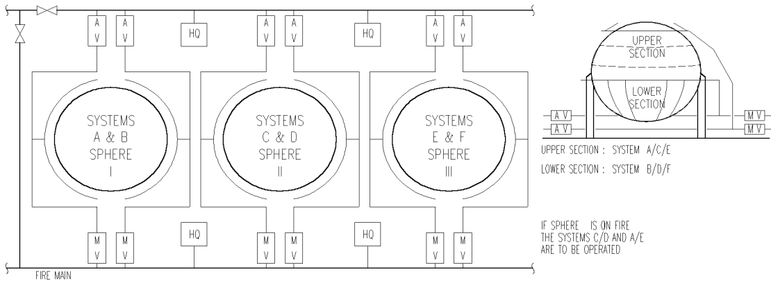
TYPICAL LPG STORAGE AREA SHOWING EXTENT AND CONNECTIONS OF WATER SPRAY SYSTEMS. EACH SYSTEM IS TO PROTECT HALF OF A SPHERICAL PRESSURE VESSEL.
