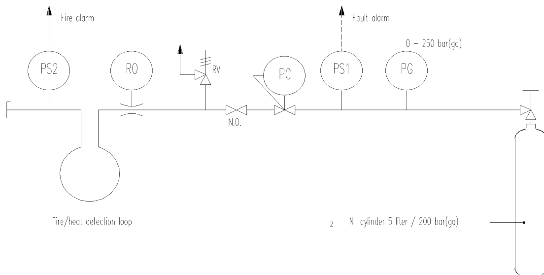
FLOW DIAGRAM
