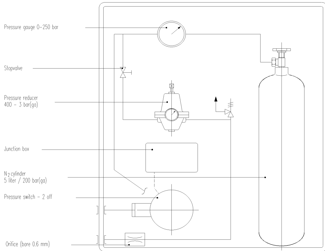
EQUIPMENT ARRANGEMENT
