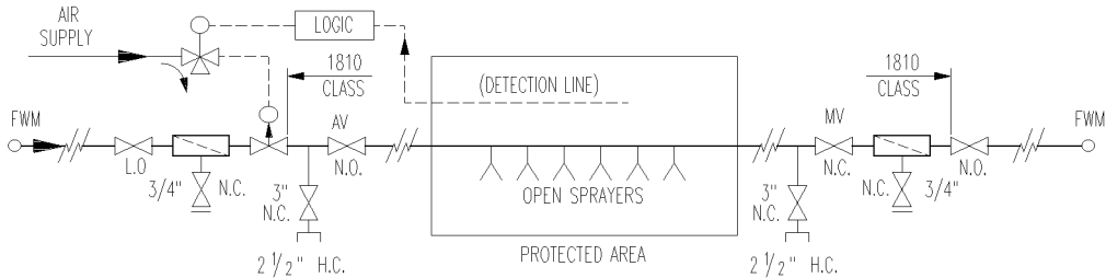
TYPICAL SCHEMATIC OF SPRAY SYSTEM (SEE ALSO APPENDICES 5 AND 6)
