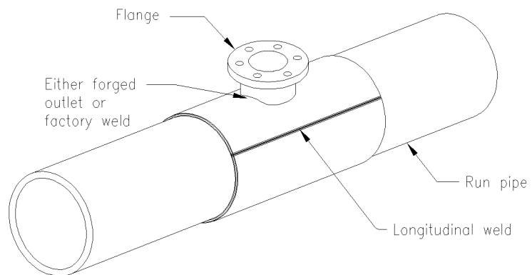
FIGURE 1 TYPES OF HOT-TAP CONNECTION
