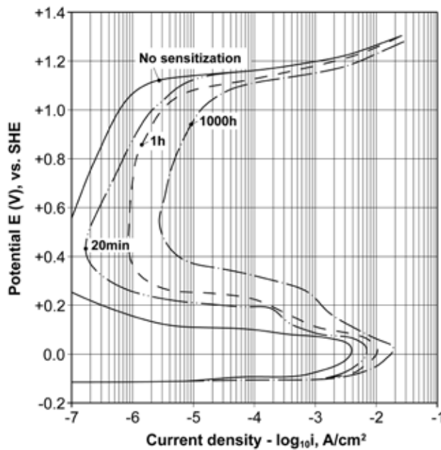
Figure 75 – Trend of the potentiodynamic curves of stainless steel type X5CrNi18-10 in its annealed status and after sensitisation at 650°C for various times; aqueous solution 1M of H_2SO_4 at 90°C [from Osozawa et al. 1966].
