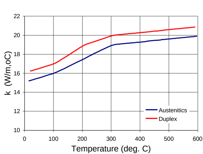
Figure 32 Thermal Conductivity for Austenitic and Duplex Stainless Steels.
