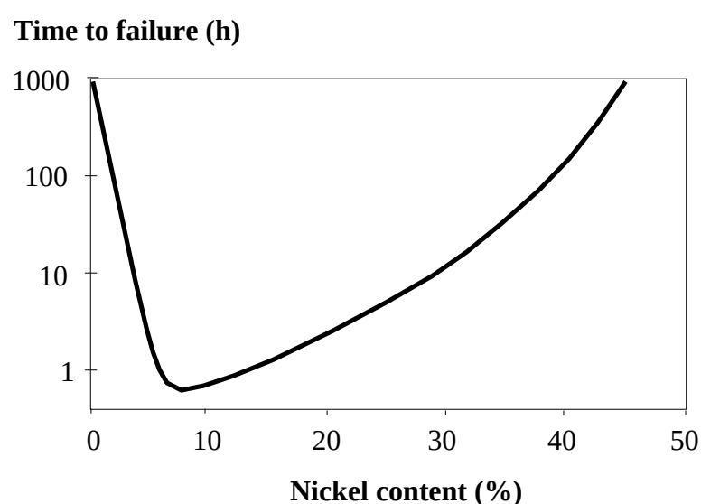
Figure 13. Stress corrosion cracking susceptibility in boiling \text{MgCl}_2 as a function of nickel content (4).
