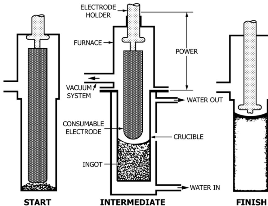
FIG. X1.1 Consumable Electrode Vacuum Melting Furnace
