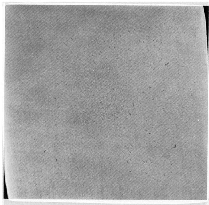
FIG. 14 Class 3—Radial Segregation—Severity D
