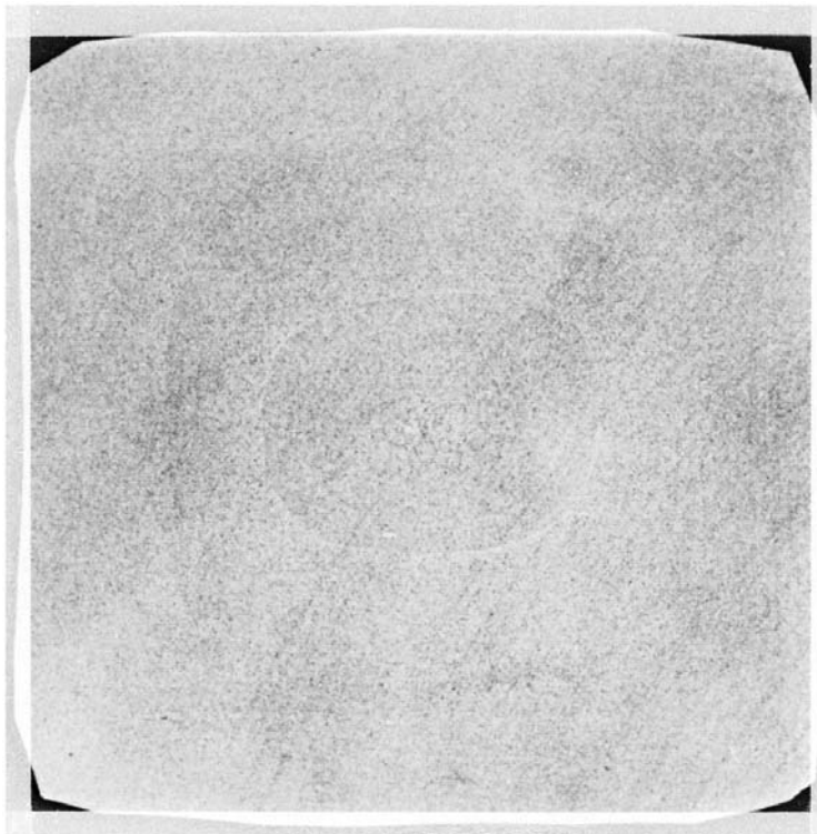
FIG. 16 Class 4—Ring Pattern—Severity A
