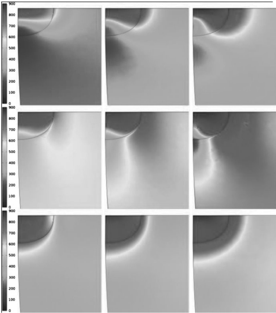
Figure 3-10 Distribution of stress on a steel pipe with a corrosion effect (top: no soil strain, middle: tensile soil strain, bottom: compressive soil strain. From left to right: operating pressures of 15, 20, and 25 MPa). (From Xu and Cheng [2012].)
