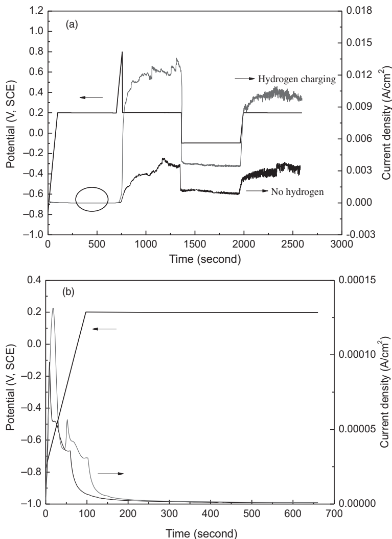
Figure 5-10 Potential–time and current density–time curves recorded in a potential step cycle in a concentrated carbonate–bicarbonate solution; (b) shows enlarged plots of the passive current densities shown in (a). (From Xue and Cheng [2010].)
