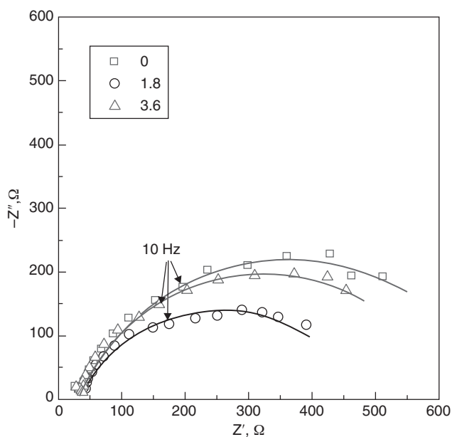
Figure 5-5 LEIS plots measured at three points across the various stressed areas marked in Fig. 5-4, where x = 0, 1.8 , and 3.6 mm, respectively, with a constant y = 1.35 mm in a concentrated carbonate–bicarbonate solution. (From Li and Cheng [2008].)
