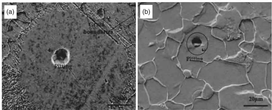
Figure 8-13 SEM views of the surface morphology of an X70 steel electrode after SVET measurement in Fig. 8-12 (a), and after etching in a 4 wt% HNO 3 -ethanol solution (b). (From Liu et al. [2010].)
