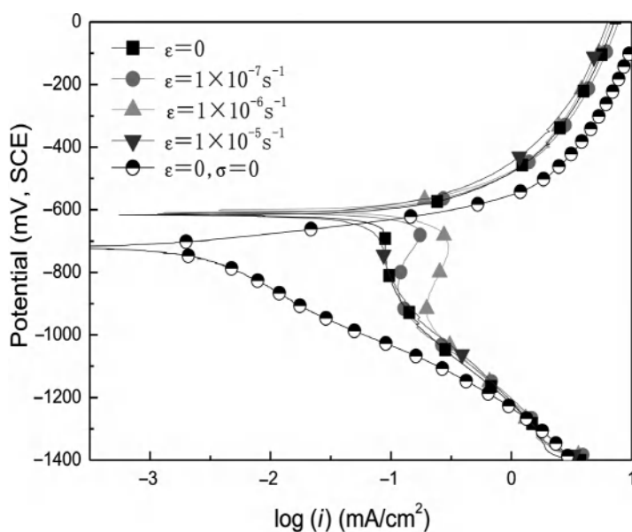
Figure 6-6 Potentiodynamic polarization curves measured on an X70 steel tensile specimen stressed at 0.5\sigma_{0.2} in a test solution. (From Liu et al. [2009b].)
