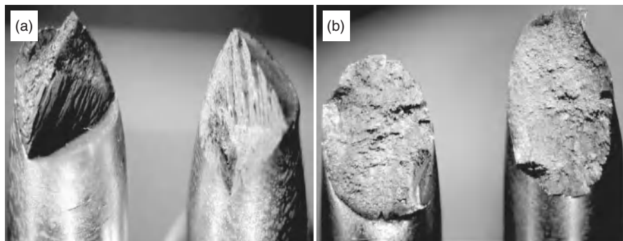
Figure 8-21 Fractographic views of (a) new X100 and (b) aged X100 steel specimens after an SSRT test at -0.85\text{ V}(\text{Cu}/\text{CuSO}_4) in a nearly neutral-pH solution. (From Sanjuan Riverol [2008].)
