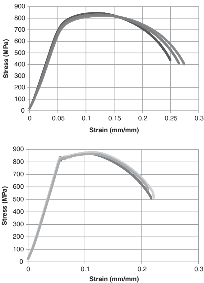
Figure 8-18 Stress–strain curves of (a) a new X100 steel and (b) an aged X100 steel specimen. (From Sanjuan Riverol [2008].)
