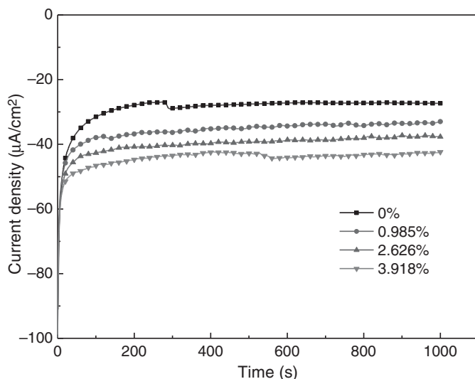
Figure 8-26 Current densities measured on an X100 steel specimen that is polarized at -1 V(SCE) under various prestrains in a nearly neutral-pH solution. (From Xu and Cheng [2012b].)
