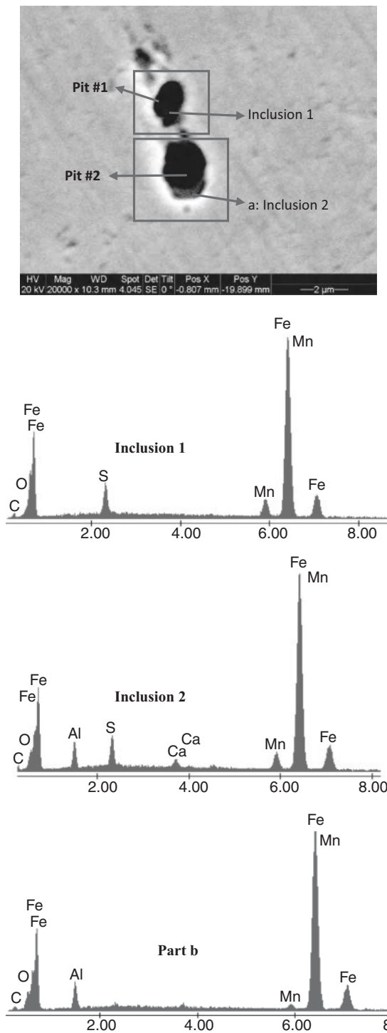
Figure 8-14 SEM image of corrosion pits initiated at an MnS inclusion (pit 1) and an MnS/Al 2 O 3 inclusion (pit 2) as well as relevant EDX spectra. (From Jin [2011].)
