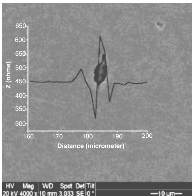
Figure 8-10 LEIS linear scanning map measured on an X100 steel substrate and around the inclusion in a nearly neutral-pH bicarbonate solution. (From Jin and Cheng [2011].)
