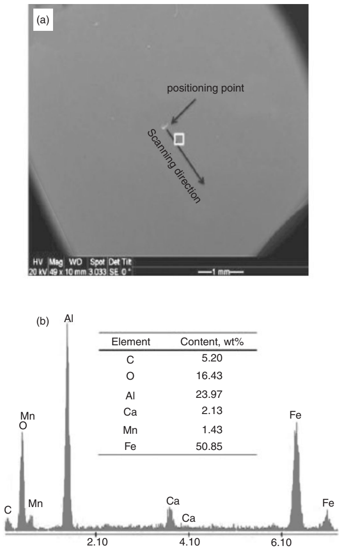
Figure 8-9 LEIS scan line on an X100 steel electrode surface (a) and the EDX spectrum (b) obtained on the defect as marked by a square in (a). (From Jin and Cheng [2011].)
