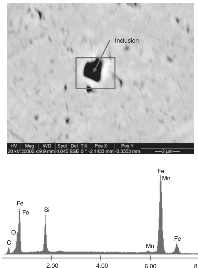
Figure 8-16 SEM view of a corrosion pit associated with a silicon-enriched inclusion as determined by an EDX spectrum. (from Jin [2011].)
