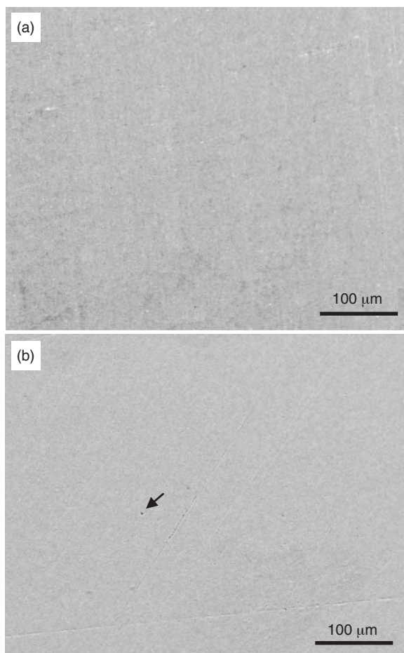
Figure 4-14 Surface morphologies of an X70 steel electrode after 144 h of potentiostatic polarization at (a) -950 \text{ mV(SCE)} and (b) -850 \text{ mV(SCE)} in an NS4 solution. (From Liu et al. [2012].)
