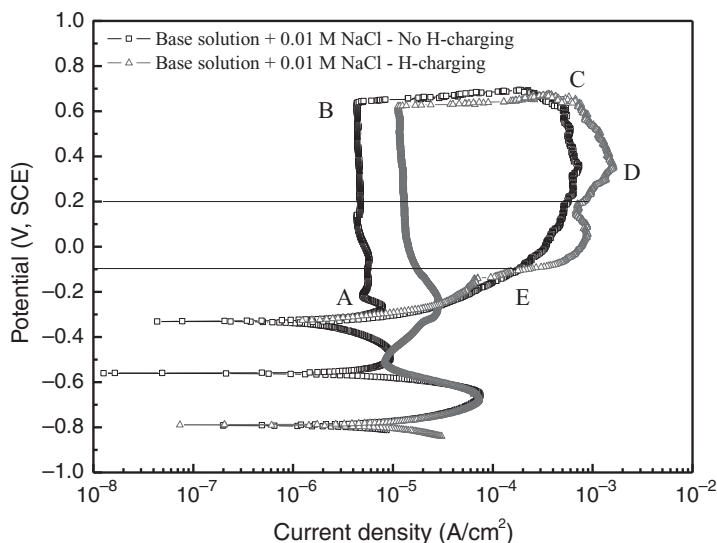
Figure 5-8 Cyclic polarization curves measured on uncharged and precharged X80 steel electrodes in a carbonate–bicarbonate solution containing 0.01 M NaCl. (From Xue and Cheng [2010].)
