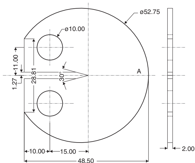
Figure 5-11 Schematic diagram of a precracked X70 steel compact tension specimen (unit: mm). (From Zhang and Cheng [2010].)
