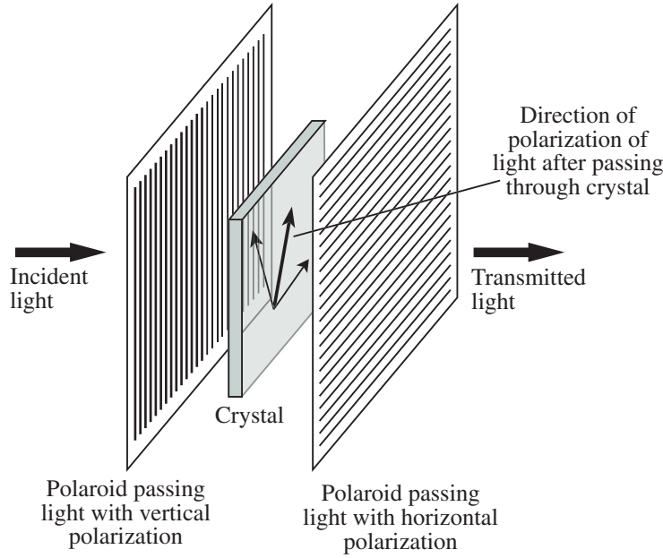
Fig. 1.3 Simple experiment in which a crystal is held between two polaroids oriented at 90^\circ with respect to each other. The first polaroid transmits only the component of the light with polarization in the vertical direction. If none of the special axes of the crystal are aligned parallel to the polarization of the light, the crystal will effectively rotate the direction of the polarization of the transmitted light, allowing some intensity to pass through the second polaroid, which only transmits the component of horizontal polarization.
