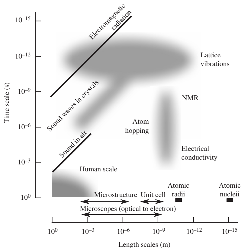
Fig. 1.13 Important length scales and time scales in the study of crystals.
