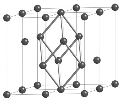
Fig. D.1 One mapping of a primitive rhombohedral unit cell onto non-primitive trigonal axes.
