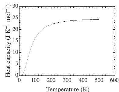
Fig. 1.9 Variation of the heat capacity of NaCl with temperature, in terms of per mole of atoms. The classical theory outlined in the text would predict a value of 3R = 24.9 \text{ J mol}^{-1} \text{ K}^{-1} , to which the heat capacity tends at high temperatures. The effect of temperature on the heat capacity is discussed in Chapter 9.
