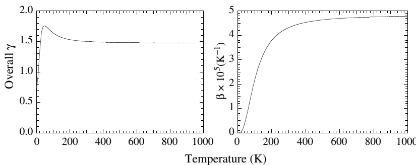
Fig. 11.6 Temperature dependence of the overall Grüneisen parameter (left) and coefficient of volume thermal expansion (right) for fluorite, \text{CaF}_2 , calculated using a simple model set of interatomic interactions (Chapter 5).
