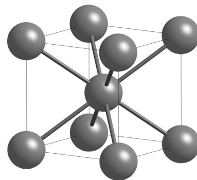
Fig. 2.10 Body-centred cubic structure. Each atom has eight neighbours, as indicated by the bonds drawn between atoms.
