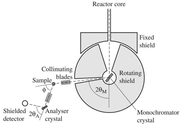
Fig. 10.2 Schematic representation of the triple axis spectrometer. The angles 2\theta_M , \phi and 2\theta_A can all be adjusted in routine operation.
