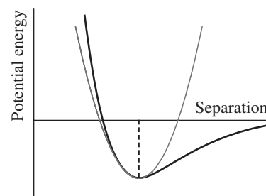
Fig. 1.7 Dependence of potential energy on the separation between a cation and anion (dark curve), compared with a symmetric potential (light curve). The steep rise at low separations arises from the repulsive interaction which prevents the ions from becoming too close. The slow tail at large separations is the residual attractive interaction. The two curves overlap around the minimum in the potential energy, denoted by the dashed line. The form of this plot will be explored in Chapter 5.
