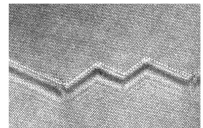
Fig. A.8 Unusual zig-zag shaped line defect in gold observed by electron microscopy. (Picture courtesy of A. Kirkland and P. Middledy, University of Cambridge.)
