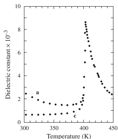
Fig. 2.31 Dielectric constant of BaTiO 3 in the vicinity of the cubic–tetragonal ferroelectric phase transition. In the ferroelectric phase there are differences along the a and c axes.
