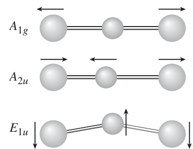
Fig. 10.7 The three normal modes of the \text{CO}_2 molecule.
