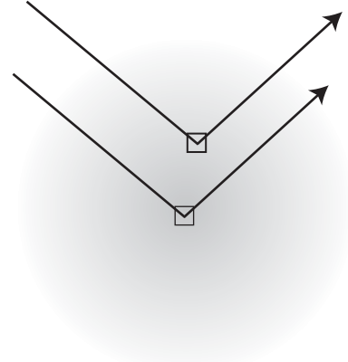
Fig. 6.13 Two rays of a radiation beam scattered from volume elements in a continuous distribution of particles, in this case shown as a representation of the distribution of electrons in an atom.
