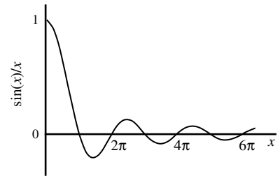
Fig. B.1 Sinc function as the Fourier transform of the slit function.
