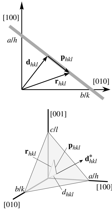
Fig. 4.4 A crystal plane ( hkl ) viewed edge-on. \mathbf{r}_{hkl} is a vector to a point in the plane. This vector is decomposed into the sum of \mathbf{d}_{hkl} , a vector from the origin to the plane and normal to the plane, and \mathbf{p}_{hkl} , a vector lying in the plane. As demonstrated in the text, the ( hkl ) plane intersects the \mathbf{a} , \mathbf{b} axes at the points a/h and b/k respectively.
