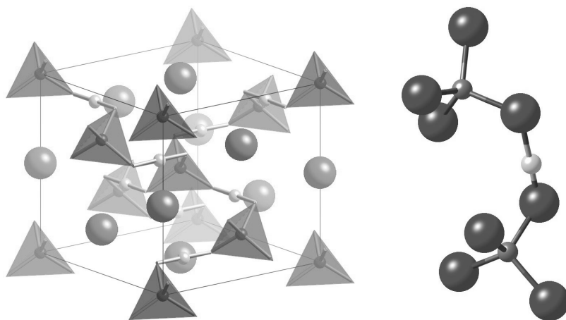
Fig. 5.7 Crystal structure of \text{KH}_2\text{PO}_4 with disordered hydrogen bond. In the left-hand plot, the \text{PO}_4 tetrahedra are shown as shaded units, the large spheres represent the K cations, and the small spheres represent the hydrogen atoms. In the right-hand plot, which focuses on a single hydrogen bond, the large atoms are the oxygen atoms, the P atoms are those bonded to four oxygen atoms, and the hydrogen atom lies between two oxygen atoms closer to one atom than the other.
