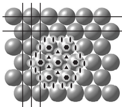
Fig. 2.3 Another view of the close-packed layer, showing some of the axes of the rotational symmetry (hexagons for 6-fold rotational symmetry, triangles for 3-fold symmetry, and ellipses for 2-fold symmetry), and the lines of the mirror planes.
