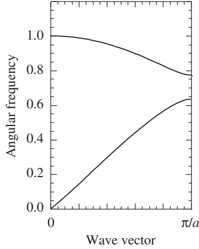
Fig. 8.14 Dispersion curves for the one-dimensional diatomic chain obtained from eqn 8.49.
