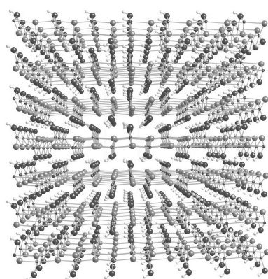
Fig. 4.1 View of the crystal structure of \text{Cu(OH)}_2 . Even in a structure this complicated, several planes of atoms with different orientations can clearly be seen.
