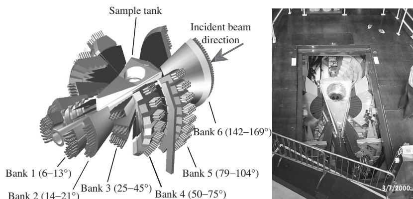
Fig. 6.10 State-of-the art neutron powder diffractometer at the ISIS spallation neutron source. (Photograph and diagram by courtesy of the ISIS Facility.)
