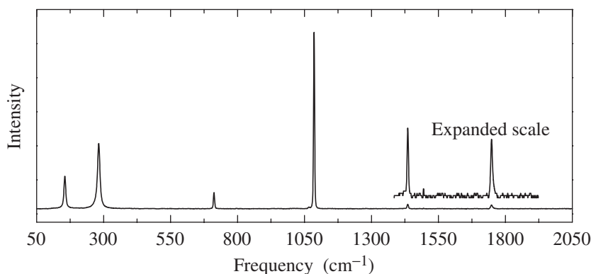
Fig. 10.8 The Raman scattering spectrum of calcite at room temperature, which can be compared with the infrared closeup absorption spectrum shown in Fig. 1.10 (data courtesy of Ming Zhang, University of Cambridge).
