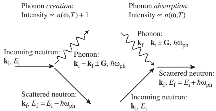
Fig. 10.1 Representation of the two types of one-phonon scattering process, drawn here for neutron scattering, but the same diagrams are also applicable to photon scattering (X-ray or light).
