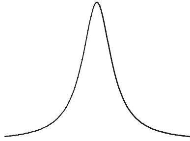
Fig. B.2 Representation of the Lorentzian function.
