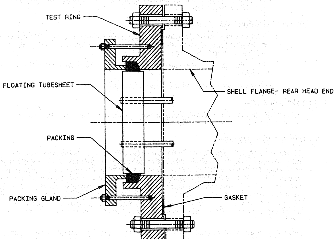
FIGURE E-4.13-2
