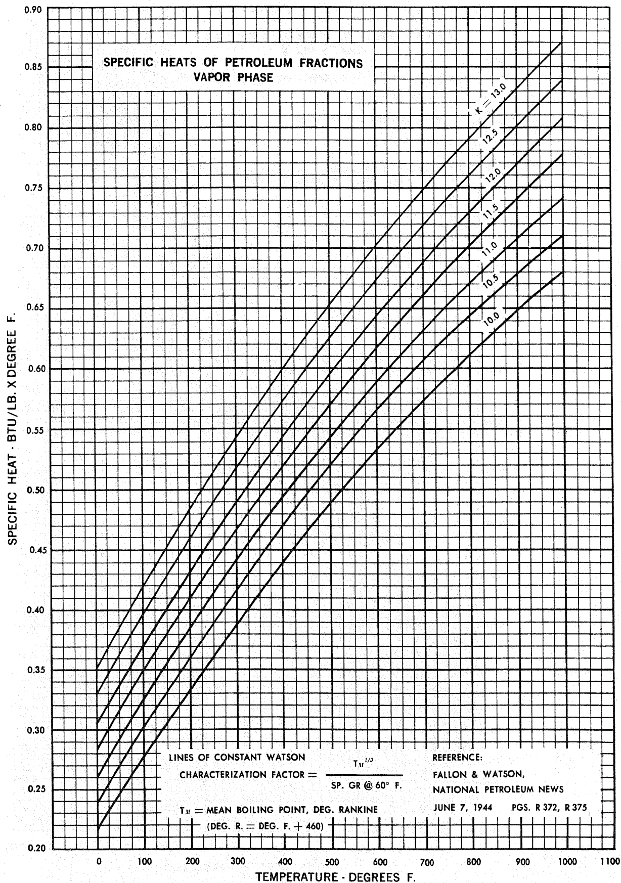
FIGURE P-2.2
