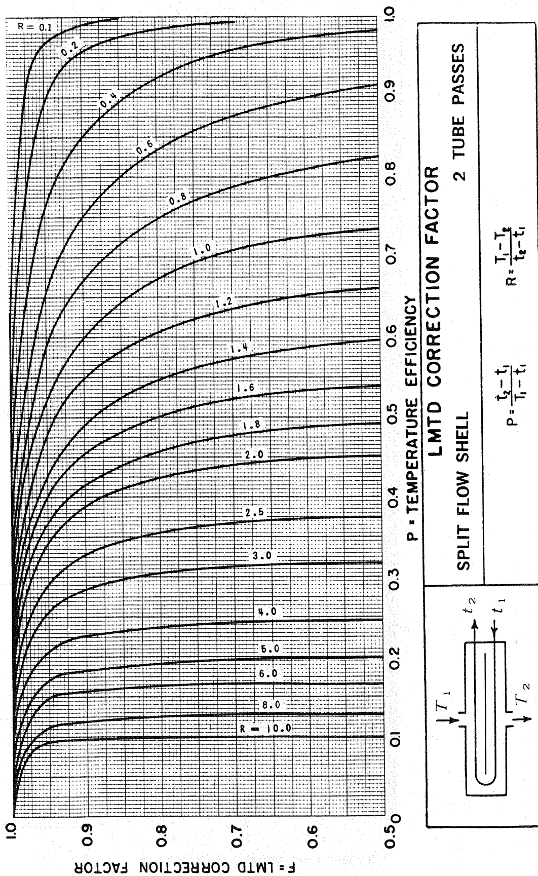
FIGURE T-3.2K
