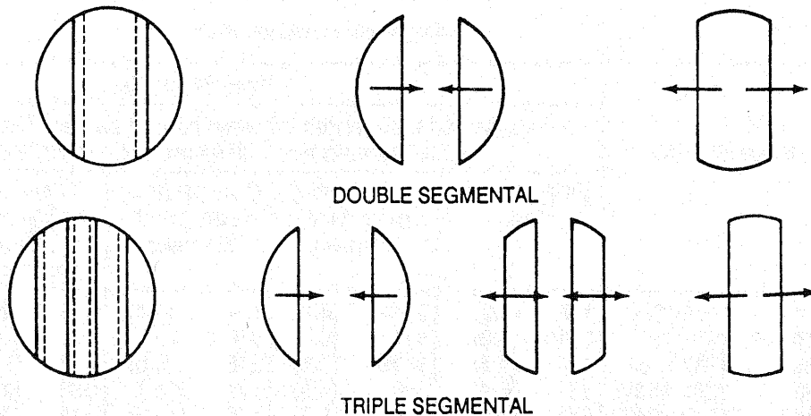
BAFFLE CUTS FOR MULTI-SEGMENTAL BAFFLES
