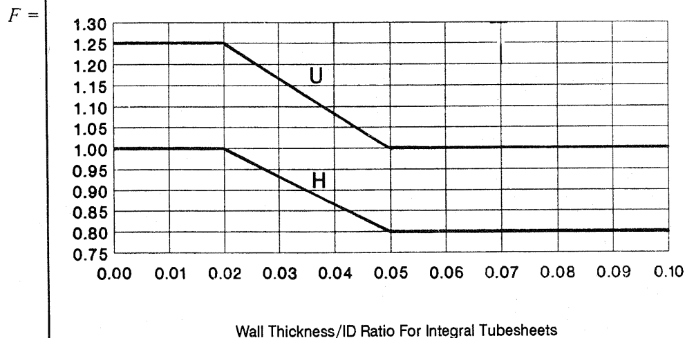
FIGURE RCB-7.132
