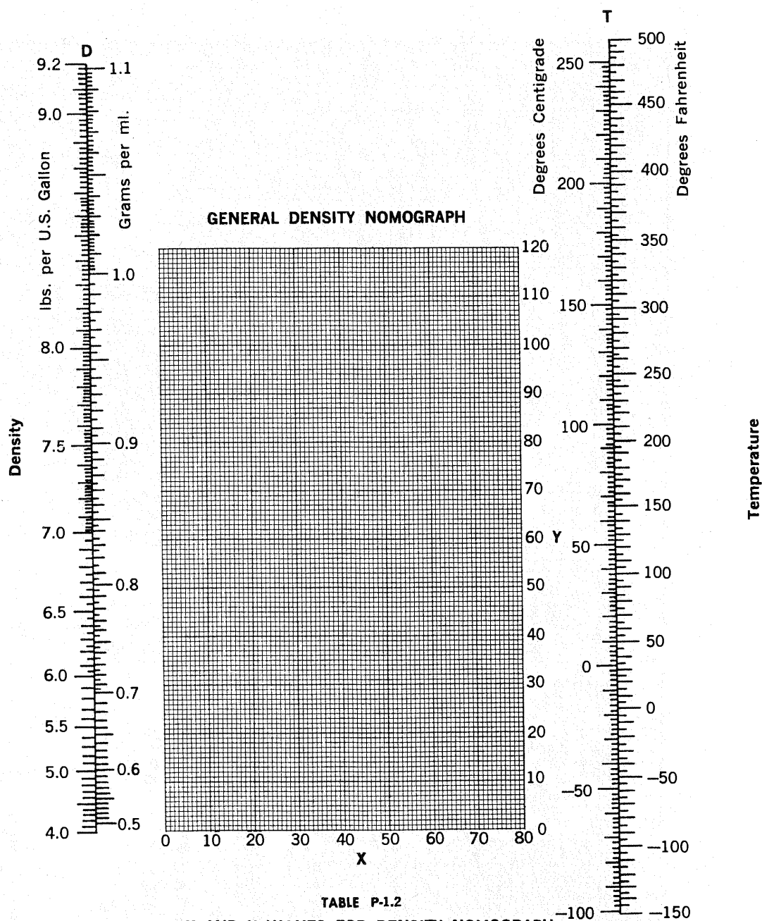
FIGURE P-1.2
