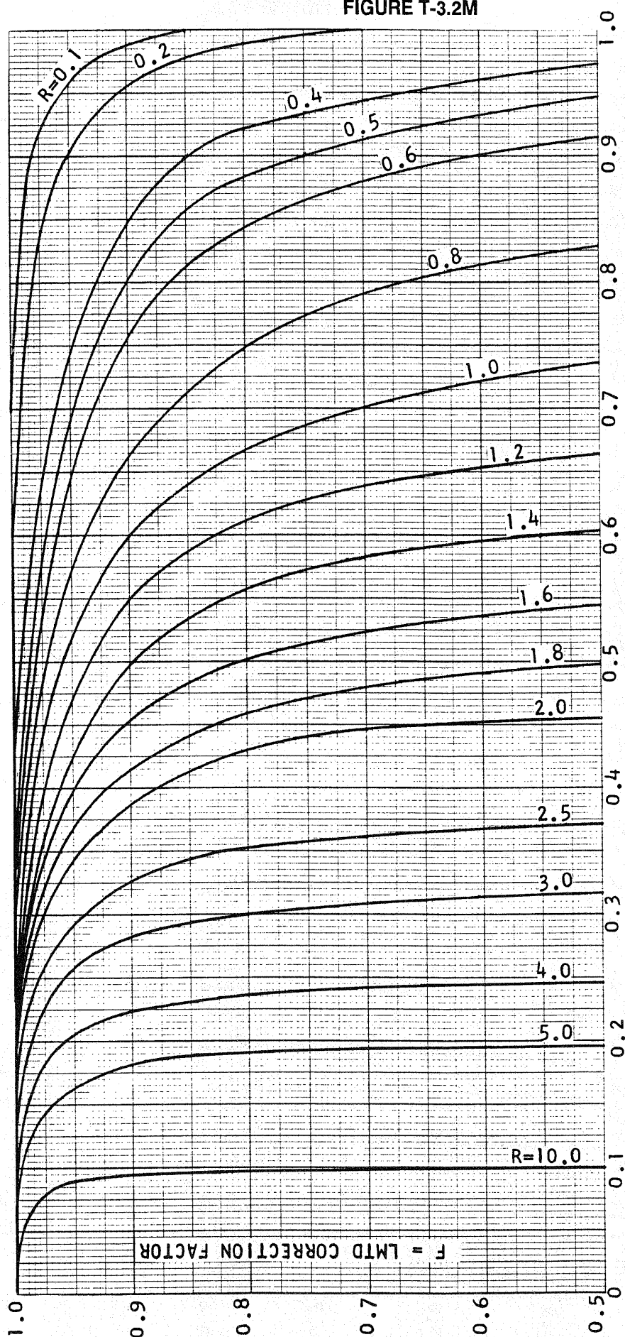
FIGURE T-3.2M
