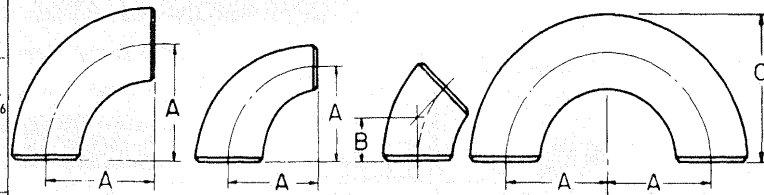
Long Radius Weld Ells
