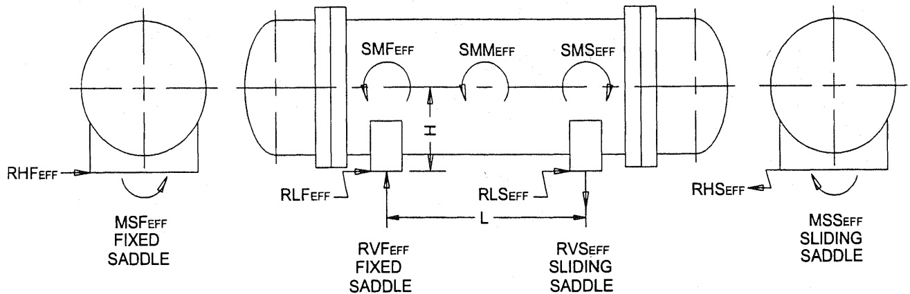
FIGURE RGP-G-7.1115
