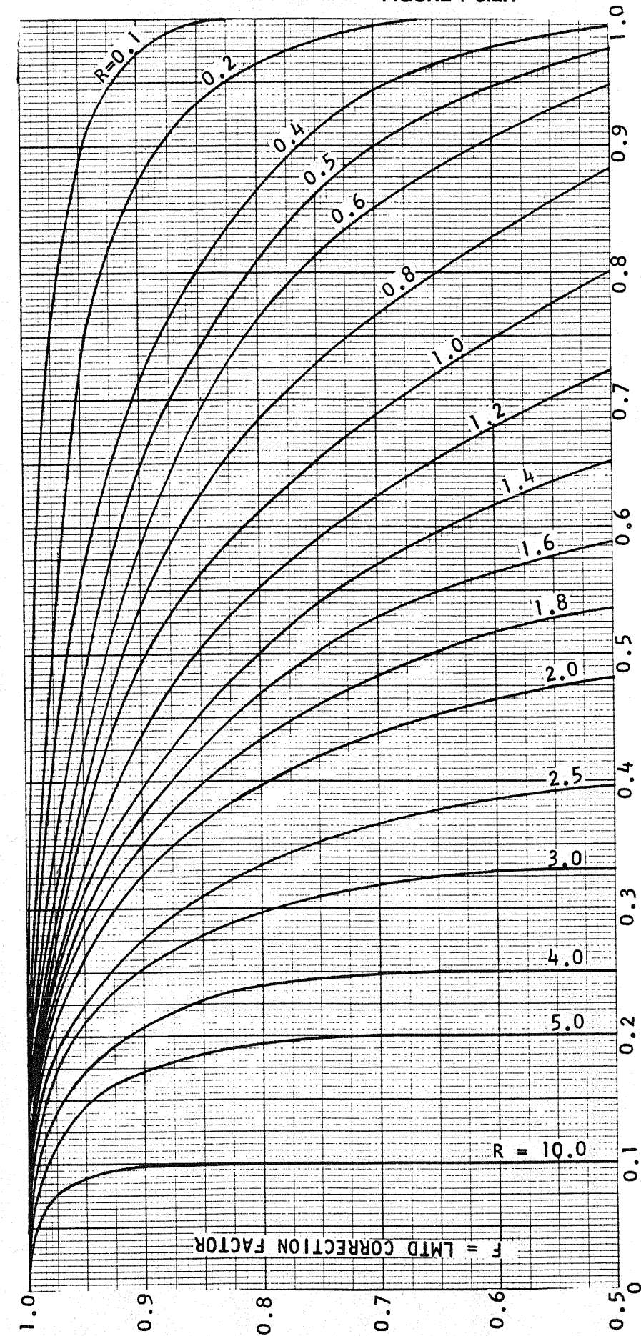
FIGURE T-3.2H
