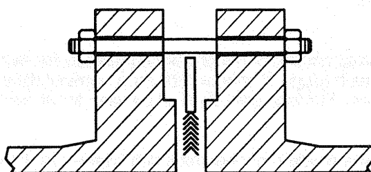
Confined Gasket
