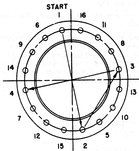
FIGURE E-3.25
