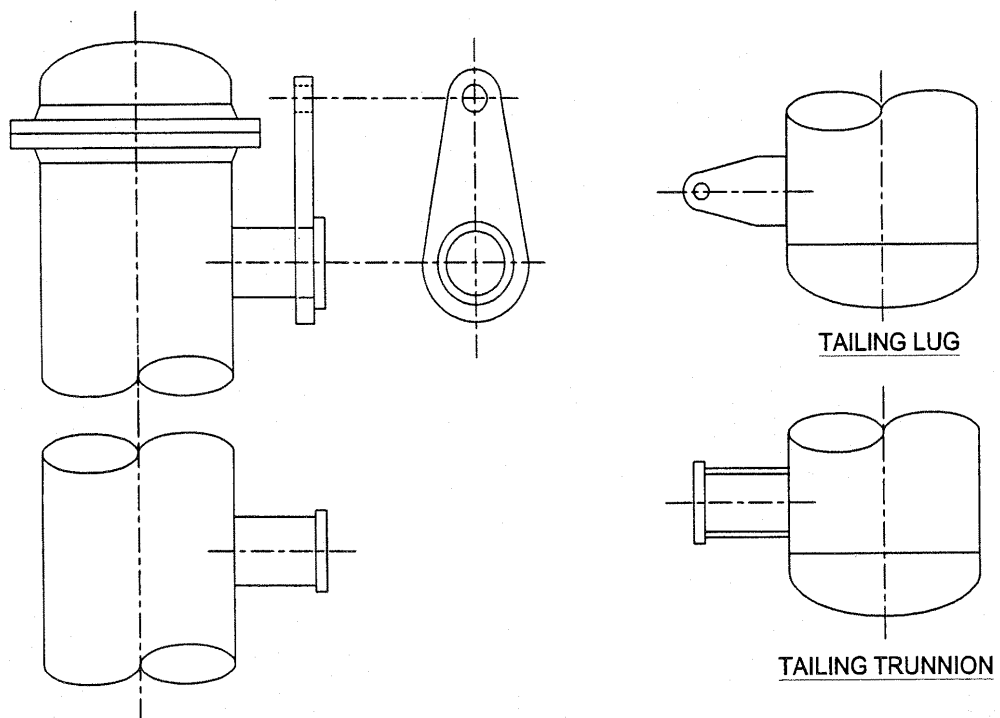
TRUNNION
