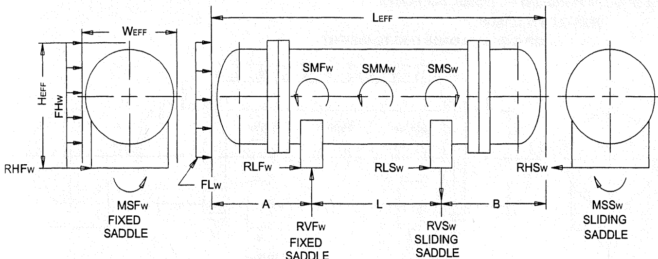
FIGURE RGP-G-7.1113
