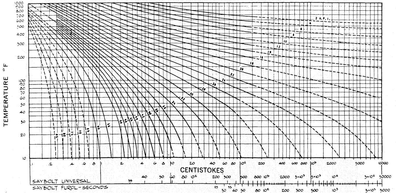
FIGURE P-5.2D
