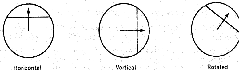
FIGURE RCB-4.1 BAFFLE CUTS FOR SEGMENTAL BAFFLES
