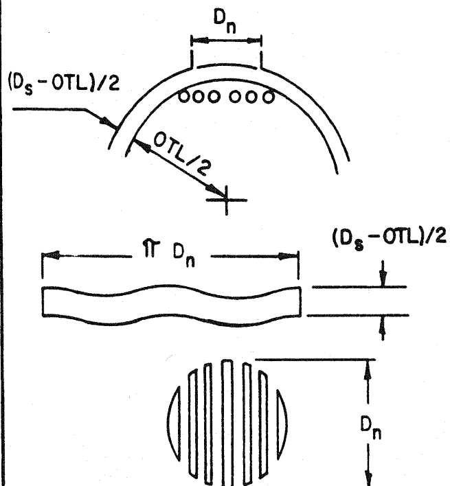
FIGURE RGP-RCB-4.6221 NO IMPINGEMENT PLATE - FULL LAYOUT
