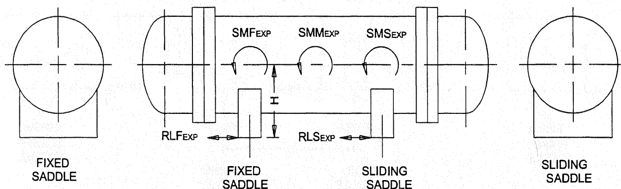
FIGURE RGP-G-7.1114
