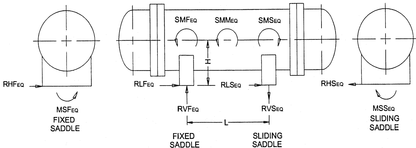
FIGURE RGP-G-7.1112
