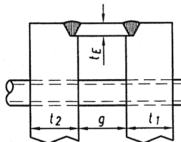
FIGURE RCB-7.155
