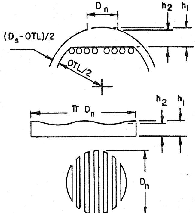
FIGURE RGP-RCB-4.6222 NO IMPINGEMENT PLATE - PARTIAL LAYOUT
