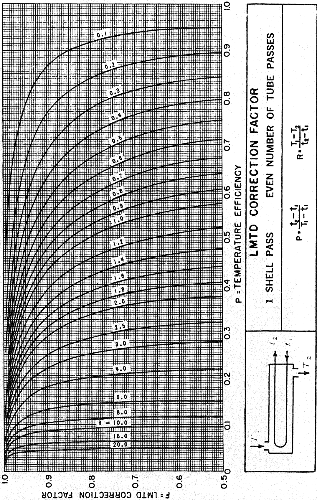
FIGURE T-3.2A
