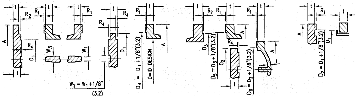
STANDARD CONFINED JOINT CONSTRUCTION
