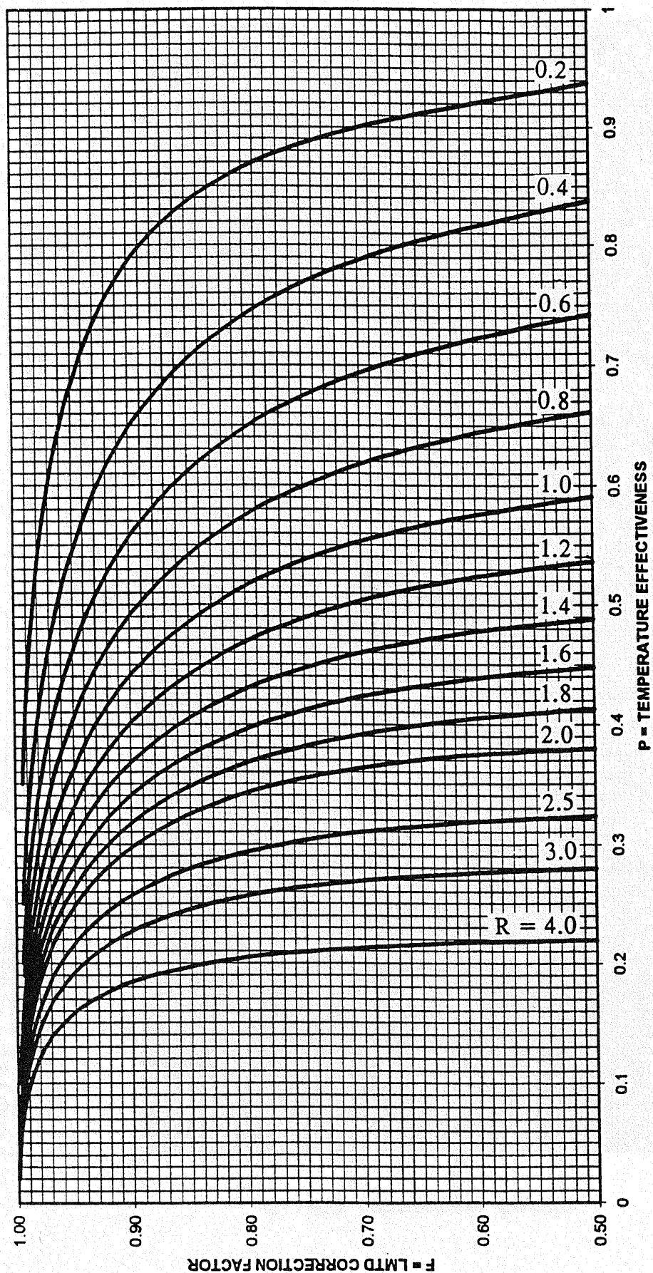
FIGURE T-3.2G
