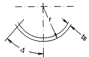
EFFECTIVE SECTION MODULUS OF ARC
