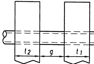
FIGURE RCB-7.156
