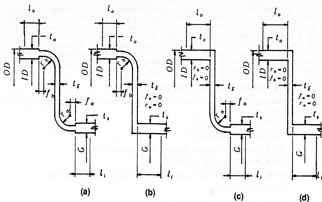
FIGURE RCB-8.21
