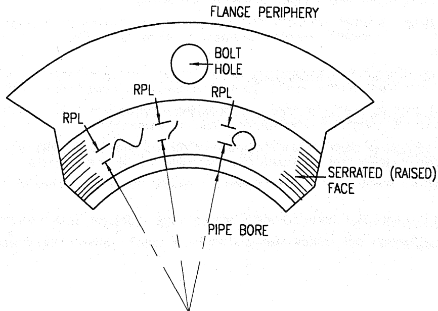
Sketch showing Radial Projected Length (RPL) serrated gasket face damage
