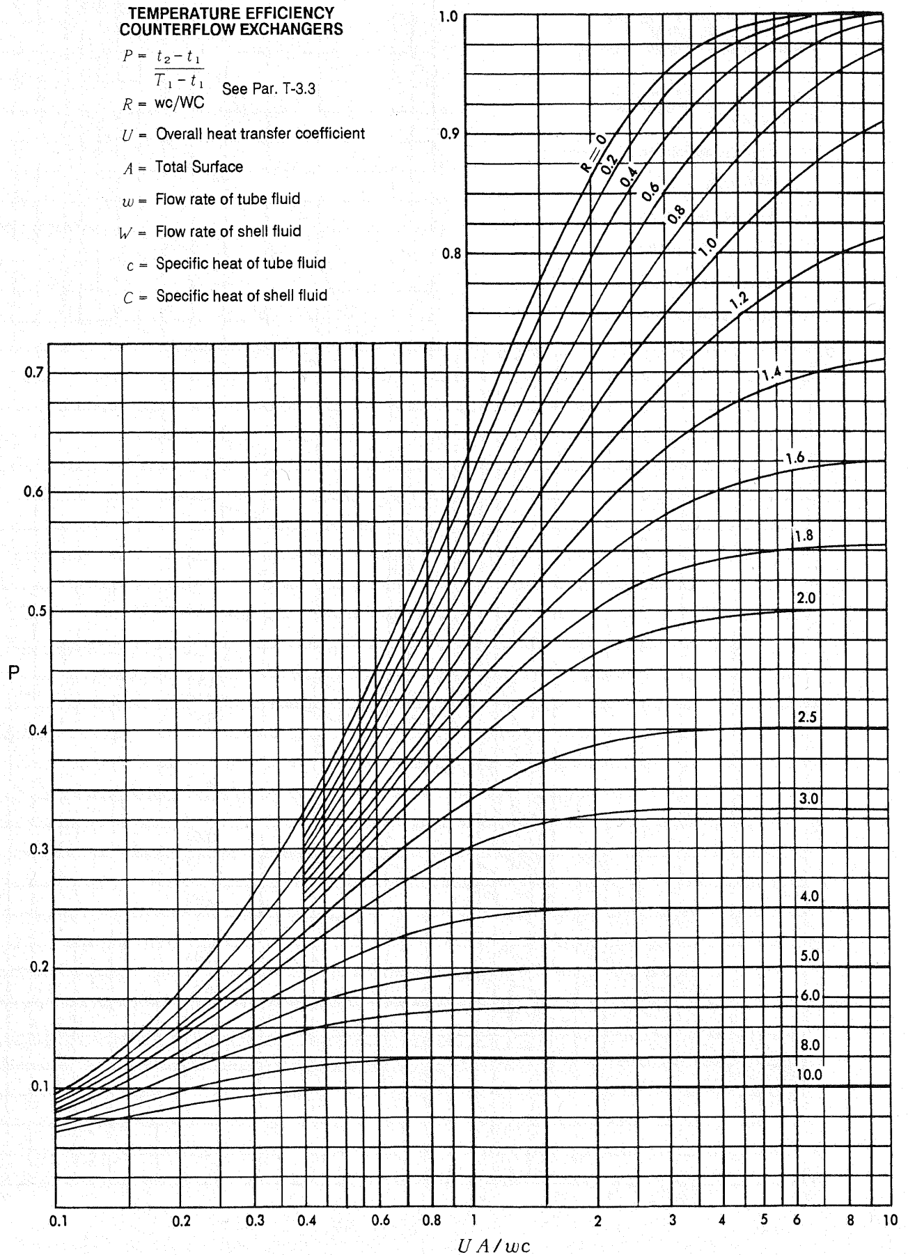
FIGURE T-3.3A
