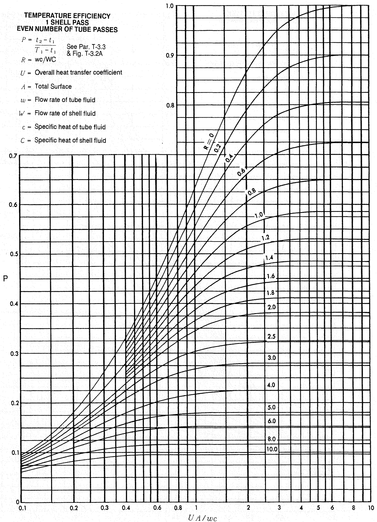
FIGURE T-3.3B
