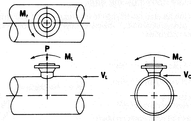
FIGURE RGP-RCB-10.6
