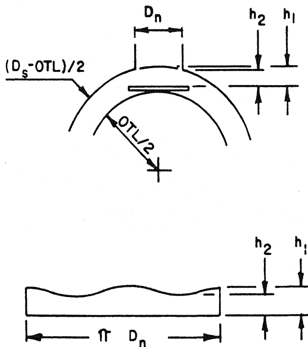
FIGURE RGP-RCB-4.6221 NO IMPINGEMENT PLATE - FULL LAYOUT
