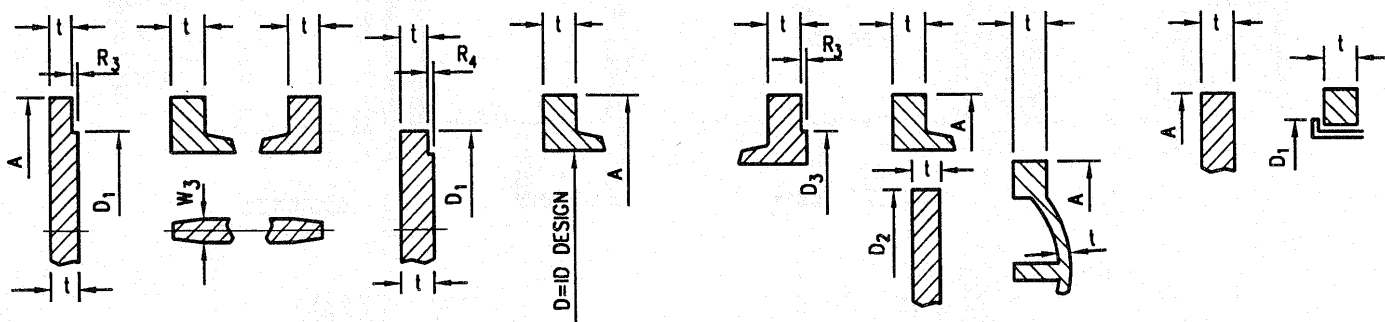
STANDARD UNCONFINED PLAIN FACE JOINT CONSTRUCTION
