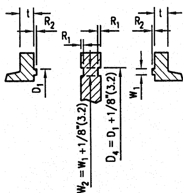
ALTERNATE TONGUE AND GROOVE JOINT
