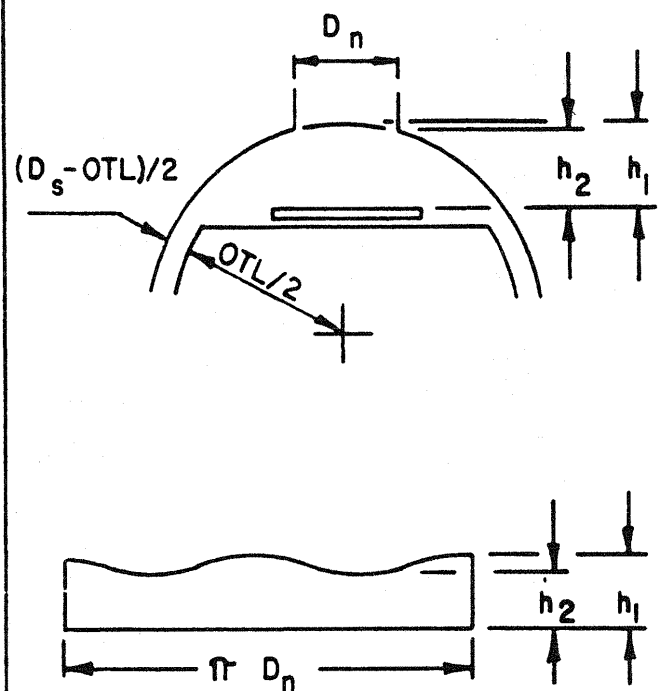
FIGURE RGP-RCB-4.6222 NO IMPINGEMENT PLATE - PARTIAL LAYOUT
