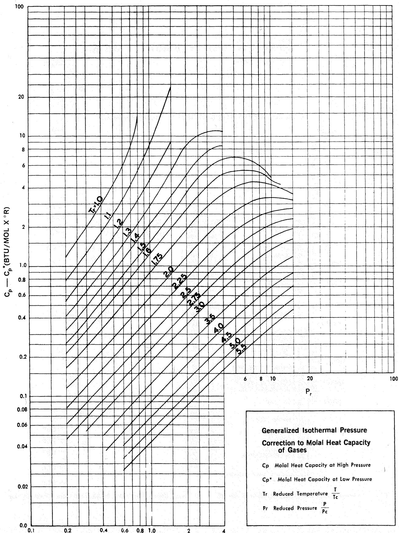
FIGURE P-2.5
