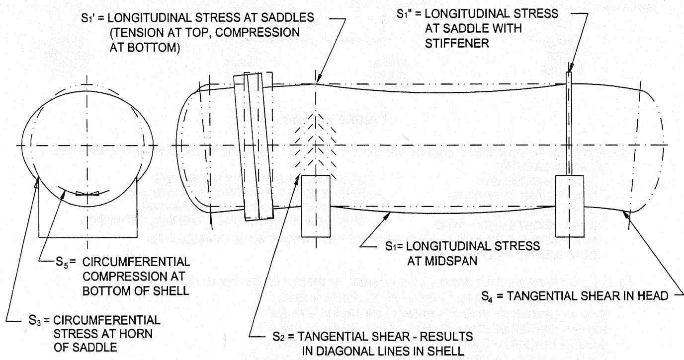
FIGURE RGP-G-7.112
