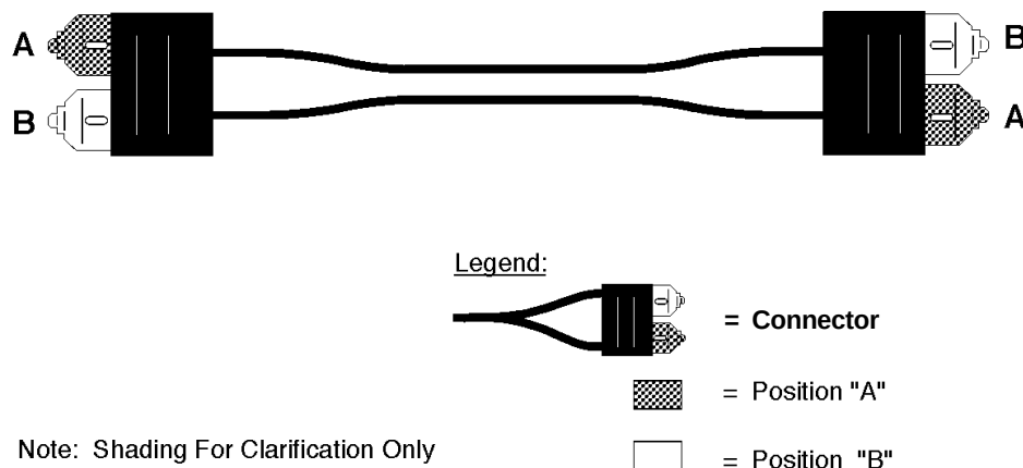
Figure 2 – Optical fiber patch cord
