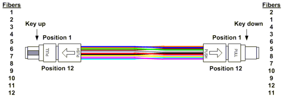
Figure 9 - Type-C array patch cord (pair-wise flipped, key-up to key-down)
