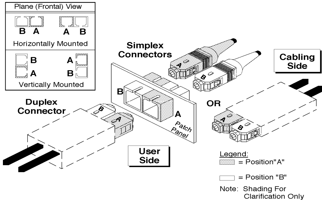
Figure 2 - Position A and B configuration of a 568SC
