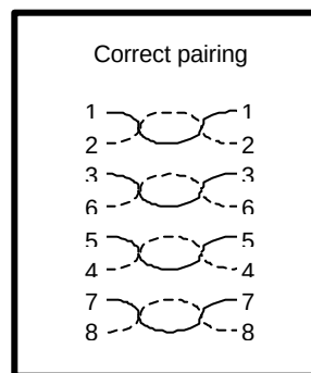
Figure 11-3 Correct pairing
