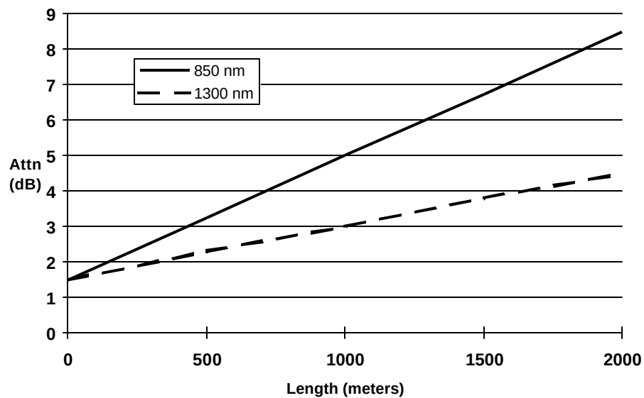
Figure 11-6 62.5/125 \mu\text{m} or 50/125 \mu\text{m} backbone cabling link attenuation based on distance
