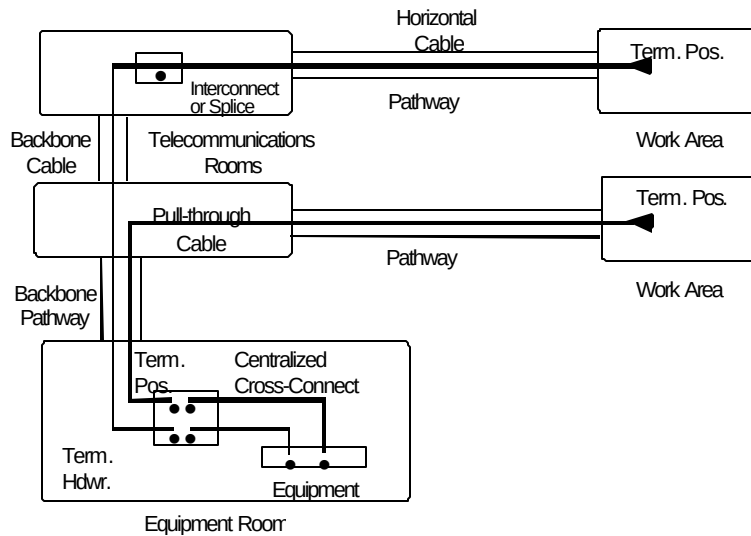
Figure A-1 Centralized optical fiber cabling
