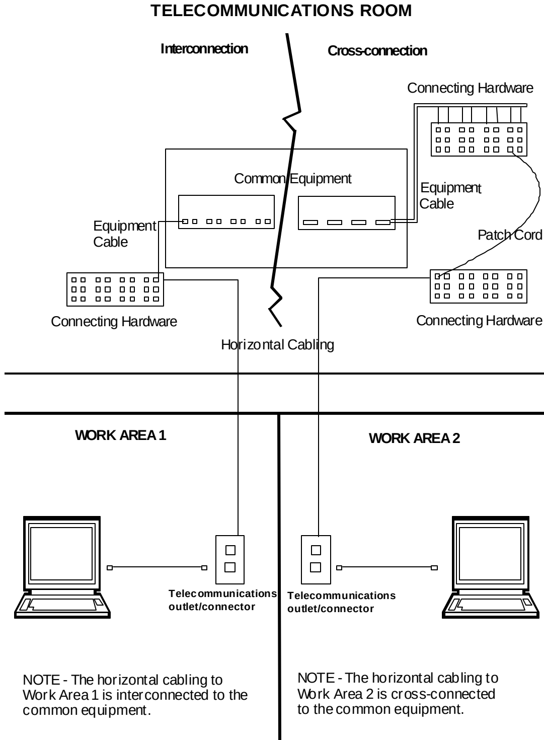
Figure 7-1 Illustration of interconnection and cross-connection schemes
