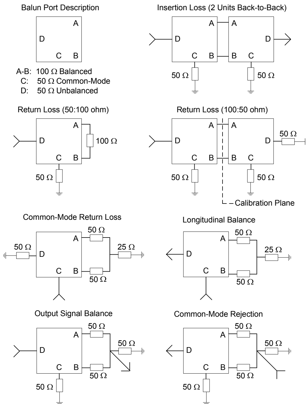
Figure B.3 - Measurement configurations for test balun qualification
