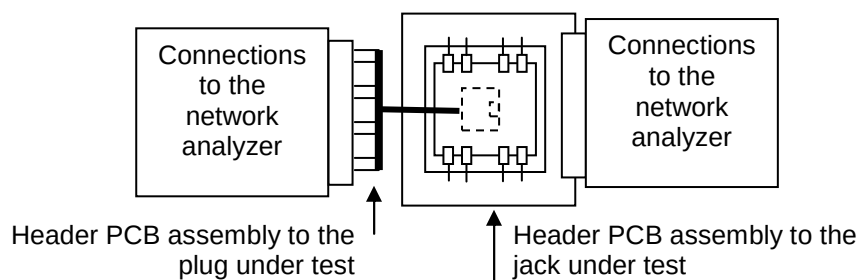
Figure E.20 - Method to minimize distance between planes
