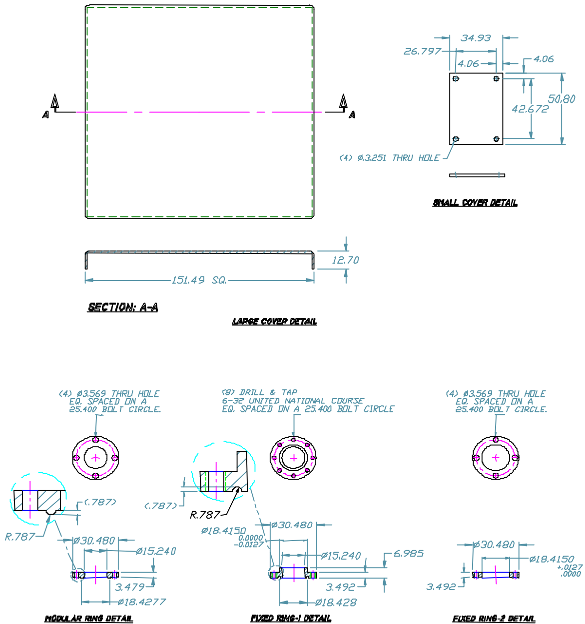
Figure D.3 - HF sealed case covers, fixed and modular ring details
