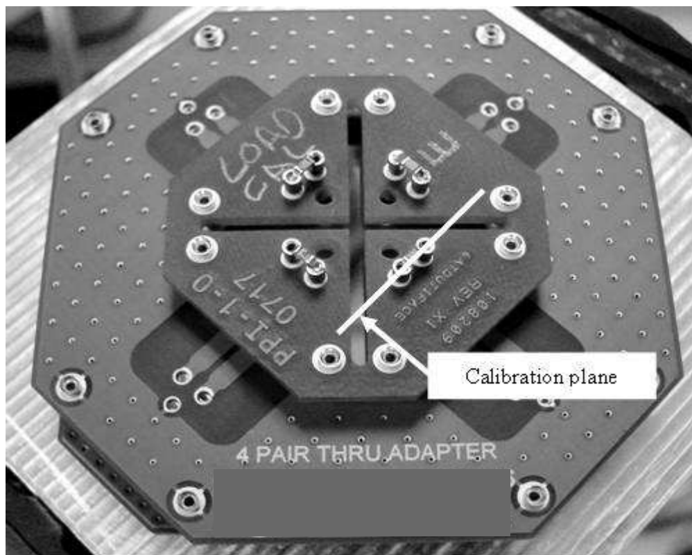
Figure E.17 - Calibration reference plane
