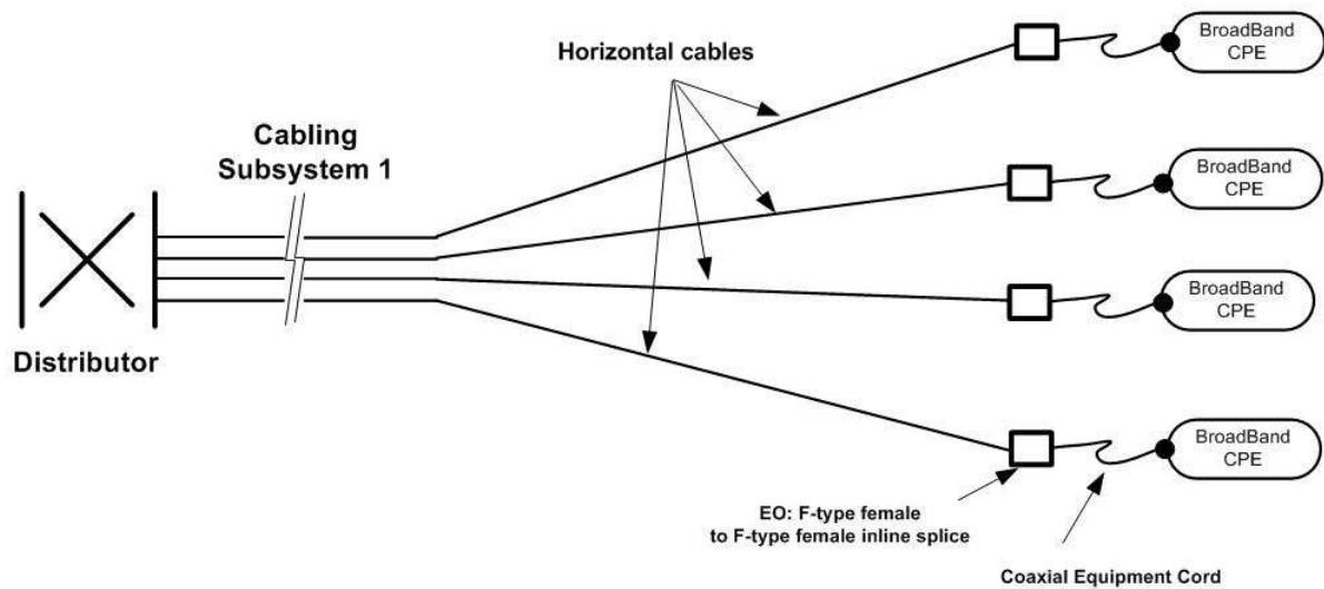
Figure 2 - Example of a star topology
