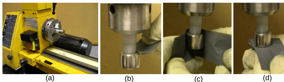
Figure 5: Steel specimen on spindle in chuck of a horizontal lathe (a) and in chuck of a vertical drill press being polished on the top (b), side (c), and bottom (d) with abrasive paper. (7)
