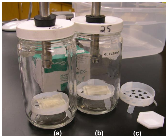
Figure 11: Examples of sample holders for powder, pellet, and liquid forms of VCI materials. (a) Jar on left contains VCI pellets in a small pouch that is placed on a sample holder with legs to maintain position above the level of the glycerin-water mixture; (b) Jar with control sample, an empty pouch on an identical sample holder; and (c) Typical plastic sample holder with holes next to an example of a weighing boat. (13)
