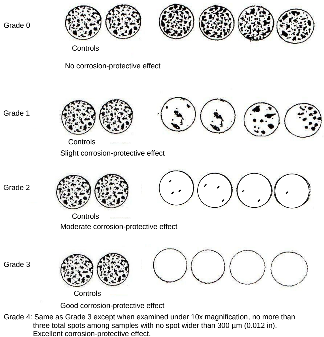
Figure 12: Typical visual patterns for rating the group of specimens according to Paragraph 6.6 with preferred option from Paragraph 3.3 of two Control specimens. (15)
