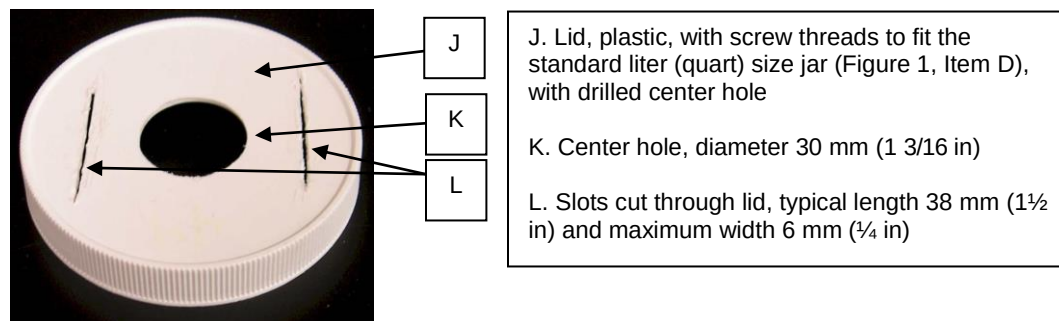
Figure 3: Jar lid used when VCI films and papers are taped to the outside of lid. (3)
