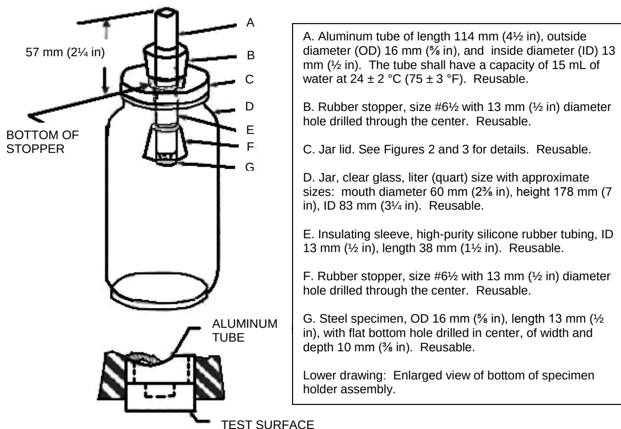
Figure 1: Jar-test apparatus with enlarged view of bottom of specimen holder assembly. All parts of the specimen holder assembly shall be in contact with the adjacent parts. (1)
