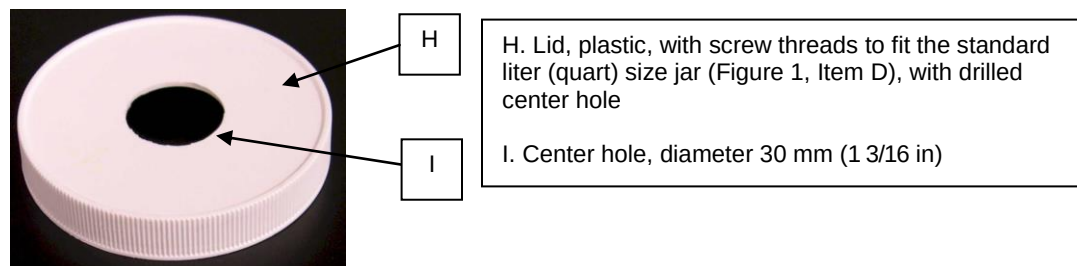
Figure 2: Jar lid used when VCI films and papers are taped to the inside of lid. (2)
