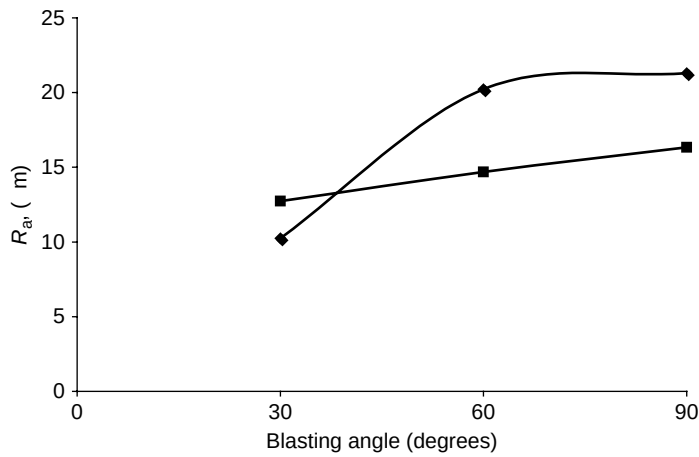
Figure 2.7 Roughness of aluminium AU4G (◆) and carbon steel 100C6 (■) (blasted using alumina grit of size ( d ) of 1400\text{ }\mu\text{m} at a distance ( l ) of 100\text{ mm} ) versus blasting angle (after Mellali et al. , 1997). Reproduced from J. Therm. Spray Technol. , 6(2), 1997, 217–227, ‘Alumina grit blasting parameters for surface preparation in the plasma spraying operation’, M. Mellali, A. Grimaud, A.C. Leger, P. Fauchais and J. Lu, Figure 6, Copyright (1997). With kind permission of Springer Science and Business Media
