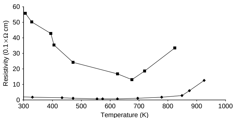
Figure 8.42 Electrical resistivity versus temperature of alloy coatings of atmospheric-plasma sprayed \text{Al}_2\text{O}_3 + 13 \text{ wt\% TiO}_2 (■) and \text{Al}_2\text{O}_3 + 40 \text{ wt\% TiO}_2 (◆) (Ramachandran et al. , 1998). This article was published in Thin Solid Films , 315, K. Ramachandran, V. Selvarajan, P.V. Ananthapadmanabhan and K.P. Sreekumar, 'Microstructure, adhesion, microhardness, abrasive wear resistance and electrical resistivity of plasma-sprayed alumina and alumina-titania coatings', 144–152, Copyright Elsevier (1998)
