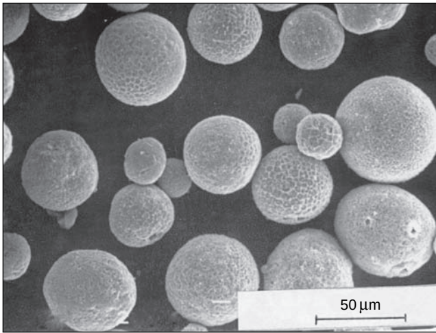
Figure 1.10 Scanning electron micrograph (secondary electrons) of an arc-plasma-densified \text{Cr}_2\text{O}_3 + 5 \text{ wt\% SiO}_2 powder (the initial powder is shown in Figure 1.8). Further details about the processing parameters are given in Table 1.4
