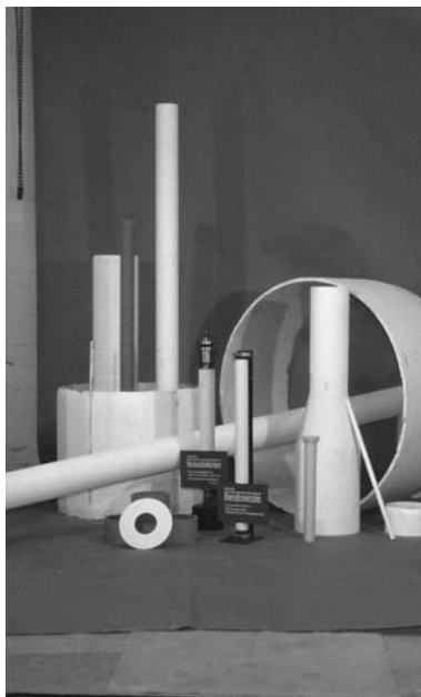
Figure 9.3 Ceramic tubes prepared by a water-stabilized plasma torch. Reproduced by permission of Dr. T. Vilics, LWK Plasmakeramik GmbH, Gummersbach, Germany
