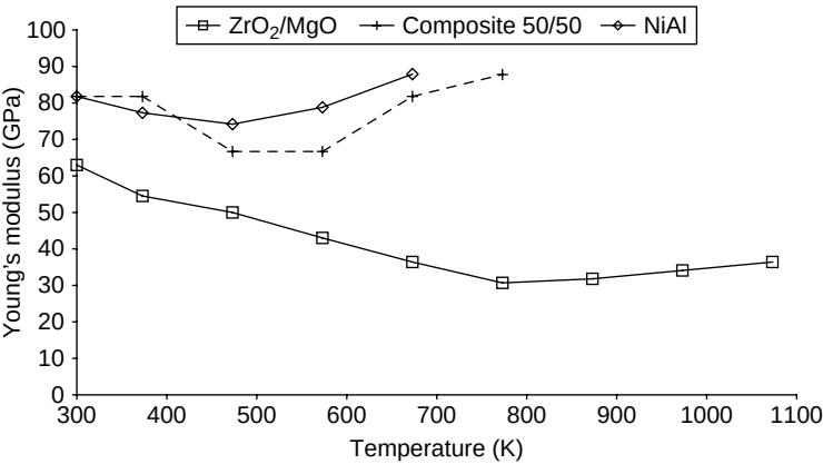
Figure 8.16 Young's modulus versus temperature of the alloy ZrO_2 + 7 \text{ wt\% } MgO ( \square ), the reinforcement Ni + 5 wt% Al ( \diamond ) and a 50/50 (volume/volume) composite of these materials (+), sprayed using the APS technique (see also Table 8.15)
