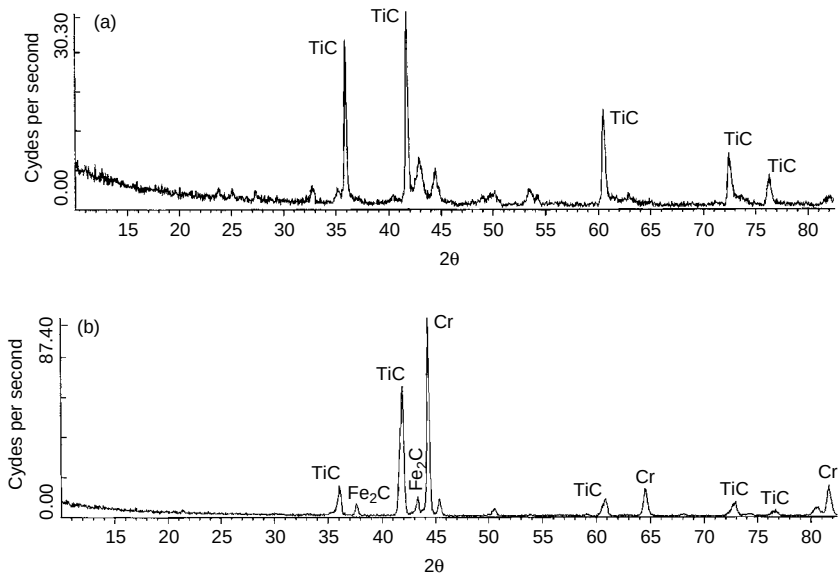
Figure 4.17 XRD diagrams of an FeCr–TiC composite: (a) as-sprayed; (b) laser-glazed. Sample preparation details are shown in Table 4.7
