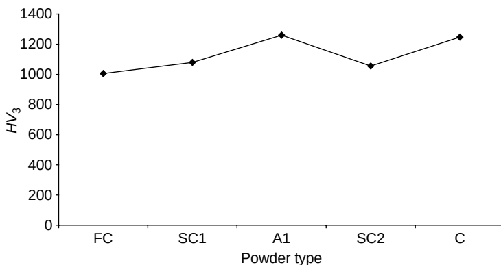
Figure 8.6 Vickers microhardness of chromia coatings (sprayed in air by Pawlowski et al. , 1993) using different arc powers and \text{Cr}_2\text{O}_3 powders having different chemical compositions (in wt%), grain sizes and/or manufacturing techniques: FC – 45.5 kW, 99.8 \text{Cr}_2\text{O}_3 , d_{50\%} = 30.4\ \mu\text{m} , fused and crushed; SC1 – 45.5 kW, bal. \text{Cr}_2\text{O}_3 + 4\text{SiO}_2 + 3\text{TiO}_2 , d_{50\%} = 32.9\ \mu\text{m} , sintered and crushed; A1 – 52.9 kW, \text{Cr}_2\text{O}_3 + 5\text{SiO}_2 , d_{50\%} = 31.29\ \mu\text{m} , agglomerated; SC2 – 44.1 kW, \text{Cr}_2\text{O}_3 + 5\text{SiO}_2 + 3\text{TiO}_2 , d_{50\%} = 73.7\ \mu\text{m} , sintered and crushed; C – 49 kW, ‘pure’ \text{Cr}_2\text{O}_3 , d_{50\%} = 7.4\ \mu\text{m} , crystalline
