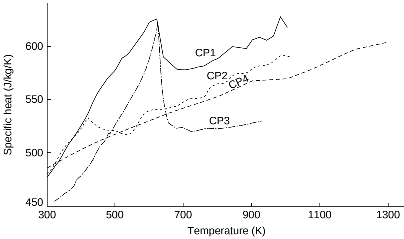
Figure 8.34 Specific heat versus temperature for pure nickel (CP1) and for NiAl coatings plasma-sprayed in air (CP2 and CP4 – described in entries 2 and 3, respectively, of Table 8.24) and in vacuum (CP3 – described in entry 4 of Table 8.24)
