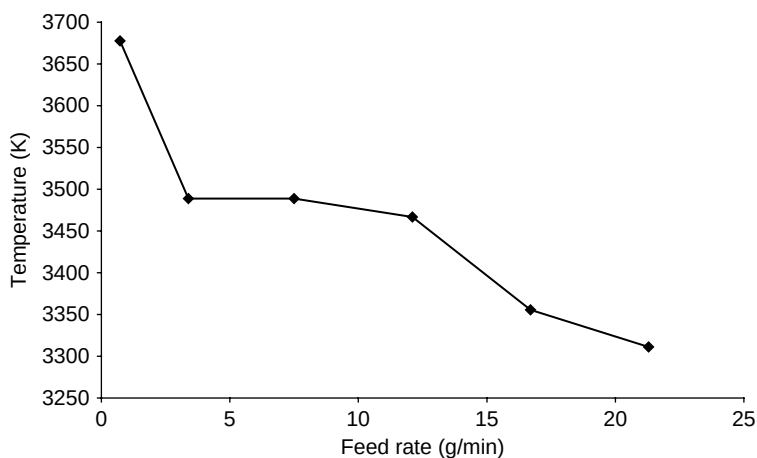
Figure 5.19 Modification of the average centreline temperatures of alumina ( \text{Al}_2\text{O}_3 ) particles having particle sizes in the range -45 to +22.5\mu\text{m} , measured by using two-colour pyrometry as a function of increasing powder feed rate. These measurements were made for a point at a distance of 12 cm from the F-4 plasma torch, supplied with \text{Ar} + \text{H}_2 (32 + 12 slpm), with an electrical power ( P ) of 34.8 kW (after Vardelle et al. , 1992). Reproduced by permission of Vardelle et al. , 1992, Thermal Spray: International Advances in Coatings Technology , C.C. Berndt (Ed.), ASM International, Materials Park, OH, USA, pp. 543–547
