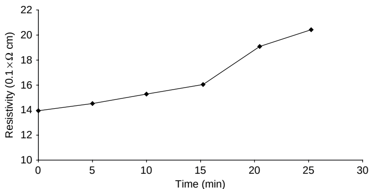
Figure 8.43 Evolution of the electrical resistivity with time of annealing at 673 K for a plasma-sprayed \text{Al}_2\text{O}_3 + 13 \text{ wt\% TiO}_2 coating (Ramachandran et al. , 1998). This article was published in Thin Solid Films , 315, K. Ramachandran, V. Selvarajan, P.V. Ananthapadmanabhan and K.P. Sreekumar, 'Microstructure, adhesion, microhardness, abrasive wear resistance and electrical resistivity of plasma-sprayed alumina and alumina-titania coatings', 144–152, Copyright Elsevier (1998)
