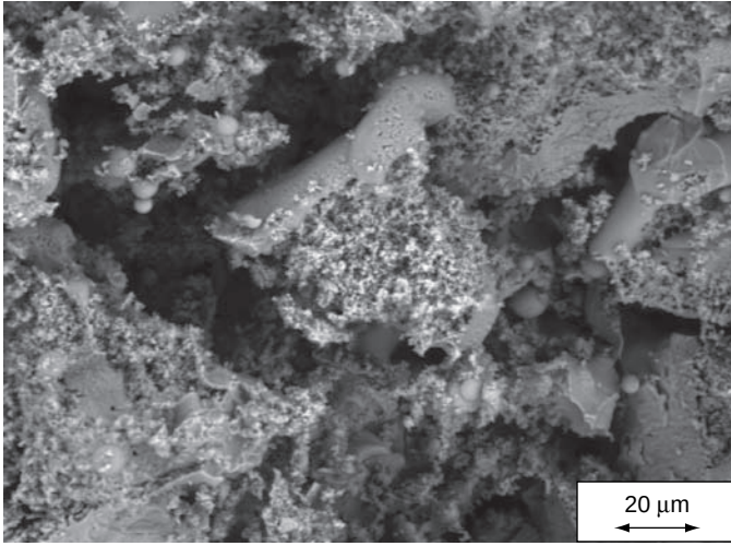
Figure 6.33 Scanning electron micrograph (secondary electrons) of an HAP coating sprayed ‘industrially’ which shows unmelted particles disagglomerated after impact with the substrate (Deram et al. , 2003)
