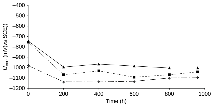
Figure 8.49 Corrosion potential evolution with time of aluminium coatings thermally sprayed using different techniques, as reported by Schiefler et al. , 2003: ♦, flame spraying; ■, arc spraying; ▲, high-velocity oxy-fuel spraying using a wire: SCE, saturated calomel electrode. Further details of the anodic polarization tests are given in Table 8.36. Reproduced by permission of ASM International from M.F.O. Schiefler et al. , 2003, 'Protection of steel components against marine corrosion by thermally sprayed anodic coatings', in Thermal Spray 2003: Advancing the Science, Applying the Technology , C. Moreau and B. Maple (Eds), ASM International, Materials Park, OH, USA, pp. 361–370
