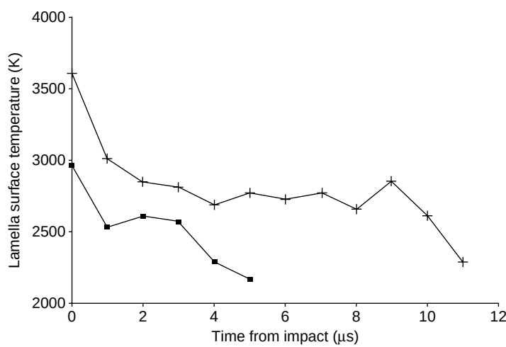
Figure 6.8 Evolution of the temperature of a niobium splat, plasma-sprayed using a powder having a particle size in the range -45 to +22.5\mu\text{m} . The power input to the plasma torch ( P ), supplied with working gases of \text{Ar} + \text{H}_2(50 + 2.7\text{ slpm}) , was 38.5 kW and the glass (+) and steel (■) substrates were placed at a distance of 115 mm from the torch
