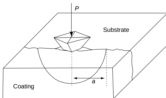
Figure 7.11 Schematic of the interfacial indentation test (Chicot et al. , 1996). This article was published in Thin Solid Films , 283, D. Chicot, P. Démarécaux and J. Lesage, 'Interfacial indentation test for the determination of adhesive properties of thermal sprayed coatings', 151–157, Copyright Elsevier (1996)
