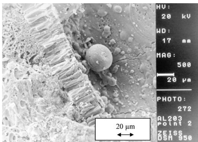
Figure 7.27 Scanning electron micrograph (secondary electrons) of a breakdown channel in an Al 2 O 3 coating obtained by air-plasma spraying. The columnar form of the grains on the channel's boundary indicates the thermal character of the breakdown (Pawlowski, 1987b)
