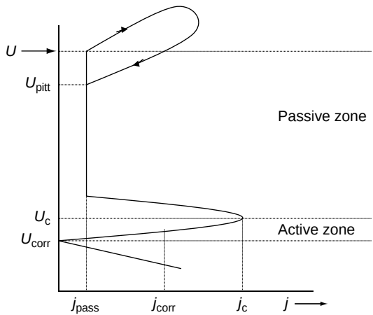
Figure 7.33 Typical curve of the current flowing in the electrolyte of a galvanic cell between the tested sample and the standard electrode as a function of polarization voltage
