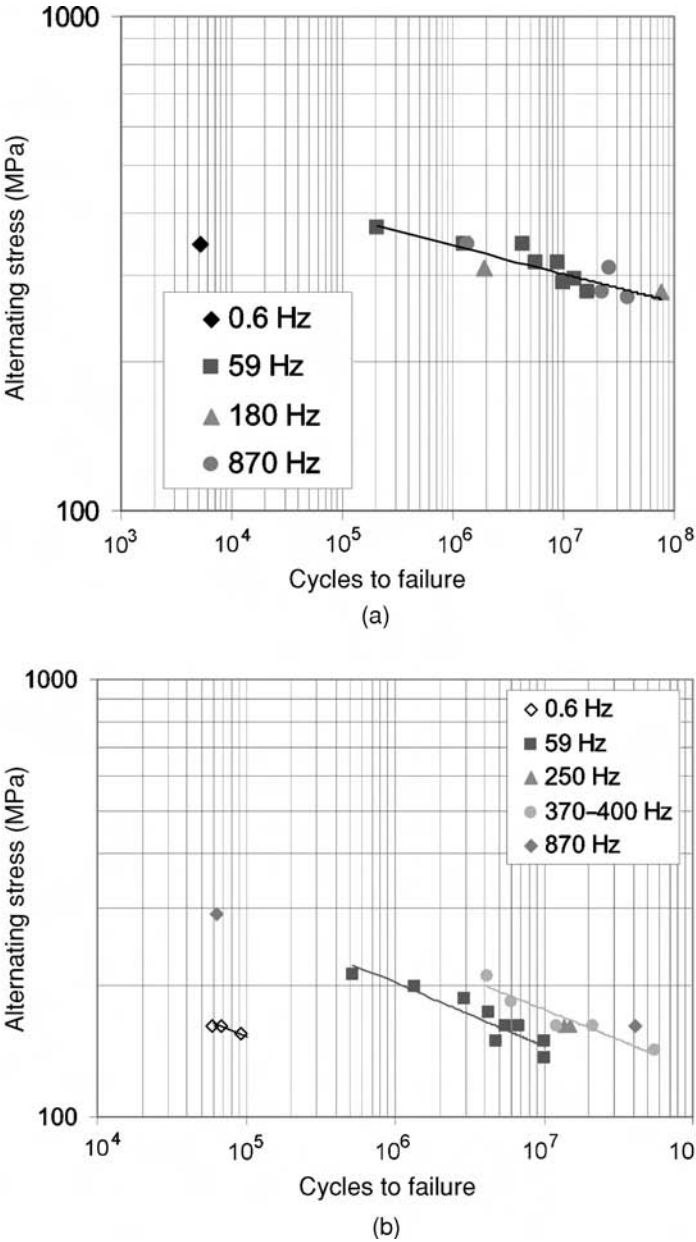
Fig. 3.78. HCF data for coated PW1484 at 1038 °C showing the effect of frequency: (a) R = -1 and (b) R = 0.1 [76].
