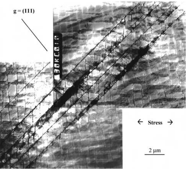
Fig. 3.69. Persistent slip bands in a \langle 001 \rangle -oriented single-crystal superalloy cycled at 700 °C [69], in which the \gamma' particles are sheared.
