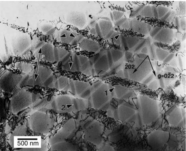
Fig. 3.70. Dislocation microstructure in the AM1 single-crystal superalloy deformed at 950 °C with \Delta\epsilon_{\text{total}} = 1.27\% and with R = 0 [70]. P is the projection of the loading axis. Dislocations are localised at \{001\} interfaces, see arrows marked 1; \{010\} and \{100\} channels, see arrows marked 2, are free of dislocations.
