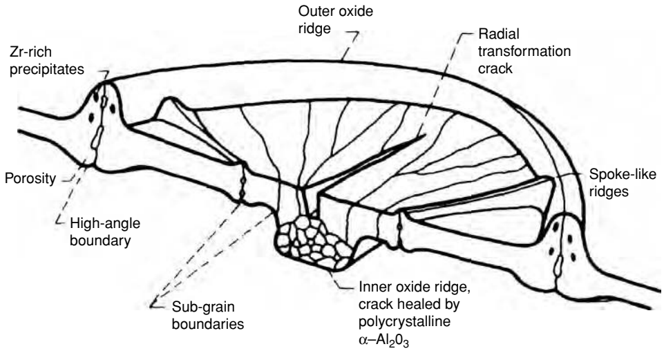
Fig. 5.40. Schematic illustration of the ridged morphology of \alpha -Al 2 O 3 formed on \beta -NiAl, the ridges forming due to the growth occurring from distinct nucleation events [97].
