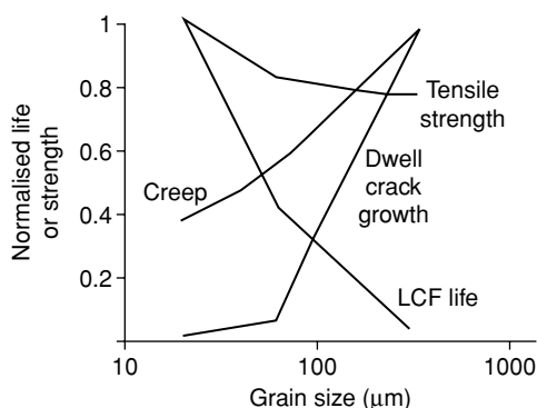
Fig. 4.28. Schematic illustration of the important properties of turbine disc alloys and their dependence upon grain size. After ref. [21].
