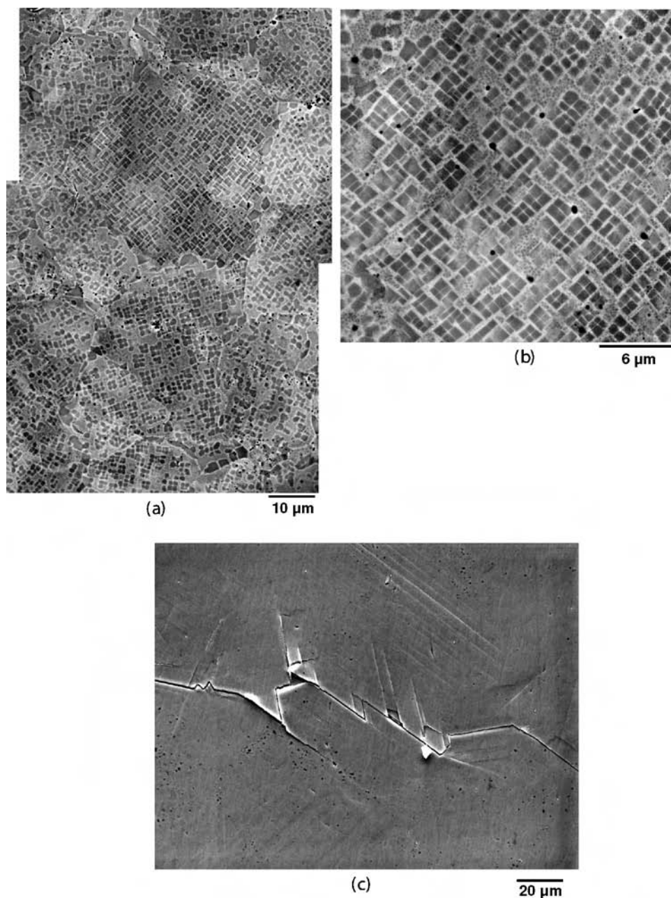
Fig. 4.33. Fracture surfaces for the IN100 P/M superalloy tested in low-cycle fatigue at 0.5 Hz with R = 0.05 [27]. (a), (b) SEM images of the {001} fracture surfaces typical of failure at 538 °C, showing the presence of cuboidal facets belonging to the \gamma' phase. (c) {111} fracture surface typical of fatigue crack growth at room temperature – note that the fracture path is parallel to the traces of the slip lines in the top right of the image.
