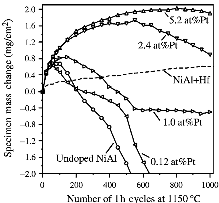
Fig. 5.44. Specimen mass change during oxidation (1 h cycles at 1150 °C in dry, flowing O 2 ) for various near-stoichiometric NiAl alloys alloyed with Pt [105].
