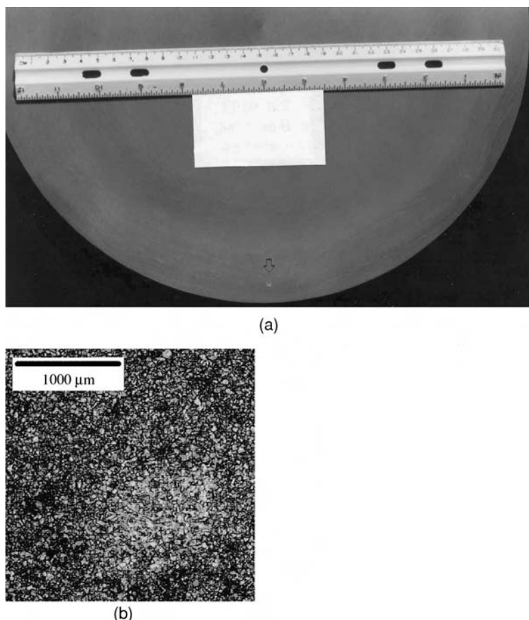
Fig. 4.8. White-spot defect in the IN718 superalloy: (a) its appearance on a cross-section of a macroetched billet; (b) optical micrograph. (Courtesy of Laurence Jackman.)
