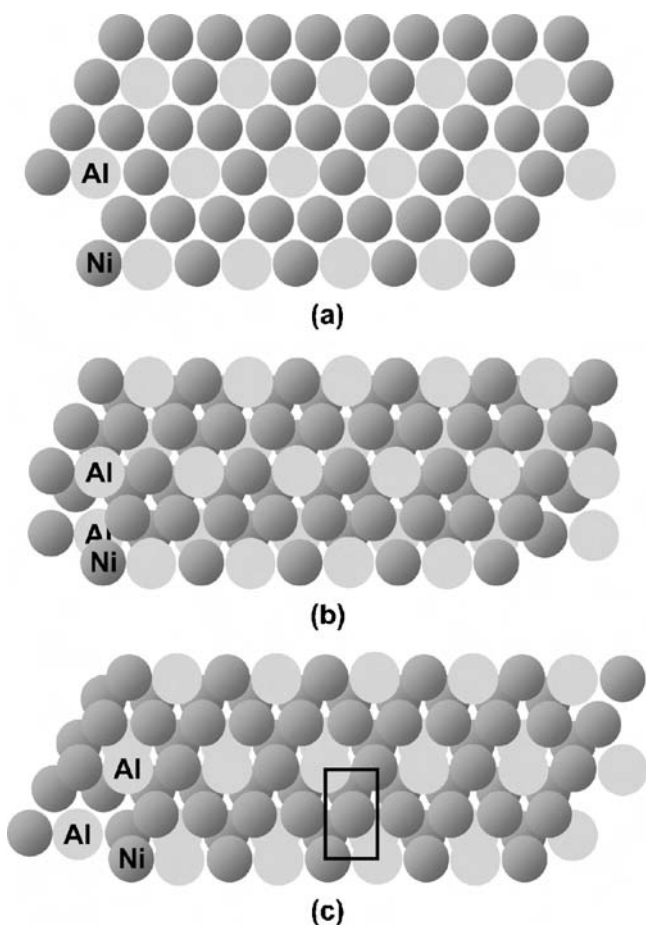
Fig. 2.37. (a) Representation of the \{111\} plane of the L_{12} crystal structure of \text{Ni}_3\text{Al} . (b) Two such planes stacked according to the crystal structure. (c) Situation after displacing the second plane by a/2(1\bar{1}0) on \{111\} . One forbidden bond is formed in the area marked.
