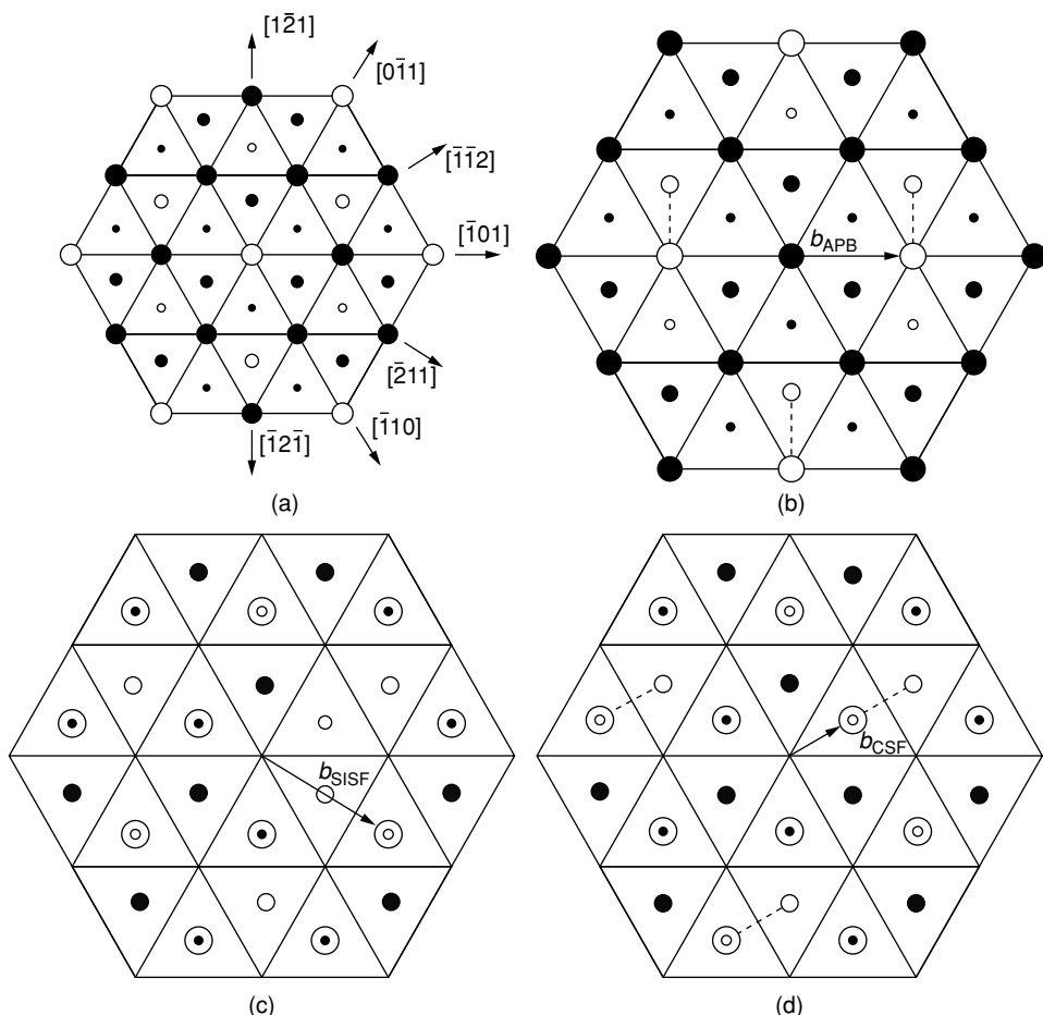
Fig. 2.39. Illustration of various faults possible in the L_2 structure formed by shearing \{111\} planes past one another: (a) three successive \{111\} planes, unfaulted; (b) after shearing the top layer by a/2\langle\bar{1}01\rangle to form an anti-phase boundary (APB); (c) after shearing by a/3\langle\bar{2}11\rangle to form a superlattice intrinsic stacking fault (SISF); (d) after shearing by a/6\langle\bar{1}12\rangle to form a complex stacking fault (CSF). Note that the large, medium and small circles represent atoms in the top, middle and bottom planes, respectively [36].
