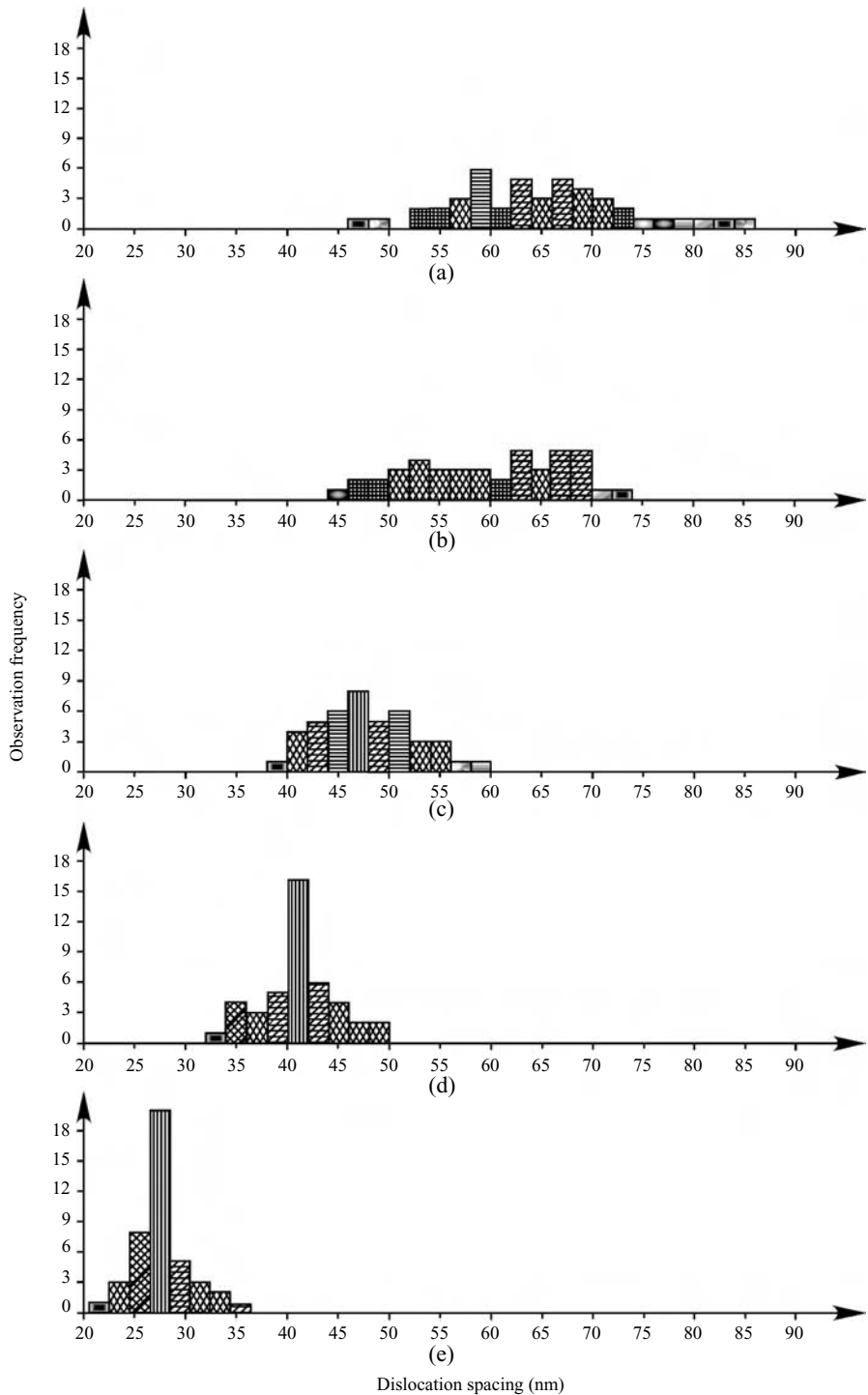
Fig. 3.65. Measurements of the equilibrium \gamma/\gamma' dislocation spacings in (a) TMS-75(+Ru), (b) TMS-75, (c) TMS-75(+Mo), (d) TMS-138 and (e) TMS-162 tested at 1100 °C and 137 MPa [64,65]; taken with the data in Figure 3.64, a strong creep strengthening effect is confirmed when the dislocation spacing is small.
