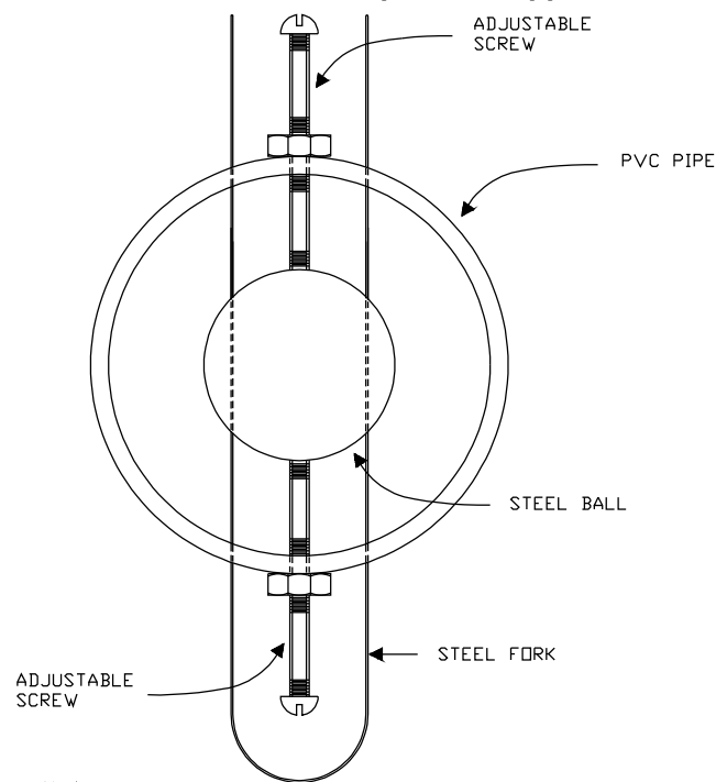
Figure 5.2 Release device for impact test apparatus
