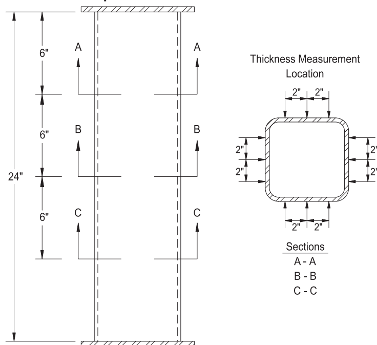
Figure 4.4 Steel tube sample – location of thickness measurements
