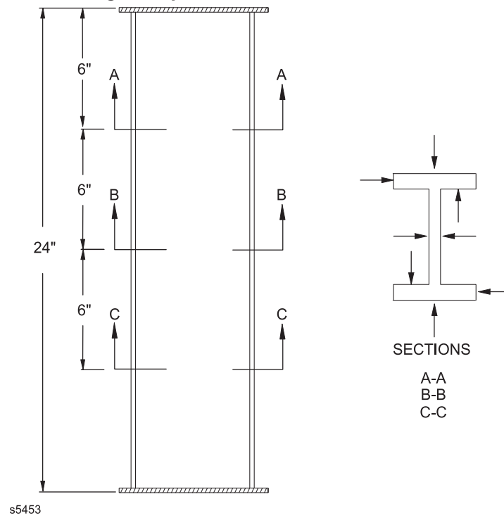
Figure 4.5 Steel wide flange sample – location of thickness measurements
