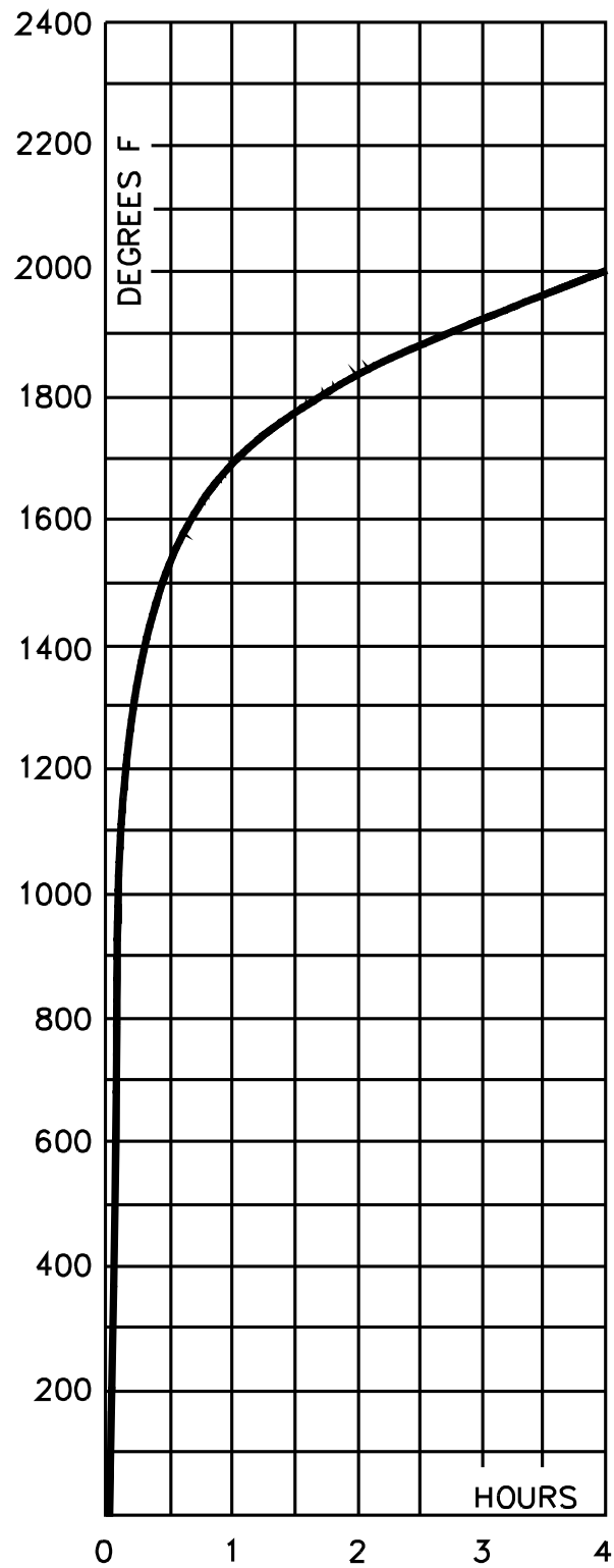
Figure 8.1 Time-temperature curve
