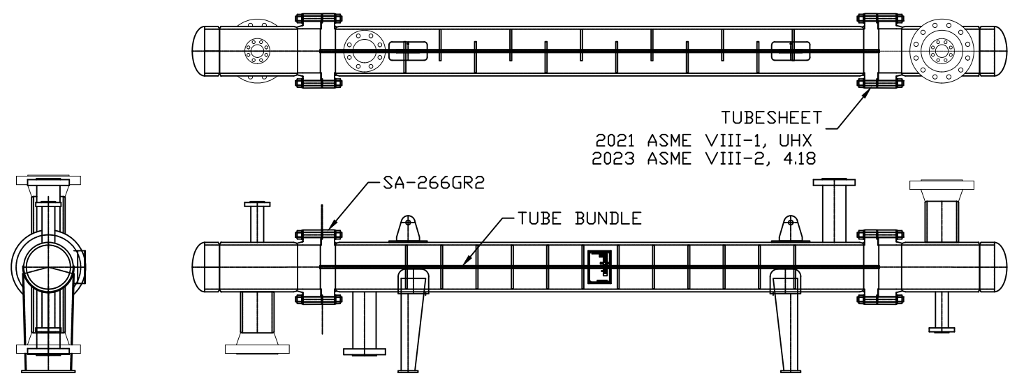
HEAT EXCHANGER
