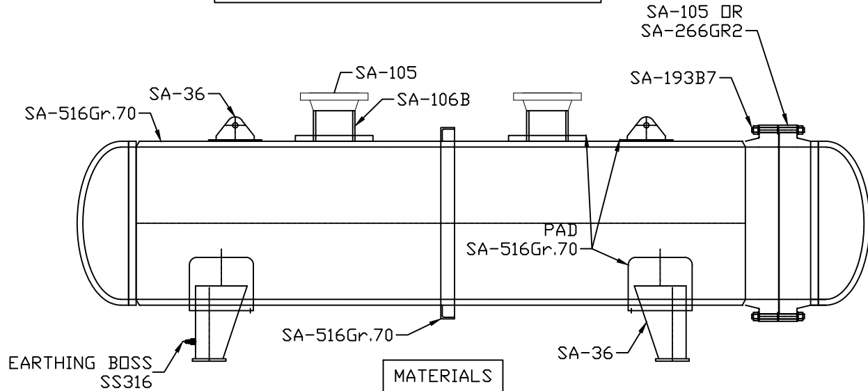
PRESSURE VESSEL
