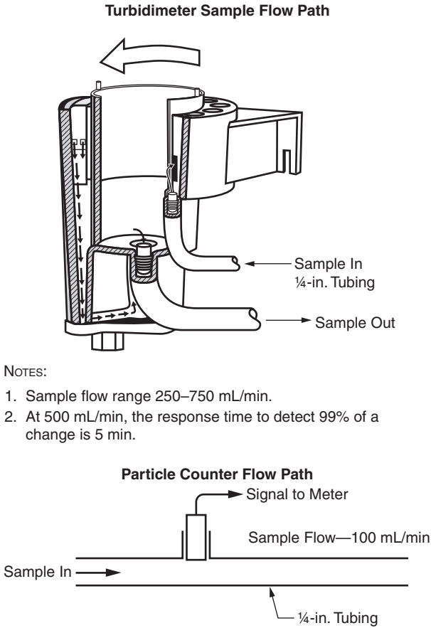
Figure 12-2 Particle counts versus turbidity
