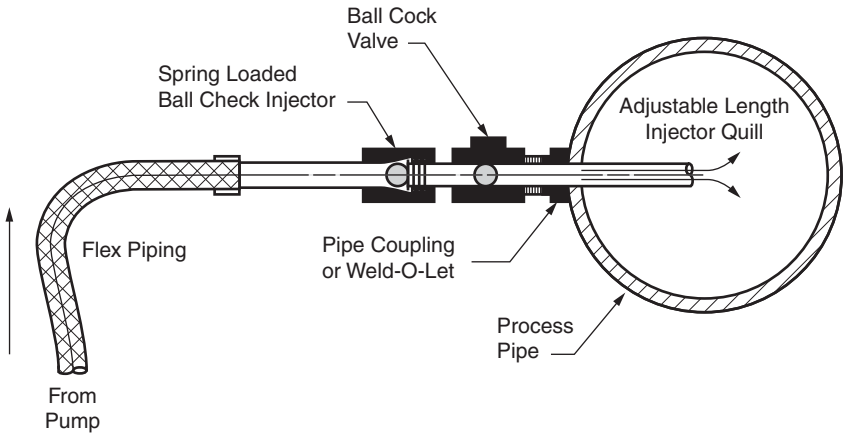
Figure 6-1 Injection assembly
