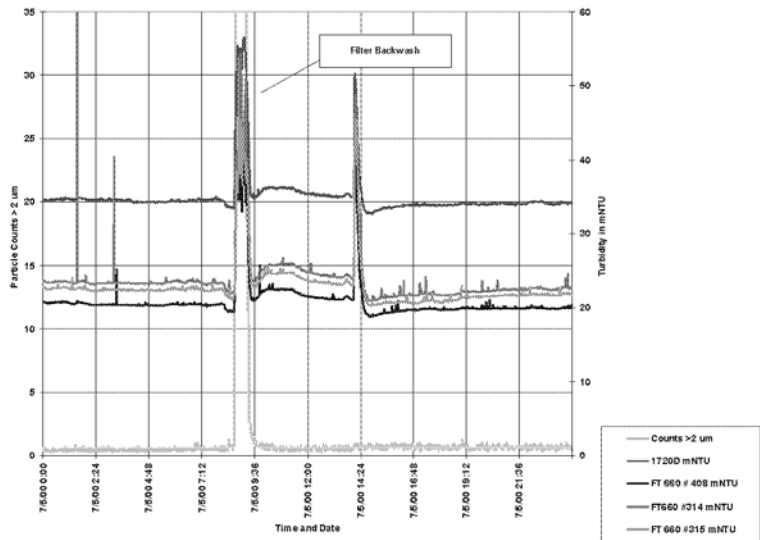
Figure 7 Water Treatment Plant Filter #12 Effluent Particulate Monitoring (07/05/00)
