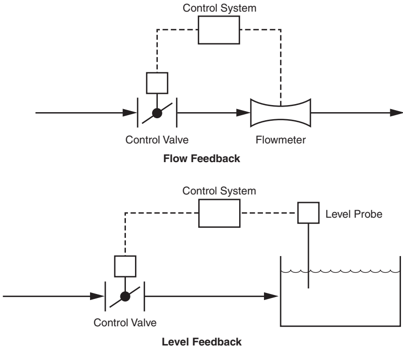
Figure 9-5 Proportional integral derivative (PID) control
