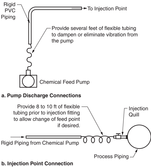
Figure 11-2 Chemical feed piping connections
