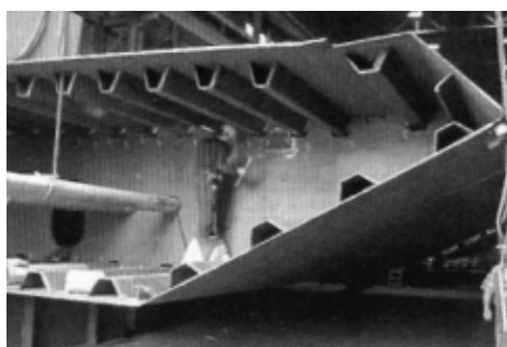
Figure 6. Storda Bridge.
