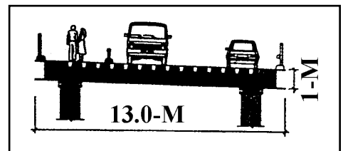
Figure 4. Nordhordland Floating Bridge.
