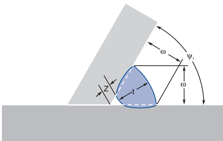
Figure 4. Z-loss.
