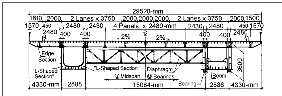
Figure 7. Twin box girder bridge crossing the Oka River, Russia (split-section).
