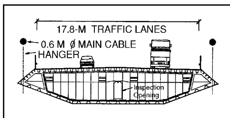
Figure 8. High Coast, Sweden, section.
