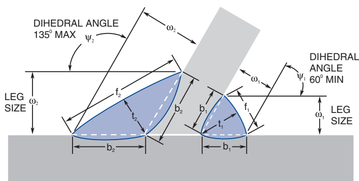
Figure 1. Equal throat sizes ( t_1 = t_2 ).
