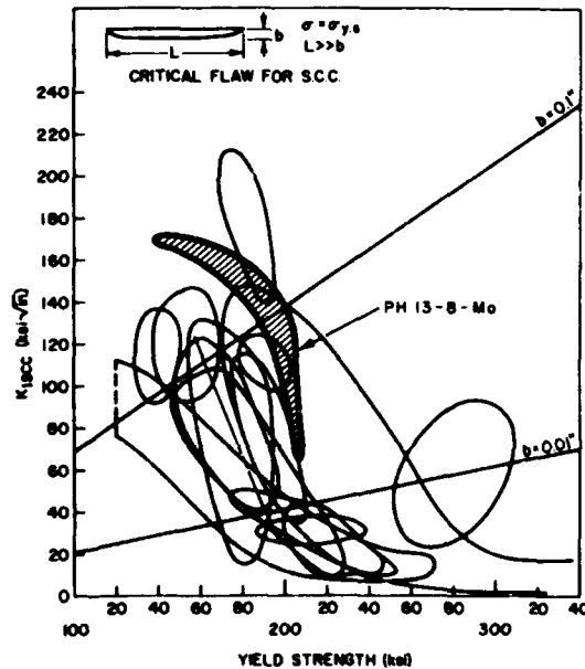
Fig. 38. Envelope of K_{Isc} values of PH 13Cr-8Ni-Mo steel (heavy lines) compared to composite of K_{Isc} envelopes for the other steels.
