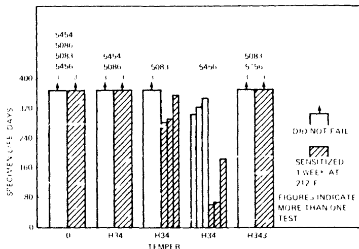
Fig. 24. Stress corrosion resistance of stressed preformed specimens of several alloys of Al-Mg-Mn alloy sheet (0.064 in.) exposed to 3.5% NaCl solution by alternate immersion. In the O temper, alloys with Mg content up to 5.5% (5456) exhibit an excellent resistance to SCC. Strain-hardened and stabilized tempers such as H34 have a low resistance when Mg content is in the 4.0 to 5.5% range, as in alloys 5083 and 5456. Special tempers such as H343 have been developed to provide a high resistance to SCC for the latter alloys [55].
