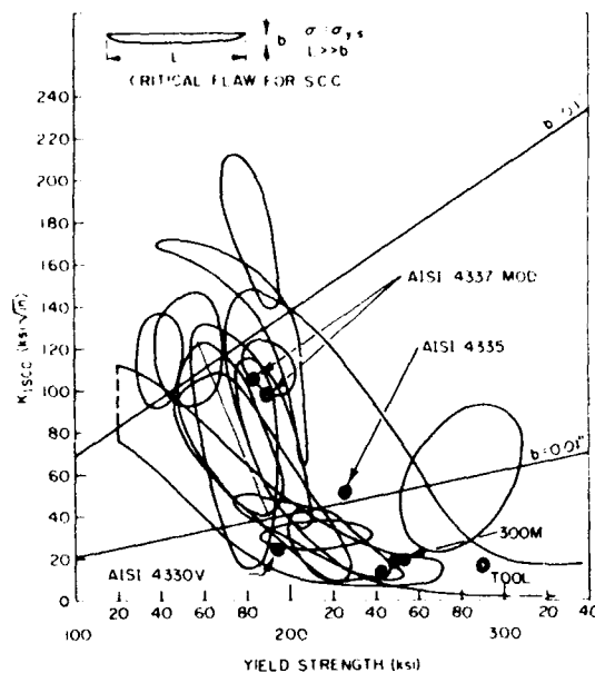
Fig. 41. Single value K_{Isc} data for a variety of steels, superimposed on a collection of K_{Isc} envelopes.
