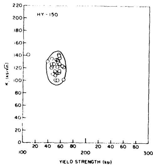
Fig. 8. Stress corrosion resistance and fracture toughness of HY-150 steel [89-91].
