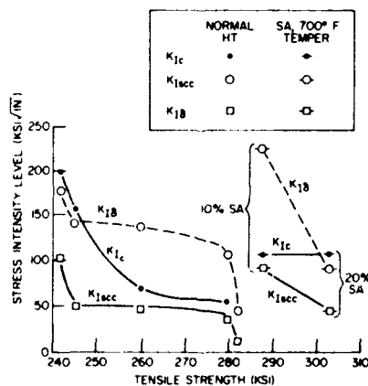
Fig. 59. Variation in K_{Ic} , K_{Isc} and K_{I6} of A5C-77 steel as a function of strength for conventionally treated and strain-aged material (from Ref. 123). K_{I6} is an estimate of fracture toughness based on the terminal purely mechanical fracture in a stress corrosion test.
