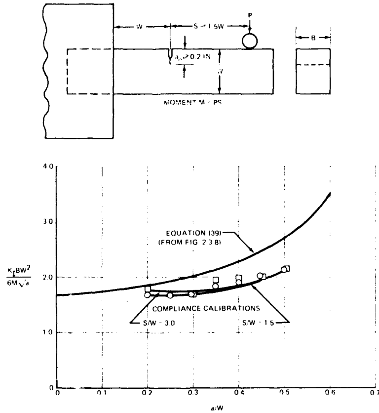
Fig. 10. Configuration and comparison of K_I calibrations for cantilever-loaded, single-edge-cracked plate bend specimens.
