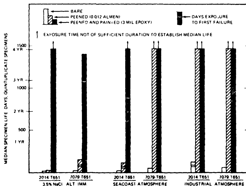
Fig. 43. Comparison of the effect of alloy and environment on the protection against SCC afforded by peening and peening plus painting on specimens stressed in the short transverse direction to 75% of their yield strength [193].
