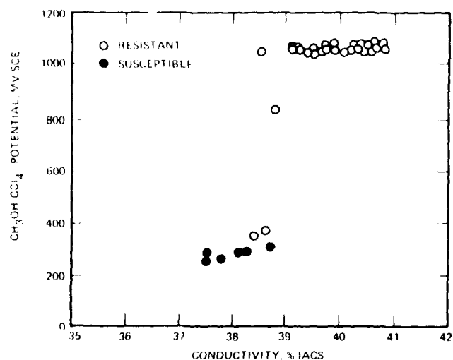
Fig. 36. Comparison of the ability of electrical conductivity and \text{CH}_3\text{OH}-\text{CCl}_4 potential to distinguish between the exfoliation-resistant and susceptible conditions of 36 production lots of 7178-T76 sheet [108]. From Corrosion 26, p. 116, Fig. 11; copyright 1970 by the National Association of Corrosion Engineers. Used by permission.
