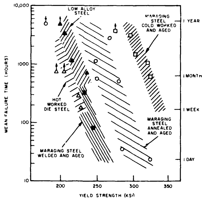
Fig. 3. Results of bent-beam tests in aerated distilled water. These specimens were exposed to the environment at stress of 75% of yield (from Ref. 48). From Mater. Protect. 4 (No. 12), 28 (1965); copyright by the National Association of Corrosion Engineers. Used by permission.
