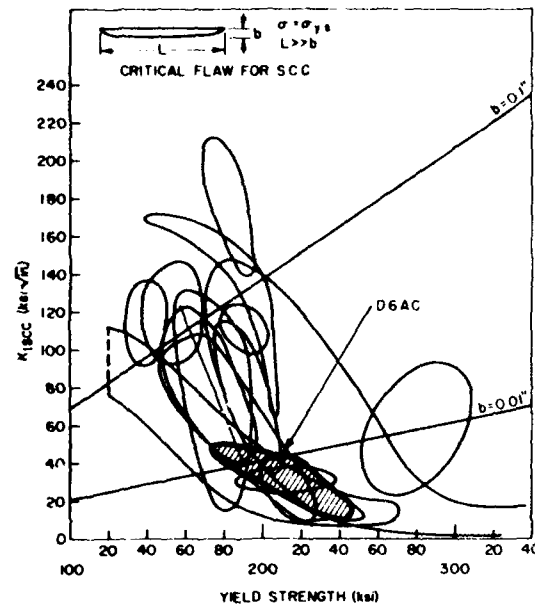
Fig. 29. Envelope of K_{Isc} values for D6AC steel (heavy lines) compared to composite of K_{Isc} envelopes for the other steels.
