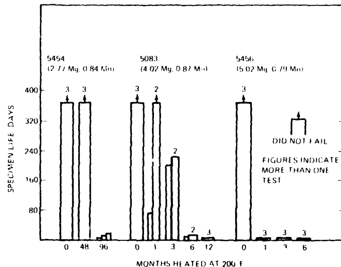
Fig. 25. Effect of heating on resistance to SCC of stressed, pretomed specimens of Al-Mg-Mn alloy sheet (0.064 in.) exposed to 3.5% NaCl solution by alternate immersion. Strip specimens of O temper sheet were plastically deformed at room temperature prior to the 200°F exposure. Only the lower-magnesium-content alloy 5454 maintained a high resistance to SCC after prolonged heating at 200°F [55]. From Proceedings of Conference on Fundamental Aspects of Stress Corrosion Cracking , 1969, p. 476, Fig. 10; copyright by the National Association of Corrosion Engineers. Used by permission.
