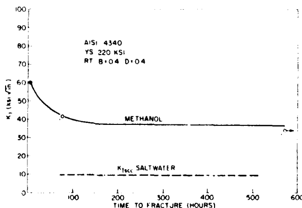
Fig. 66. Comparison of the values of K_{Isc} in methanol and in salt water for AISI 4340 steel.
