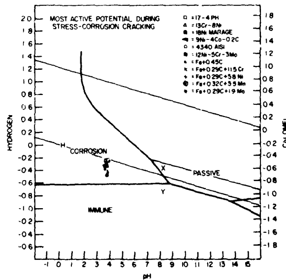
Fig. 68. Values of potential and pH at the crack tips of several steels during stress corrosion crack propagation.
