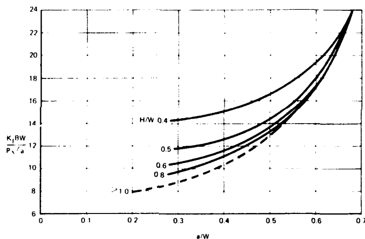
Fig. 5. Comparison of K_I calibrations represented by Eqs. (24) and (25) for (W-a) -indifferent, crackline-loaded, single-edge-cracked plate specimens.
