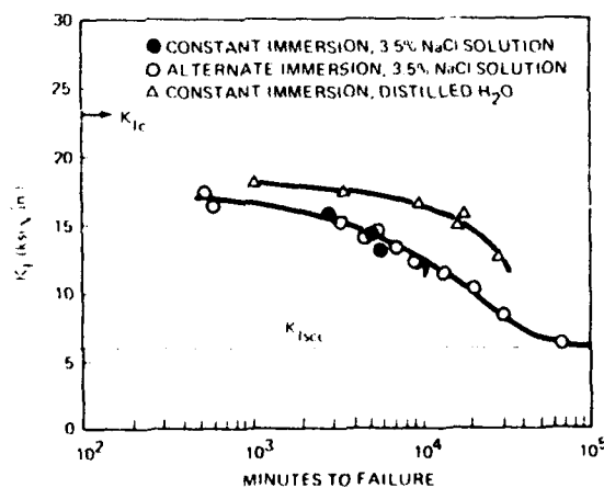
Fig. 10. Precracked-specimen stress corrosion data for short transverse 7075-T651 plate illustrating the TTF method of obtaining K_{ISCC} . Using this technique, a K_{ISCC} of about 6 ksi \sqrt{\text{in.}} is obtained [61]. From Symposium on Stress Corrosion Testing , Atlantic City, 1966, p. 24, Fig. 1; copyright by the American Society for Testing and Materials. Used by permission.
