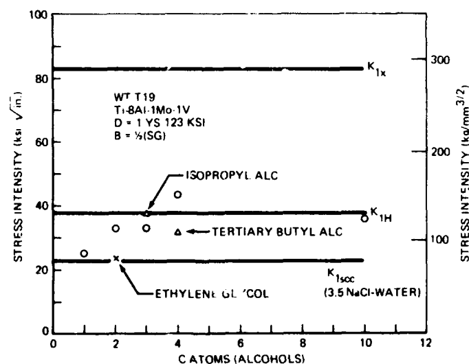
Fig. 28. Apparent threshold stress intensity ( K_{Isc} in 360 min) for Ti-8Al-1Mo-1V tested in alcohols with increasing number of carbon atoms. ( K_{IH} refers to a threshold for slow crack growth in an inert environment, perhaps caused by internal hydrogen) [67]. From Proceedings of Conference on Fundamental Aspects of Stress Corrosion Cracking , 1969, p. 687, Fig. 1; copyright by the National Association of Corrosion Engineers. Used by permission.
