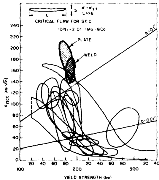
Fig. 36. Envelopes of K_{Isc} values of 10Ni-2Cr-1Mo-8Co steel and welds (heavy lines) compared to composite of K_{Isc} envelopes for the other steels.
