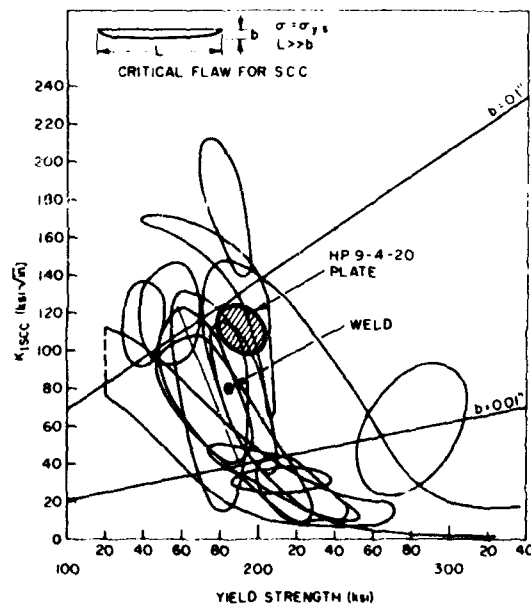
Fig. 30. Envelopes of K_{Isc} values of HP 9-4-20 steel and welds (heavy lines) compared to composite of K_{Isc} envelopes for the other steels.
