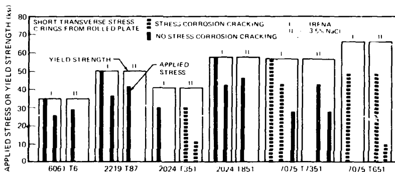
Fig. 20. Comparison of smooth-specimen resistance to SCC of various alloys in inhibited red fuming nitric acid at 165^\circ\text{F} and in 3.5% NaCl alternate immersion [79]. From Proceedings of Conference on Fundamental Aspects of Stress Corrosion Cracking , 1969, p. 24, Fig. 1; copyright by the National Association of Corrosion Engineers. Used by permission.
