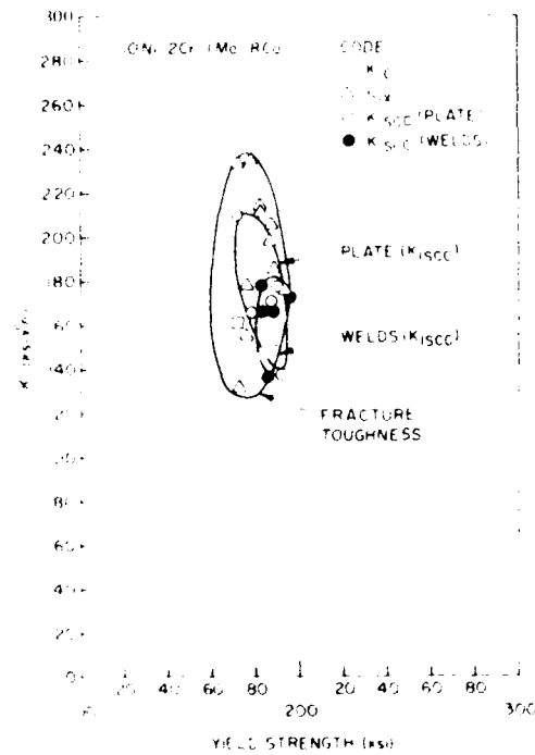
Fig. 19. Stress corrosion resistance and fracture toughness of 10Ni-2Cr-1Mo-8Cu steel and weldments [81,87,94,95,99,116-120]
