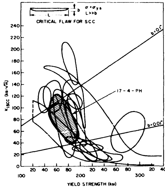
Fig. 37. Envelope of K_{Isc} values of 17-4-PH steel (heavy lines) compared to composite of K_{Isc} envelopes for the other steels.
