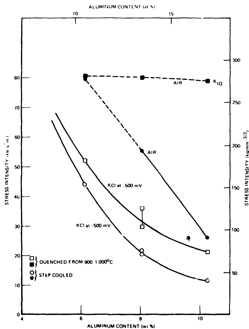
Fig. 31. Variation of K_{Ic} and K_{Isc} with aluminum content and heat treatment in binary titanium-aluminum alloy [30]. From Proceedings of Conference on Fundamental Aspects of Stress Corrosion Cracking , 1969, p. 630, Fig. 20a; copyright by the National Association of Corrosion Engineers. Used by permission.
