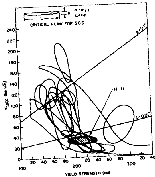
Fig. 28. Envelope of K_{Isc} values for H-11 steel (heavy lines) compared to composite of K_{Isc} envelopes for the other steels.
