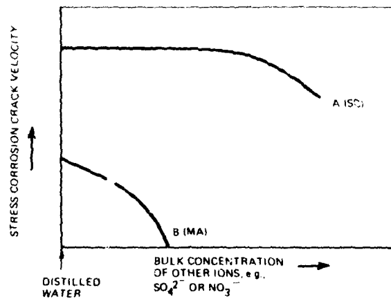
Fig. 25. Schematic of the influence of other ions and metal-lurgical factors on crack velocity.
