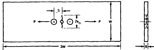
Fig. 15. Configuration and K_I calibration of the crackline-loaded, center-cracked plate specimen.
