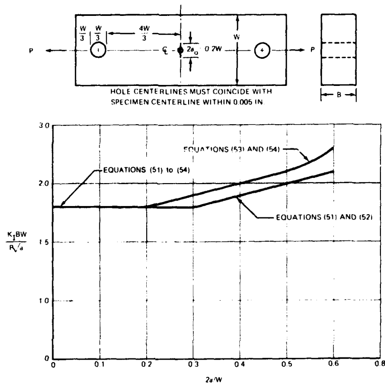
Fig. 14. Configuration and K_I calibration of the remote-loaded, center-cracked plate specimen.
