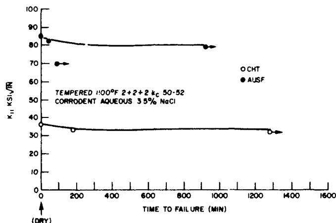
Fig. 58. Pre-crack cantilever stress corrosion results for ausformed and conventionally heat treated H-11. Corrodent, 3.5% NaCl solution (from Ref. 93). From Metals Eng. Quart. 8 (No. 4), 2; copyright 1968 by American Society for Metals. Used by permission.
