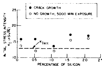
Fig. 51. Effect of silicon on threshold stress intensity K_{I_{SCC}} (202 to 241-ksi yield strength range) (from Ref. 67). From Corrosion 25 (No. 10), 423-431 (1965); copyright by the National Association of Corrosion Engineers. Used by permission.
