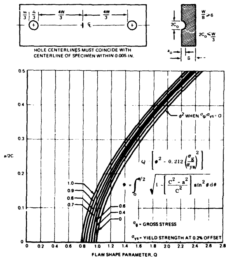
Fig. 16. Configuration and K_I calibration of the surface-cracked plate specimen.
