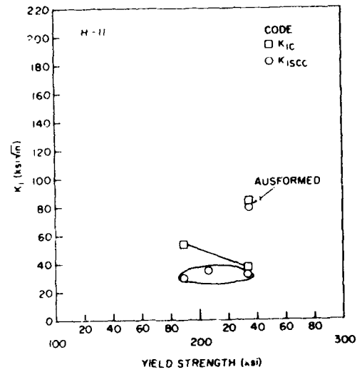
Fig. 9. Stress corrosion resistance and fracture toughness of H-11 steel [27,62,63,92,93].
