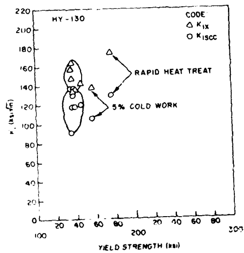
Fig. 6. Stress corrosion resistance and fracture toughness of HY-130 steel [11,77-81].
