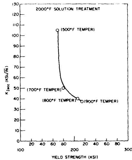
Fig. 53. Effect of yield strength on the K_{Isc} value of AFC-77 steel (from Ref. 123).
