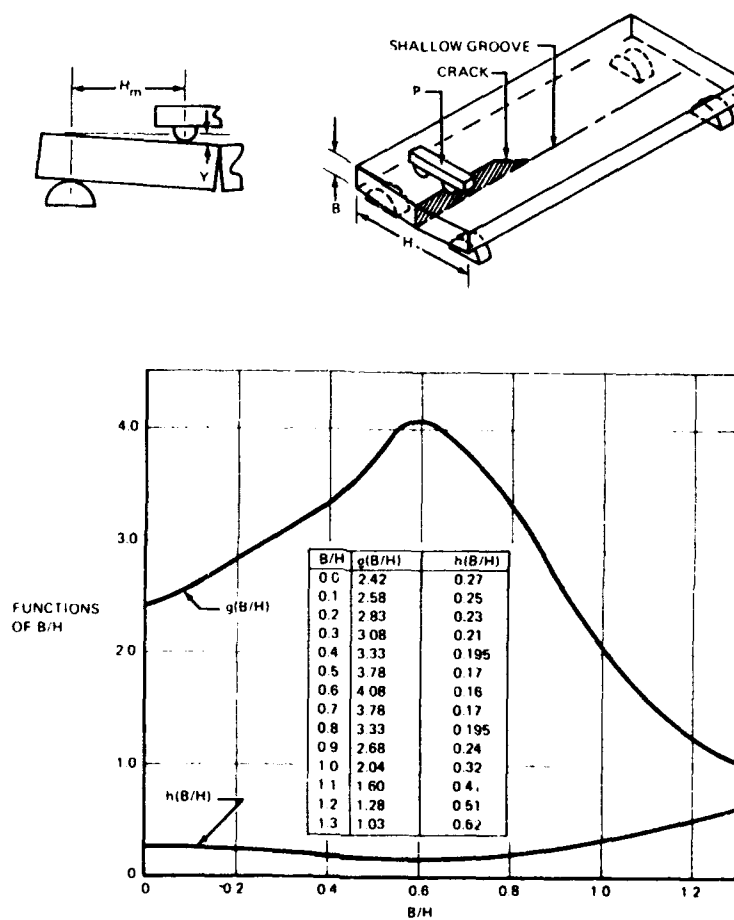
Fig. 13. Configuration and K_I calibration of the torsion-loaded, single-edge-cracked plate specimen.
