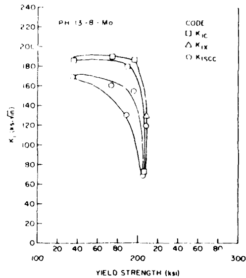
Fig. 21. Stress corrosion resistance and fracture toughness of 13Cr-8Ni-Mo PH steel [71,72,96,121].
