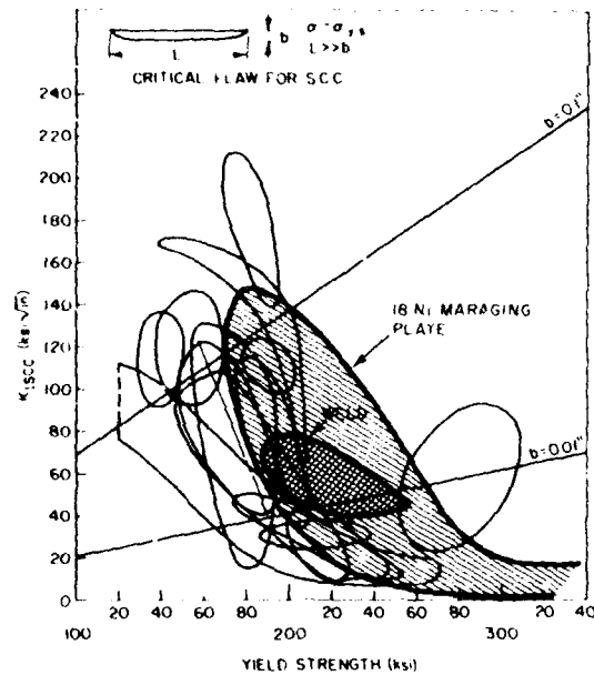
Fig. 35. Envelopes of K_{Isc} values of 18Ni maraging steel and welds (heavy lines) compared to composite of K_{Isc} envelopes for the other steels.
