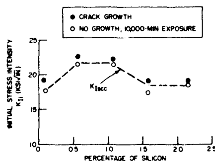
Fig. 50. Effect of silicon on threshold stress intensity K_{ISCC} (193- to 216-ksi yield strength range) (from Ref. 67). From Corrosion 25 (No. 10), 423-431 (1965); copyright by the National Association of Corrosion Engineers. Used by permission.
