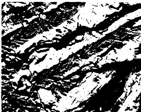
(a) Ti-6Al-4V showing cleavage of the \alpha phase [126]
