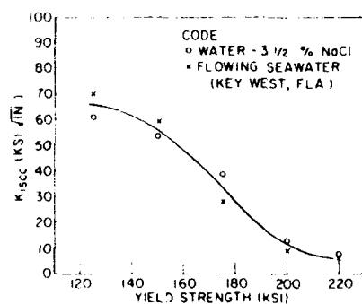
Fig. 65. Effects of quiescent distilled water containing 3½% NaCl and flowing seawater on the threshold stress intensity parameter for stress corrosion cracking of AISI 4340 steel in the 125-ksi to 220-ksi range of yield strength [156].
