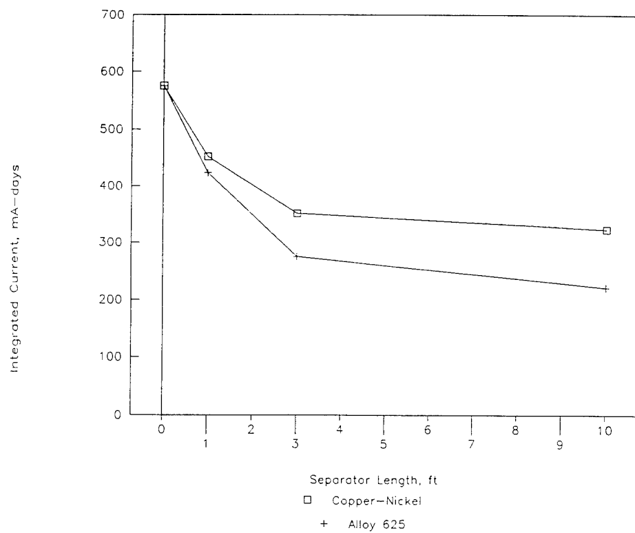
Figure 9. Effect of separator length over first 6 mo exposure (less than 1 ft/s [0.3 m/s]).
