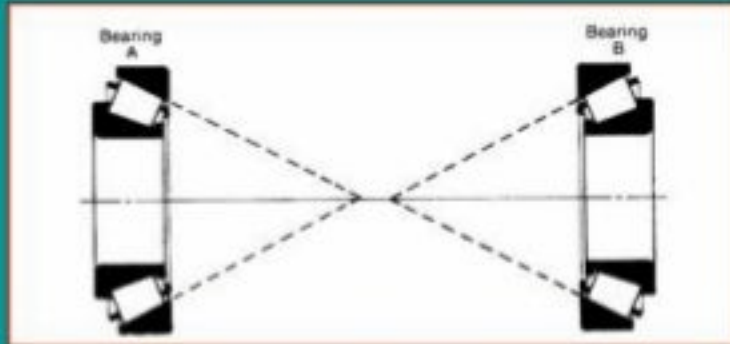
Indirect mounting
