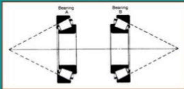
Direct mounting
