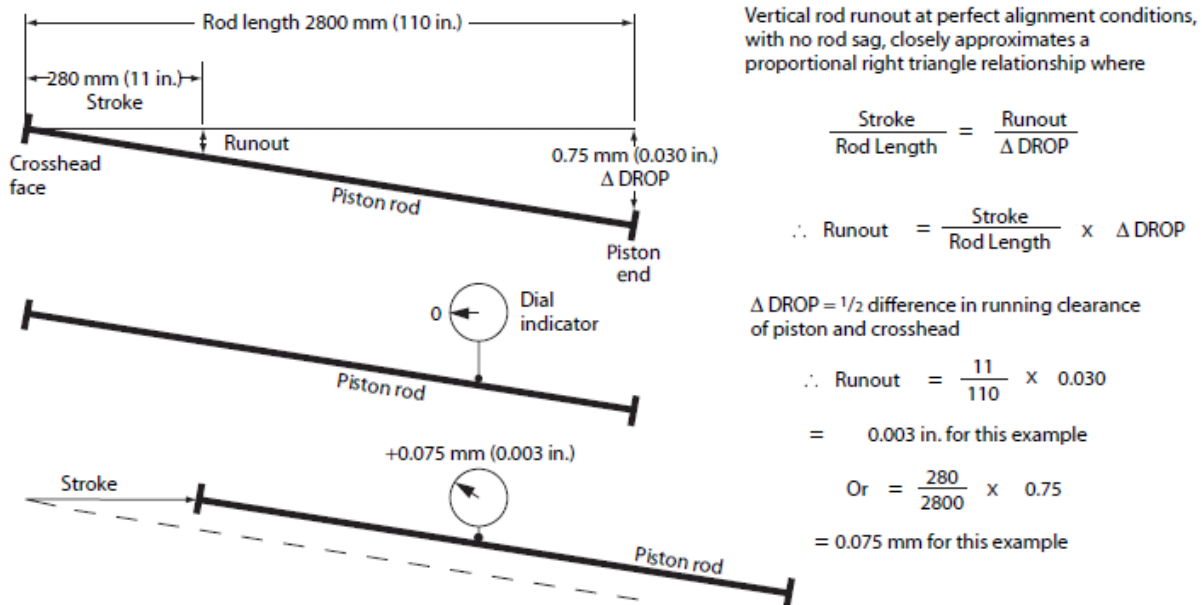
Figure C-2—Vertical Runout Geometric Relationships Based on No Rod Sag
