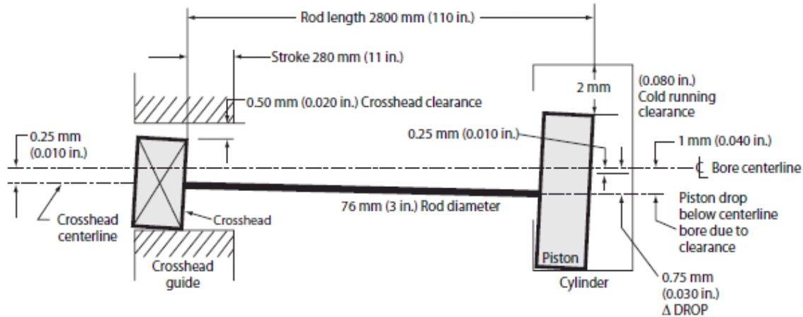
Figure C-1—Basic Geometry with Cold Vertical Runout
