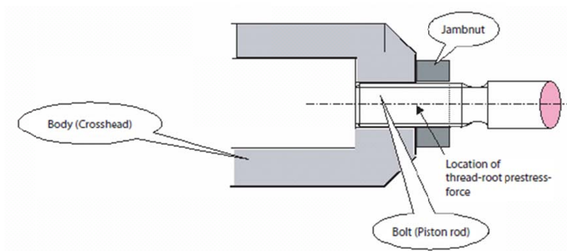
Figure F-6—Conceptual Direct Rod Connection
