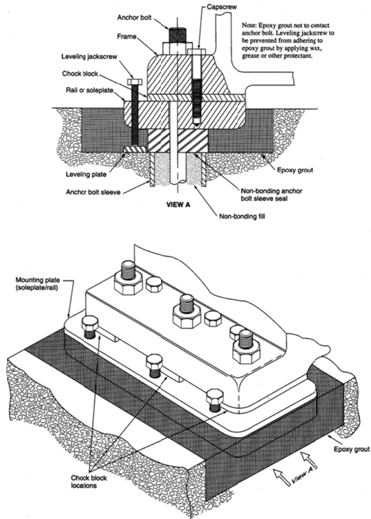
Figure K-1—Typical Mounting Plate Arrangement
