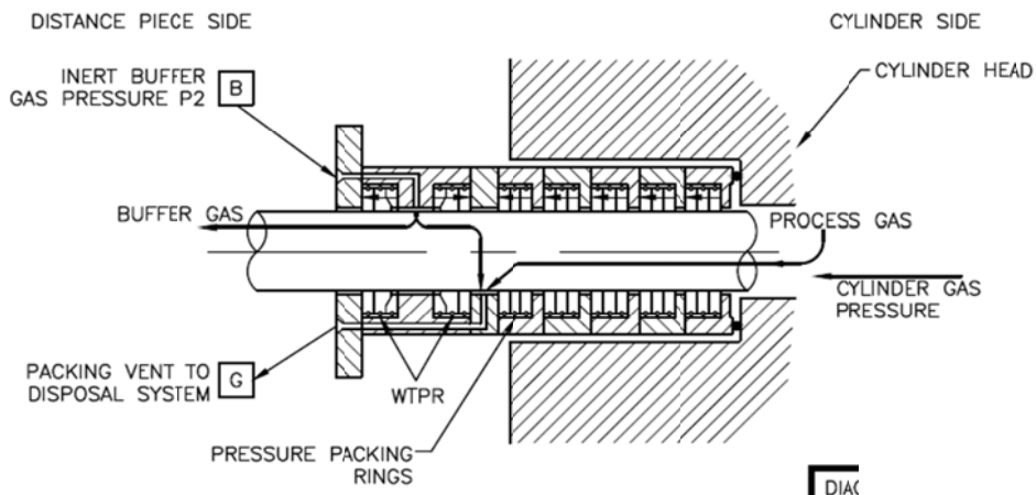
Figure H-3—Typical Purged Packing Arrangements
