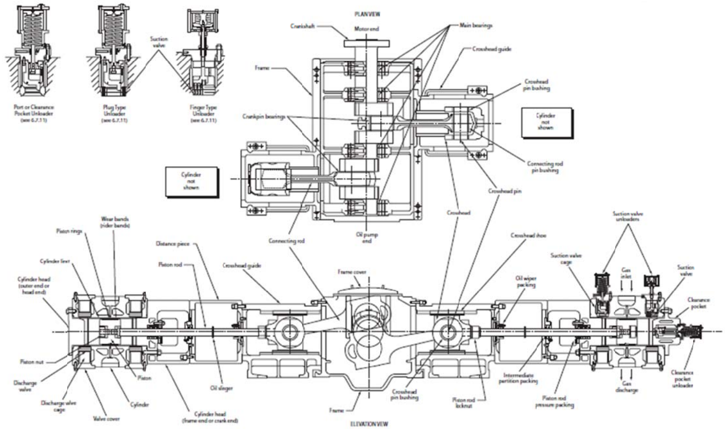
Figure I-1—Reciprocating Compressor Nomenclature
