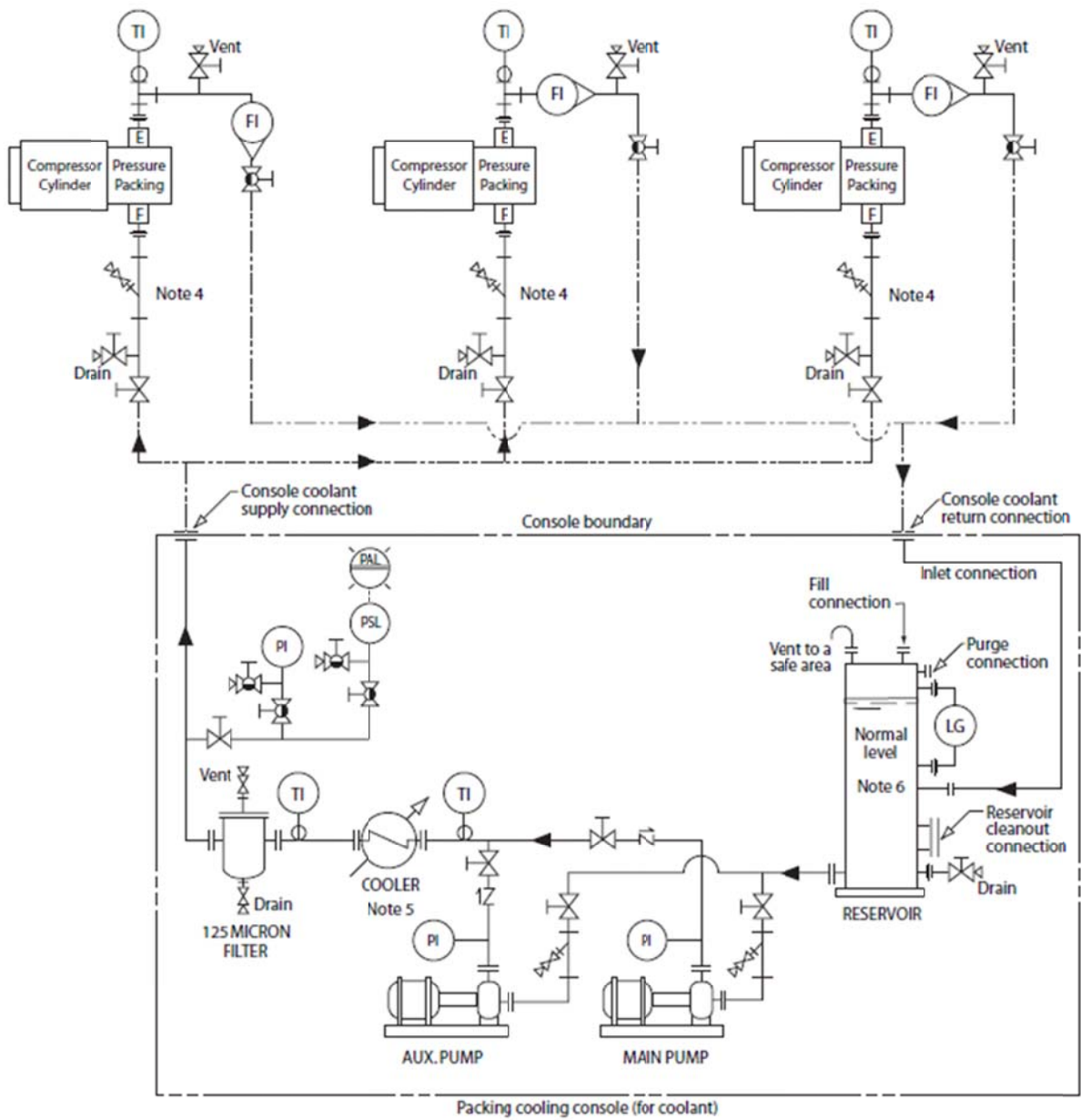
Figure F-4—Typical Self-Contained Cooling System for Piston Rod Pressure Packing
