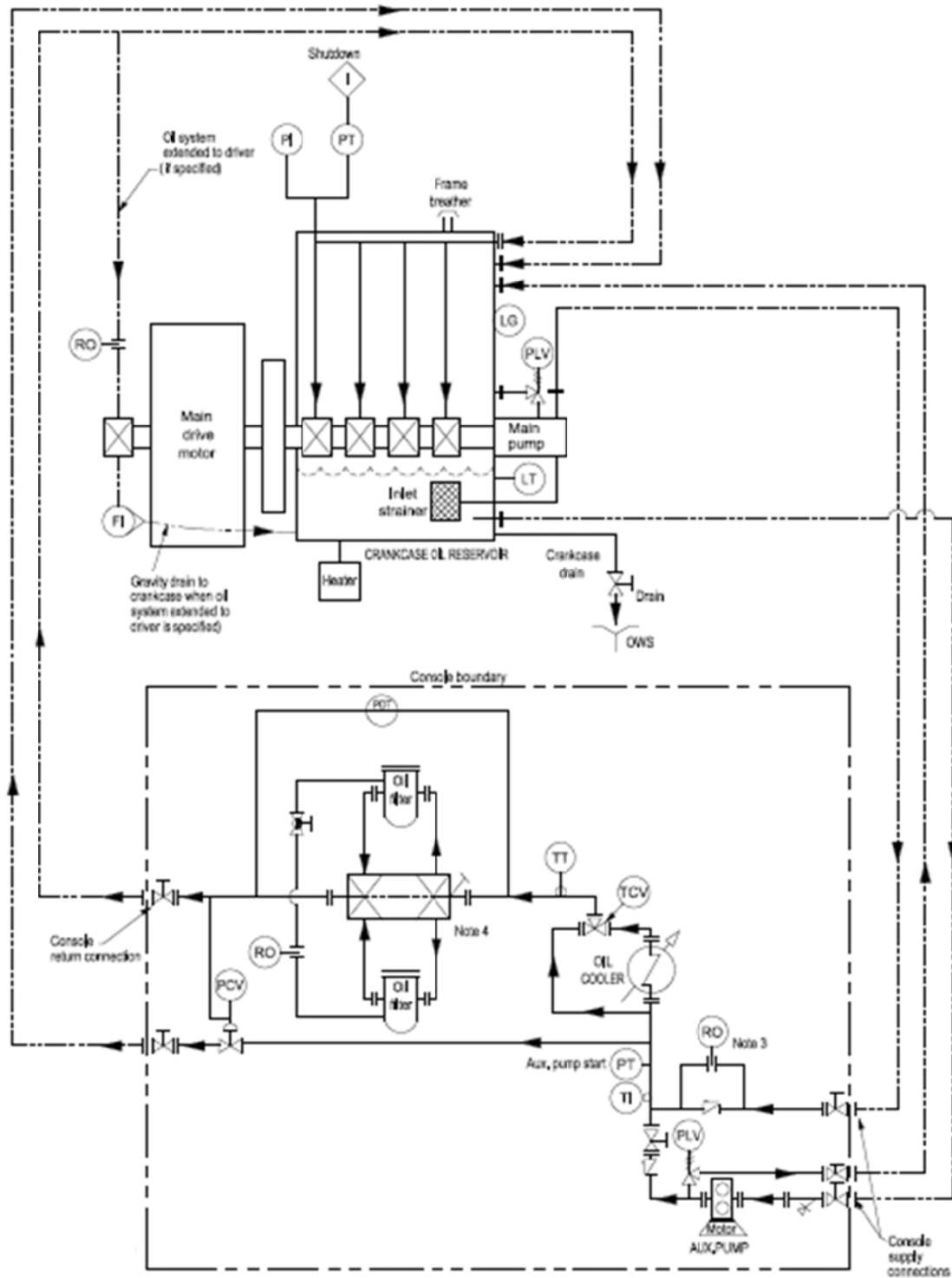
Figure F-5—Typical Pressurized Frame Lube Oil System
