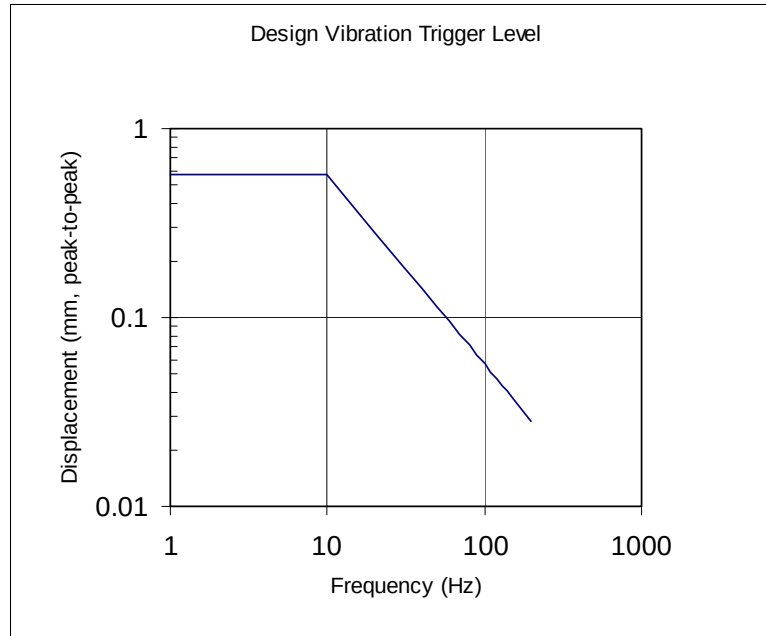
Figure 4—Piping Design Trigger Level at Discrete Frequencies
