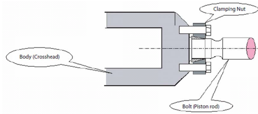
Figure F-8—Conceptual Indirect Clamped Rod Connection
