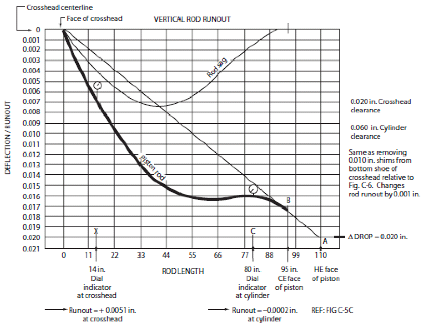
Figure C-8—Graphical Illustration of Rod Runout at 0.060 in. Cylinder Running Clearance
