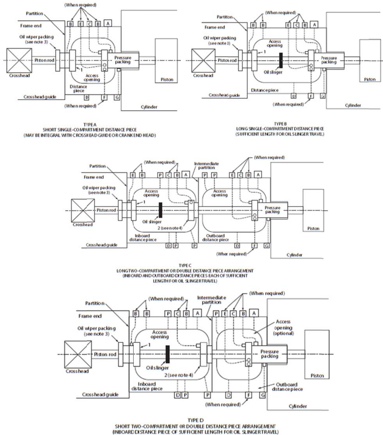
Figure F-3—Distance Piece and Packing Arrangements
