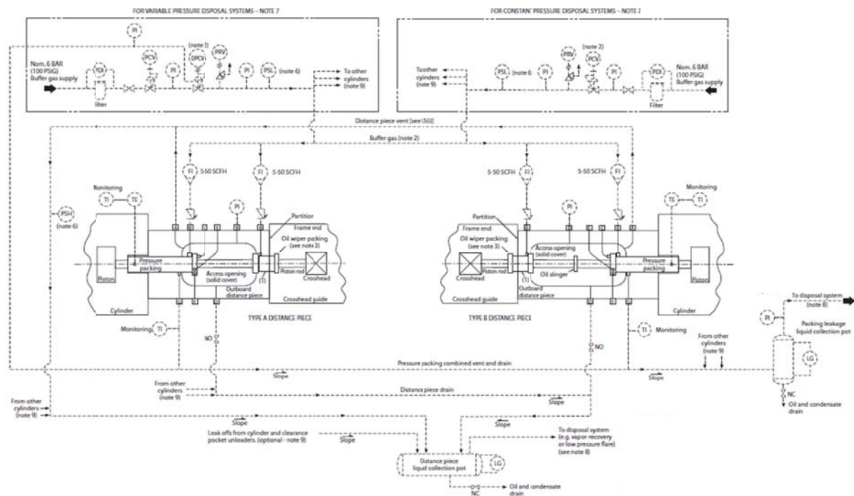
Figure H-1—Typical Buffered Single Compartment Distance Piece Vent, Drain, and Buffer Arrangement to Minimize Process Gas Leakage
