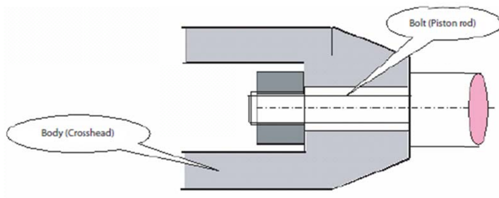
Figure F-7—Conceptual Indirect Rod Connection
