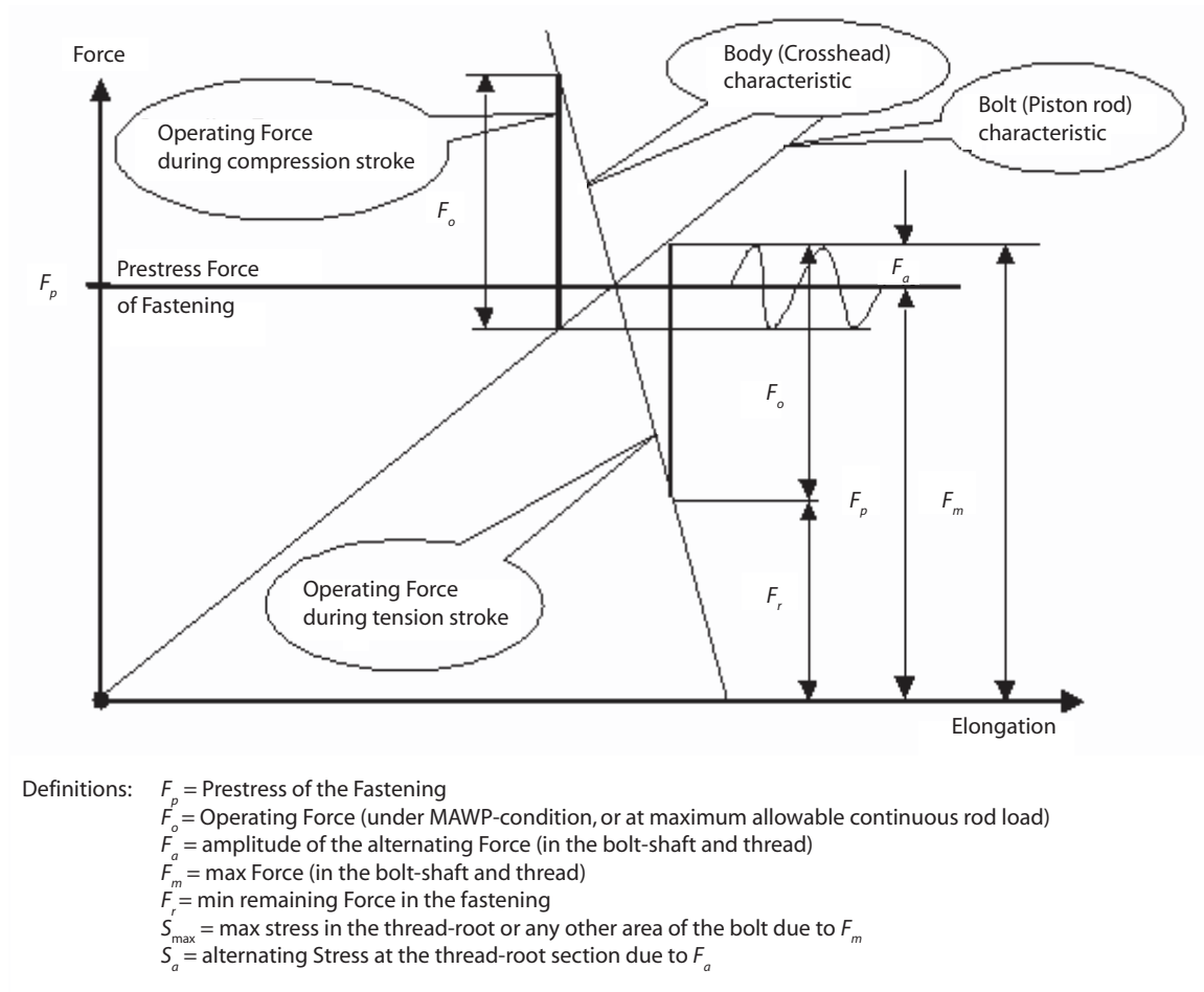
Figure G-9—Tightening Diagram (Bolt-Bracing-Diagram)
