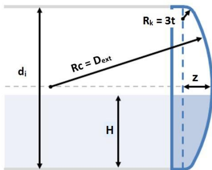
Fig 8. An horizontal tank with torispherical head [9]
