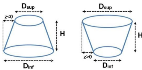
Fig 11. Conical tanks
