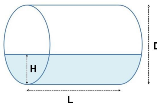
Fig 2. Horizontal cylinder
