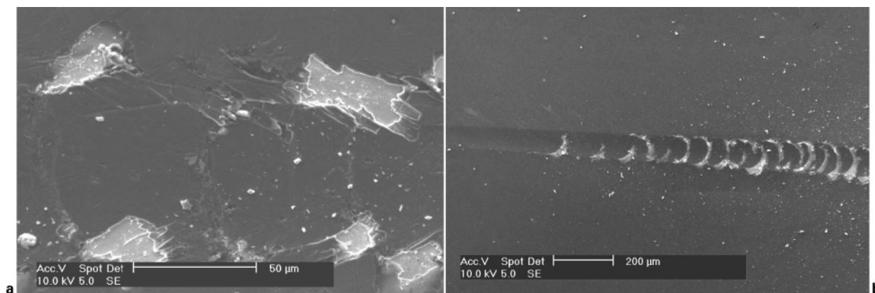
13 a forward chevron cracking in DLC coating on nitrided steel substrate (scratch direction right to left) and b wedge spallation in DLC coating on steel substrate (scratch direction left to right)
