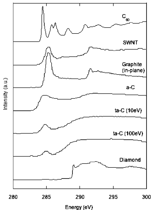
16 Schematic diagram showing intensity versus energy for different types of carbon. 26 Plots of this type can be used to determine sp^2/sp^3 bonding fractions in DLC films
