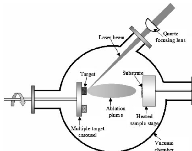
7 Schematic of pulsed laser deposition system 48
