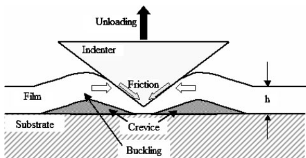
15 Schematic diagram showing cracks introduced during nanoindentation test that can be used for determining fracture toughness of DLC coatings 106
