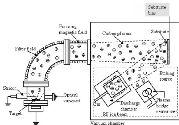
6 Schematic of FCVA 35
