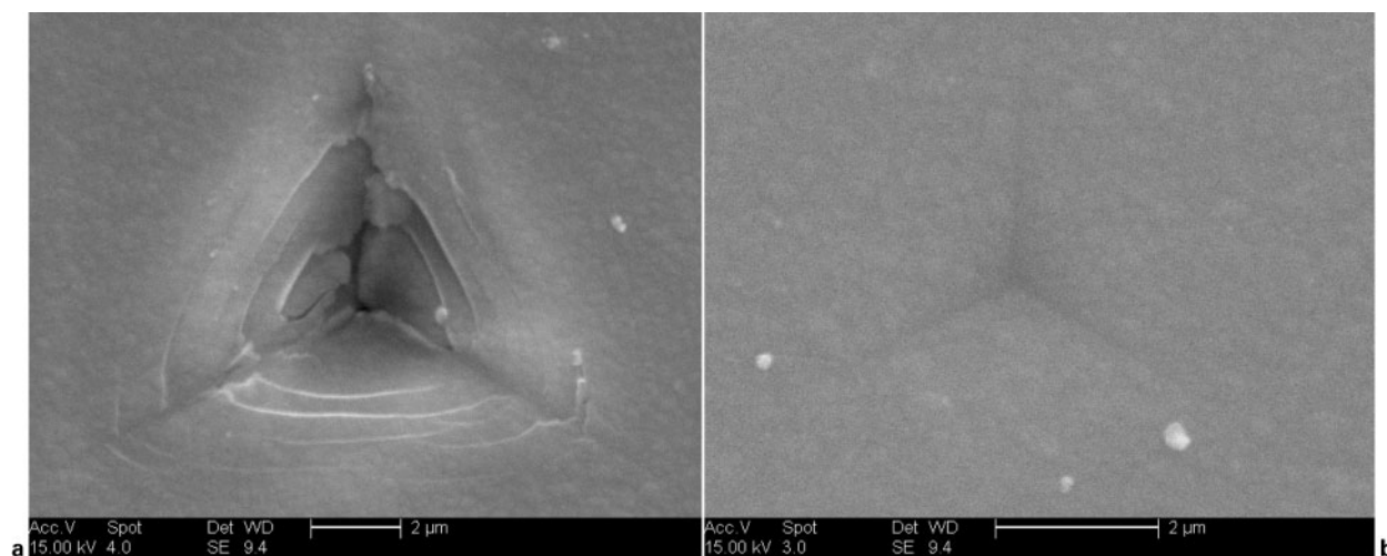
10 Images (SEM) of a 500 mN nanoindentation showing nested cracks within indentation and b 250 mN nanoindentation showing little evidence of indentation outline
