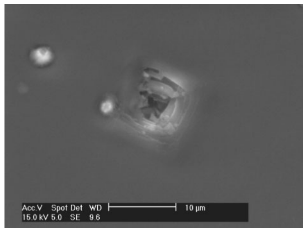
8 Nested cracks around 200 gf microindentation on DLC film. Cracking makes it difficult to accurately identify corners of indentation and leads to uncertainty in calculated microhardness values
