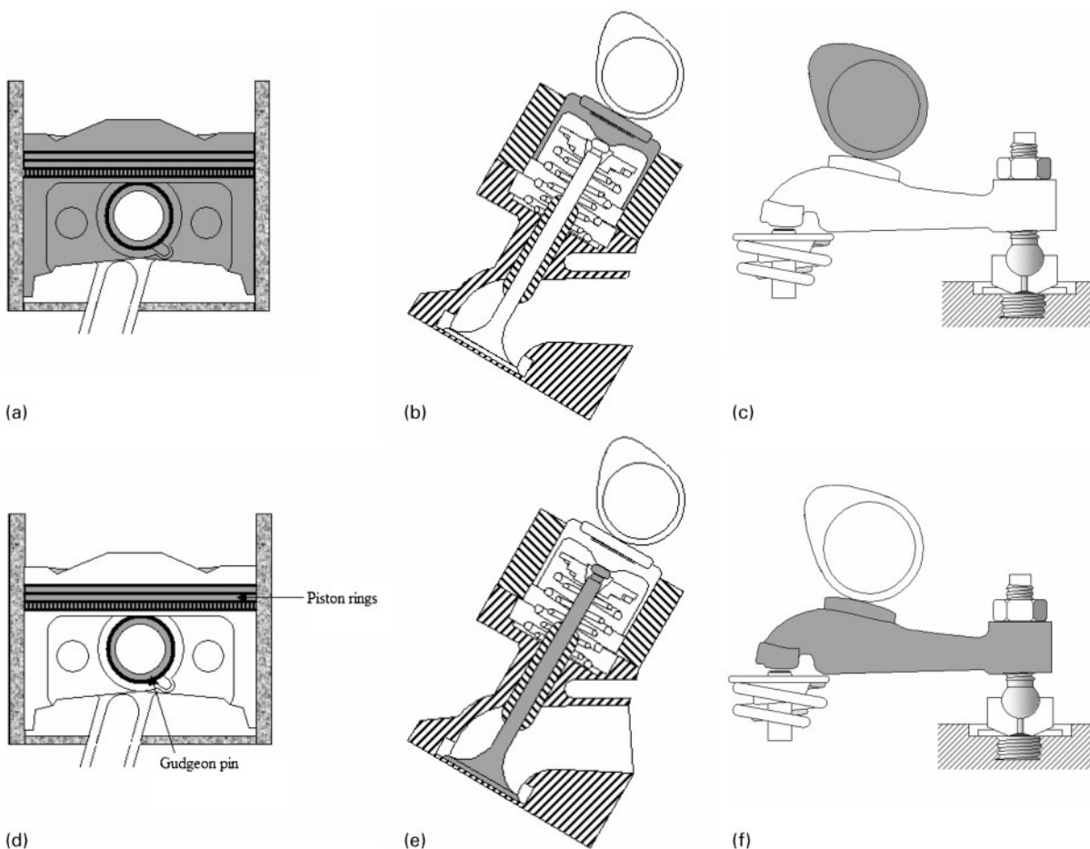
a piston; b tappet; c camshaft; d piston rings and gudgeon pin; e valve stem and head; f rocker arm 23 Components that have been successfully coated with DLC for use in automotive engine (areas in solid grey are DLC coated)
