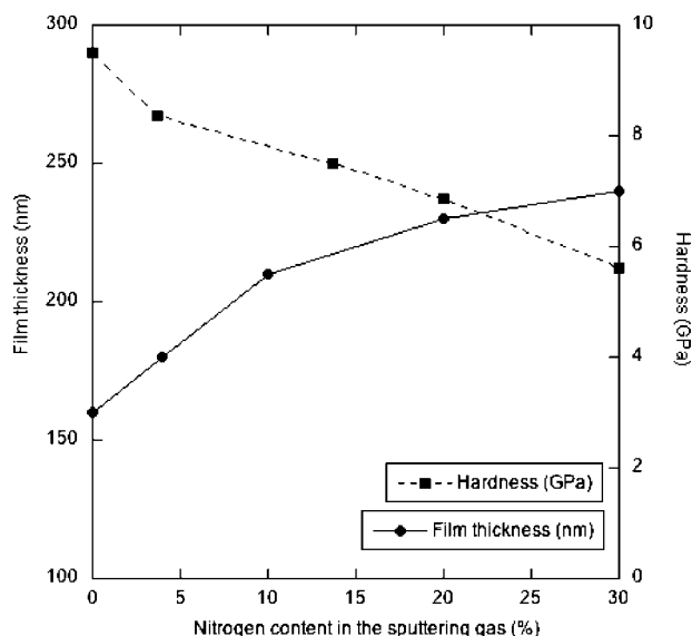
18 Film hardness and thickness as function of nitrogen content 136
