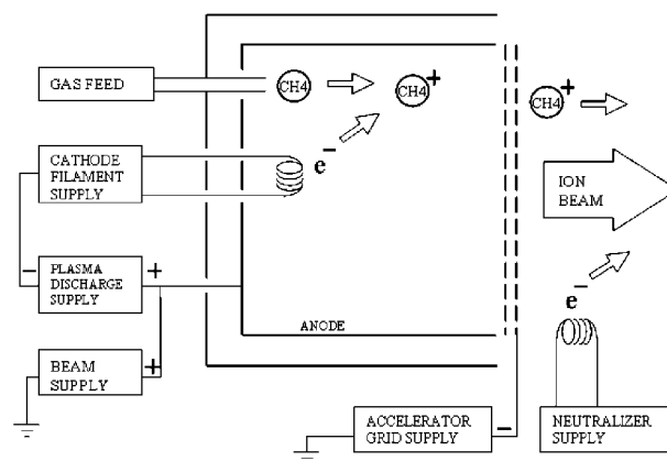
5 Schematic of ion beam deposition system 34
