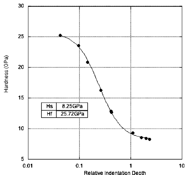
11 Hardness versus relative indentation depth for PACVD a-C:H DLC coating: data was fit by Korsunsky model 80 to extract values for substrate H_s and coating H_f hardness
