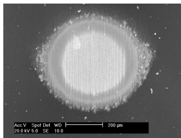
14 Micro-abrasion wear scar on a-C:H coating with TiN and SiC bond layers on steel substrate. Different layers are clearly revealed and micro-abrasion wear testing can be used to measure layer thicknesses and wear rate of differing layers
