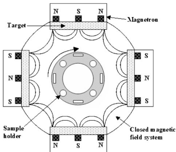
4 Schematic of closed field unbalanced magnetron sputtering ion plating system 30
