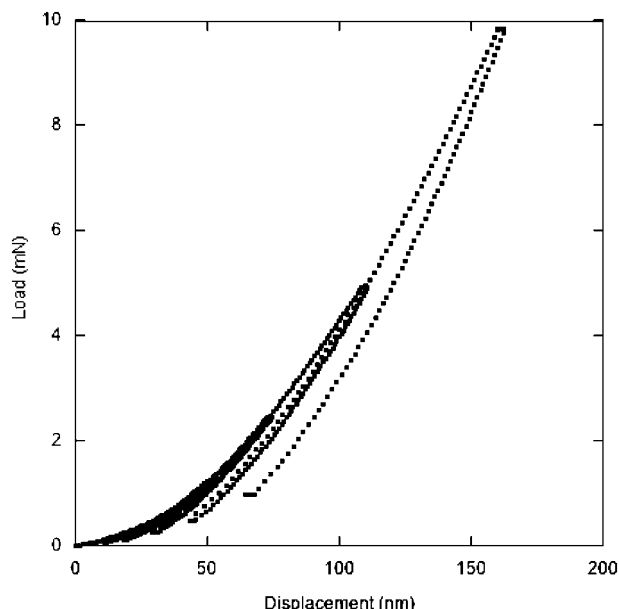
9 Typical nanoindentation load displacement curve for 10 mN indentation in PACVD a-C:H coating. Graph shows five load-unload cycles at different proportions of maximum load (10 mN) which show that coating loads in repeatable manner with no viscoelastic deformation. Hardness and modulus can be calculated from each load-unload cycle
