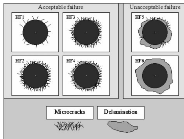
12 Schematic showing acceptable and unacceptable failure morphologies around Rockwell indentations for VDI 3198 adhesion test. Acceptable failures indicate good level of adhesion between coating and substrate 82
