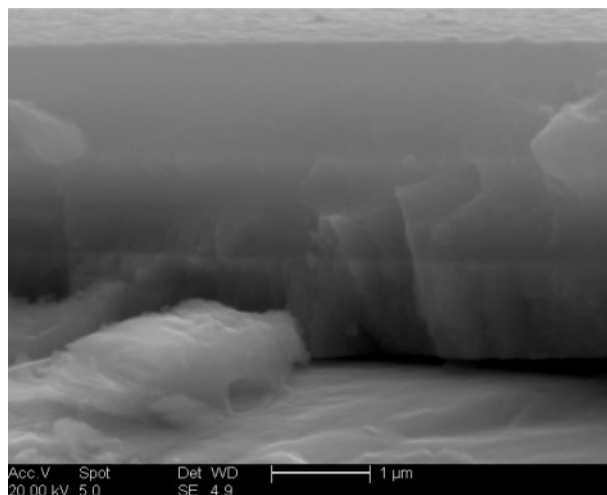
19 Cross-section through a-C:H coating that clearly reveals three different layers, a-C:H topcoat, SiC inter-layer and TiN layer for promoting adhesion to steel substrate
