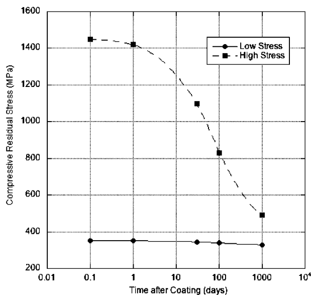
21 Effect of exposure time on measured residual stress for 1 μm thick DLC films on silicon deposited by IBAD at AEA Technology using process parameters designed to generate low and high residual stresses 189
