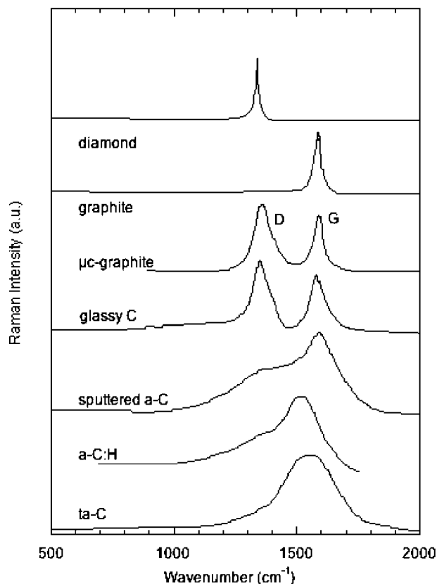
17 Typical Raman plot for different types of carbon. 26 Plots of this type can be used to determine sp^2/sp^3 fractions. Magnitude of peak shift can also be used to determine residual stress levels in film
