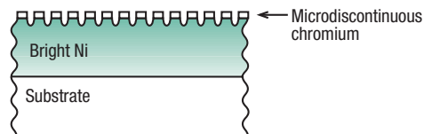
Corrosion of Nickel/Chromium Coatings Bright nickel plus microdiscontinuous chromium
