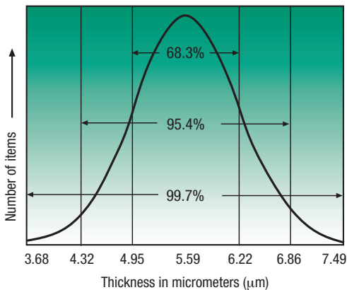
Figure 13 Probable frequency distribution in a barrel load plated to a batch thickness of 5 \mu\text{m}
