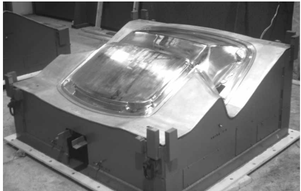
Figure 10 Electroformed nickel mould for reinforced plastic automotive body component
