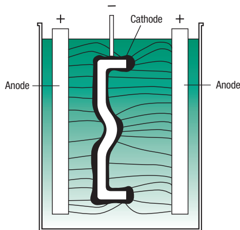
Figure 2 Thickness variation resulting from non-uniform current distribution
