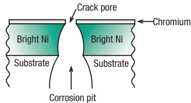
Corrosion of Nickel/Chromium Coatings Bright nickel plus regular chromium
