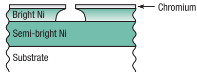
Corrosion of Nickel/Chromium Coatings Dual layer nickel plus regular chromium
