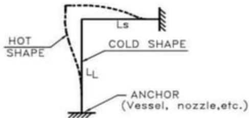
FIGURE 13 – SIMPLE PIPING SYSTEM
