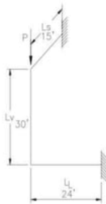
FIGURE 12B – SECTION B
