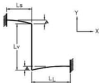
FIGURE 11 – VERTICAL PIPING
