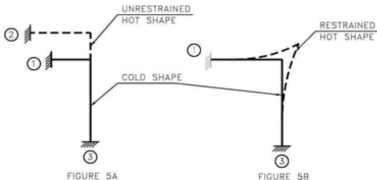
FIGURE 5 — RESTRAINED PIPING SYSTEM
