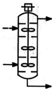
Multistage stirred column
