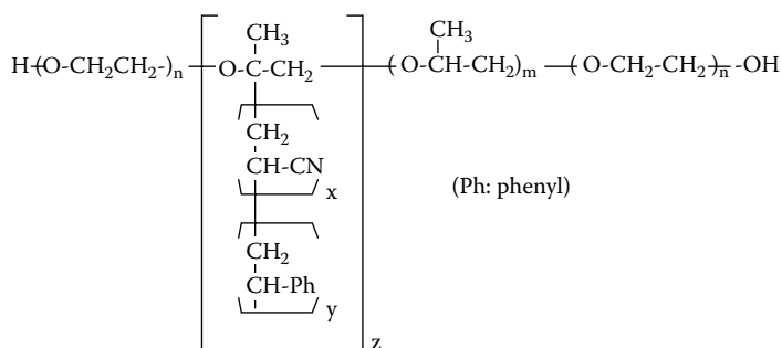
Figure 3.1 Graft Polyols.
