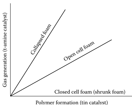
Figure 3.11 Concept of Open Cell Formation, [3.172].
