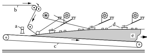
Figure 4.6 Henecke-Planibloc Process, [4.7].
