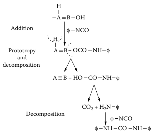
Figure 3.3 Mechanism of \text{CO}_2 Generation from Enolizable Compounds, [3.172].
