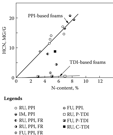
Figure 5.36 % Nitrogen in Foams vs. Amount of HCN Generation, [5.86].
