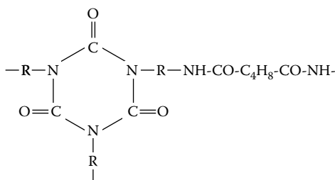
Figure 5.13 Amide-Modified PIR foam, [5.23].
