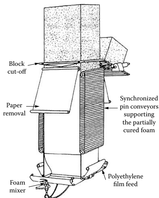
Figure 4.7 Verifoam Process, [4.103].
