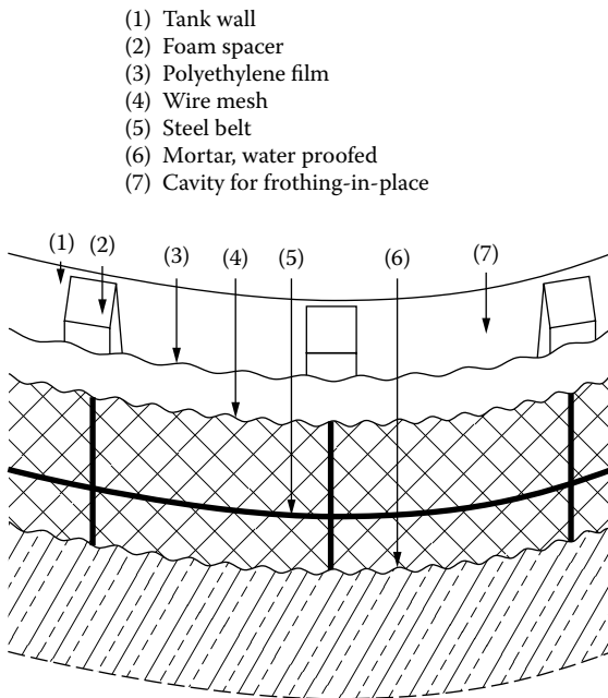
Figure 4.13(a) Frothing-in-Place into Cavity of Tank Surface [4.54].
