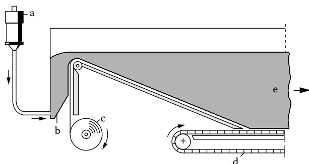
Figure 4.5 Maxifoam Process, [4.7].
