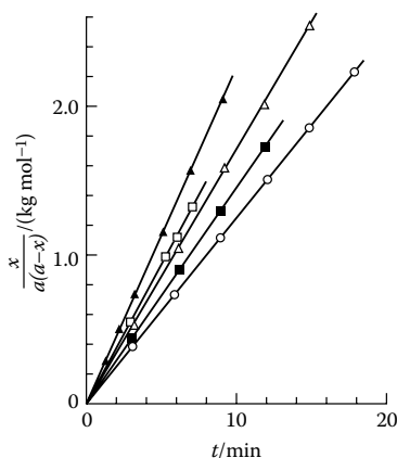
Figure 5.23 The Integral Foam of the Second Order-Time Plot for the Cyclotrimerization of Phenyl Isocyanate, [5.73].
