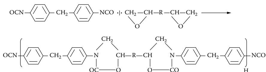
Figure 5.9 NCO-Terminated Poly-2-Oxazolidone Prepolymer [5.20].
