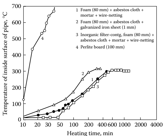
Figure 5.32 Inside Temperature of Large Fire Test, [5.44].
