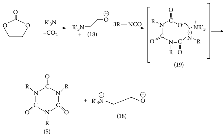
Figure 5.22d Amine-Alkylene Catalysis, [5.8].
