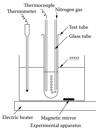
Figure 5.25 Gel Time Determination Apparatus, [5.72].
