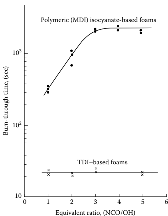
Figure 5.6 Comparison of Polyisocyanurates in Burn-Through Time, [5.11].
