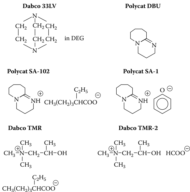
Figure 5.27 Cyclotrimerization Catalysts-2, [5.81].
