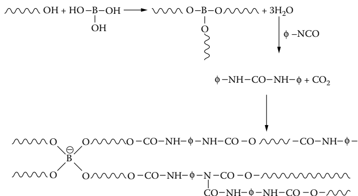
Figure 3.4 Mechanism of \text{CO}_2 Generation from Boric Acid [3.172].
