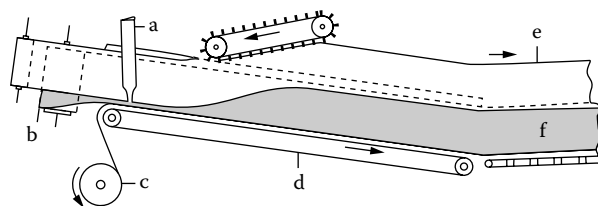
Figure 4.4 Draka-Petzetakis Process, [4.7].
