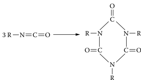
Figure 5.1 Cyclotrimerization of monoisocyanate.
