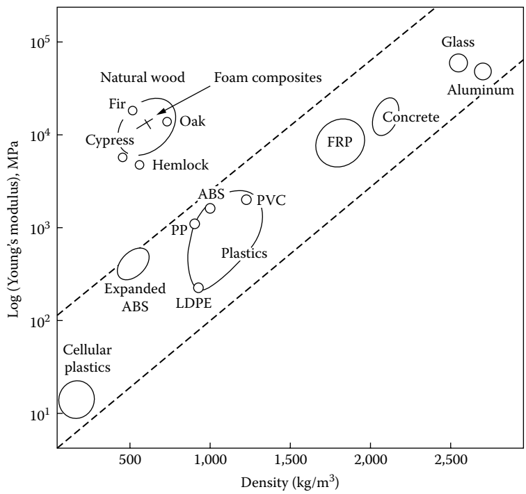
Figure 4.19 Comparison in Strength of Various Materials, [4.90].
