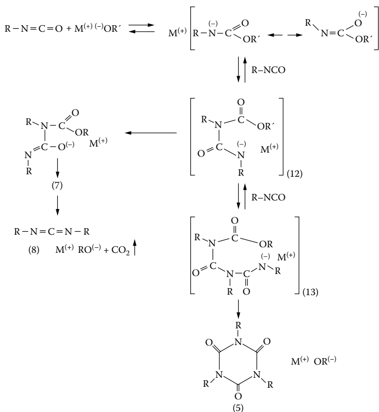
Figure 5.22b Base-Catalyzed Cyclotrimerization, [5.8].
