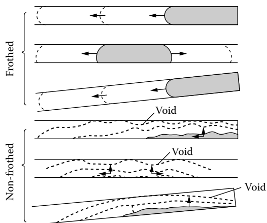
Figure 3.19 Horizontal Foaming-in-Place, [3.173].
