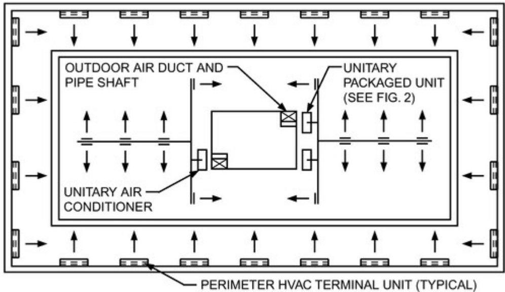
Figure 1. Multiple-Unit Systems: Single-Zone Unitary HVAC Equipment for Interior and Packaged Terminal Air Conditioners (PTACs) for Perimeter (Courtesy RDK Engineers)
