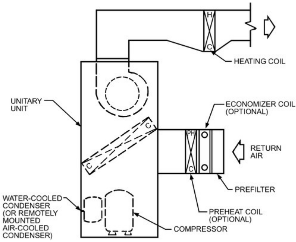
Figure 2. Vertical Self-Contained Unit (Courtesy RDK Engineers)
