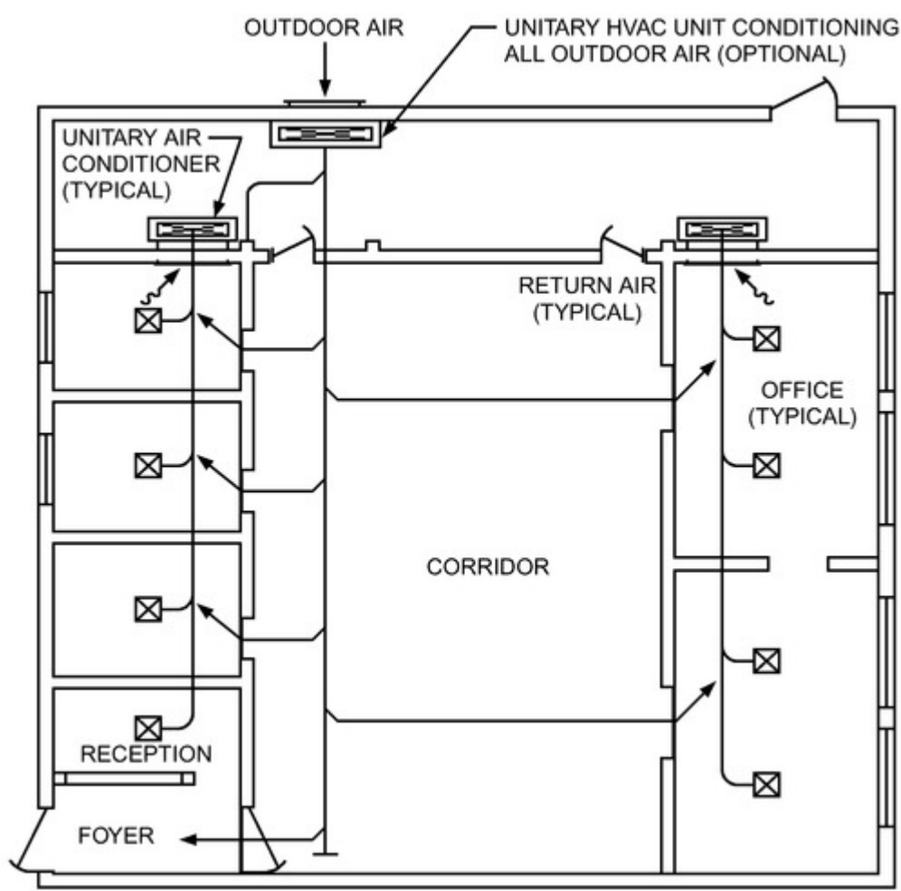
Figure 3. Dedicated Outdoor-Air-Conditioning Unit (Courtesy RDK Engineers)
