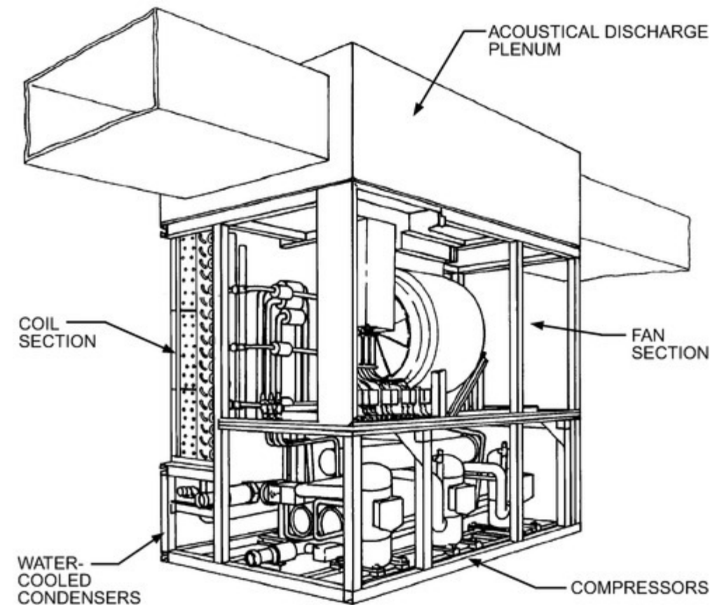
Figure 4. Commercial Self-Contained Unit with Discharge Plenum
