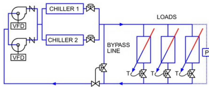
Figure 1. Primary Variable-Flow System
