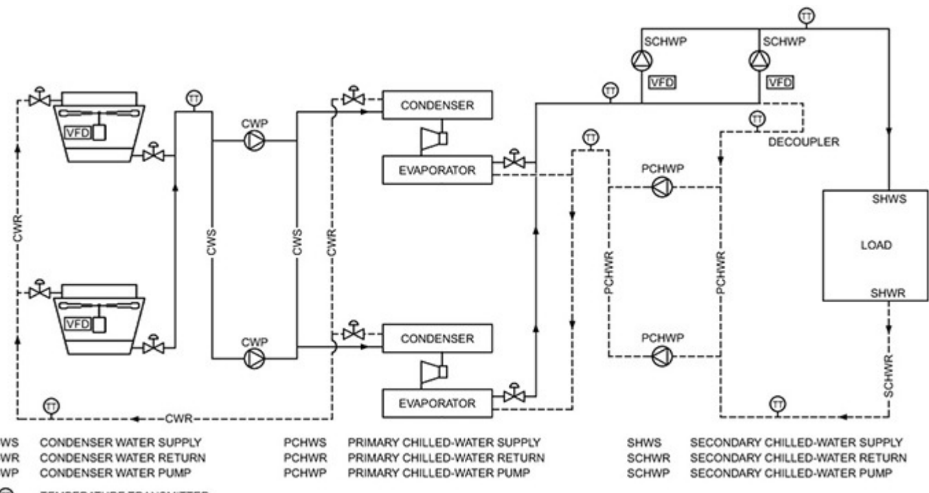
Figure 3. Primary/Secondary Pumping Chilled-Water System (Courtesy RDK Engineers)
