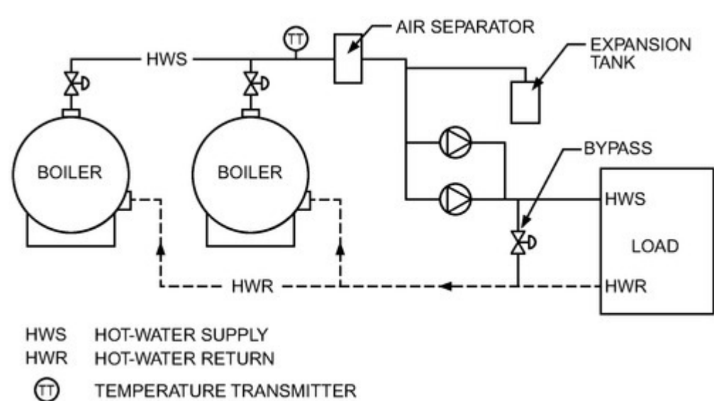
Figure 2. Primary (Limited) Variable-Flow System Using Distribution Pressure Control (Courtesy RDK Engineers)
