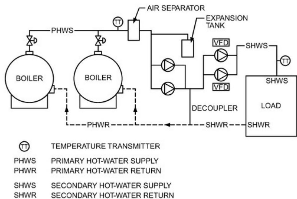
Figure 4. Primary/Secondary Pumping Hot-Water System (Courtesy RDK Engineers)
