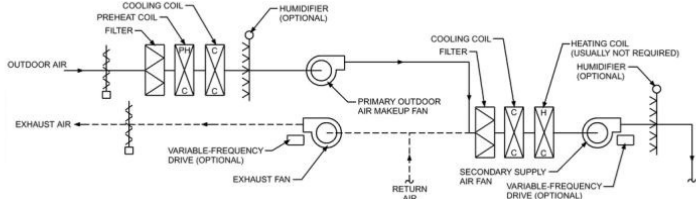
Figure 14. Primary/Secondary System (Courtesy RDX Engineers)
