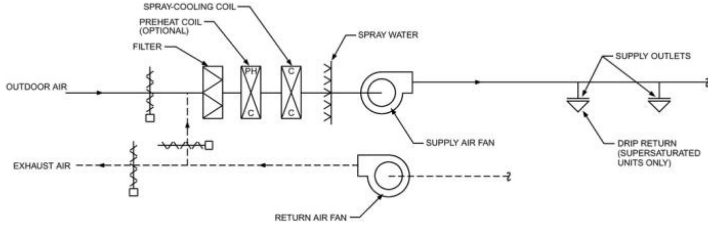
Figure 16. Supersaturated/Wetted Coil (Courtesy RDX Engineers)
