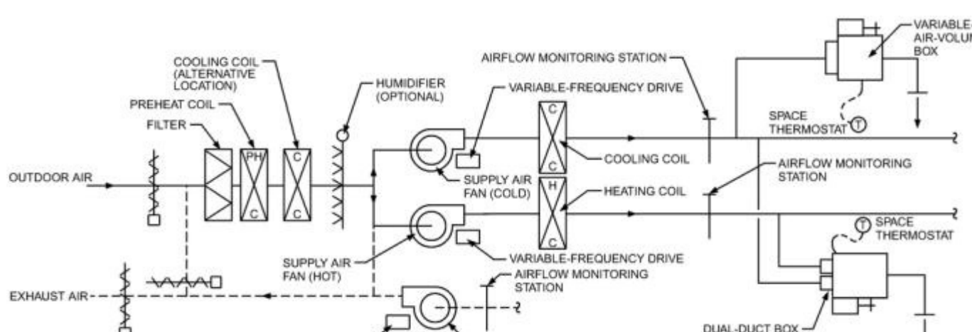
Figure 12. Dual-Fan, Dual-Duct System (Courtesy RDK Engineers)
