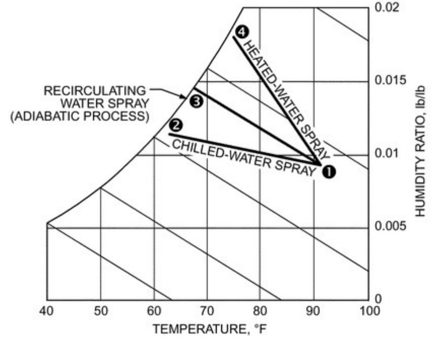
Figure 3. Direct Spray of Water in Airstream Cooling
