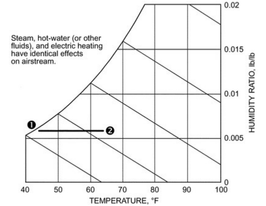
Figure 5. Steam, Hot-Water, and Electric Heating, and Direct and Indirect Gas- and Oil-Fired Heat Exchangers
