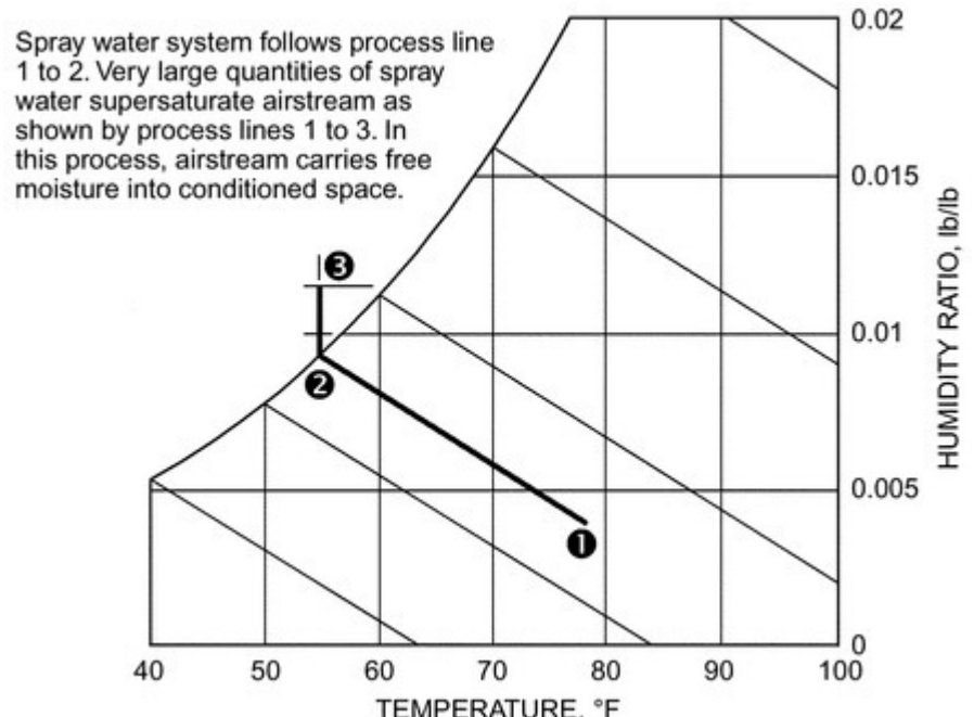
Figure 4. Supersaturated Evaporative Cooling
