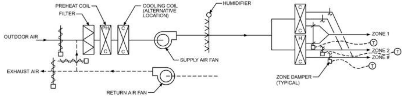
Figure 13. Multizone System (Courtesy RDX Engineers)
