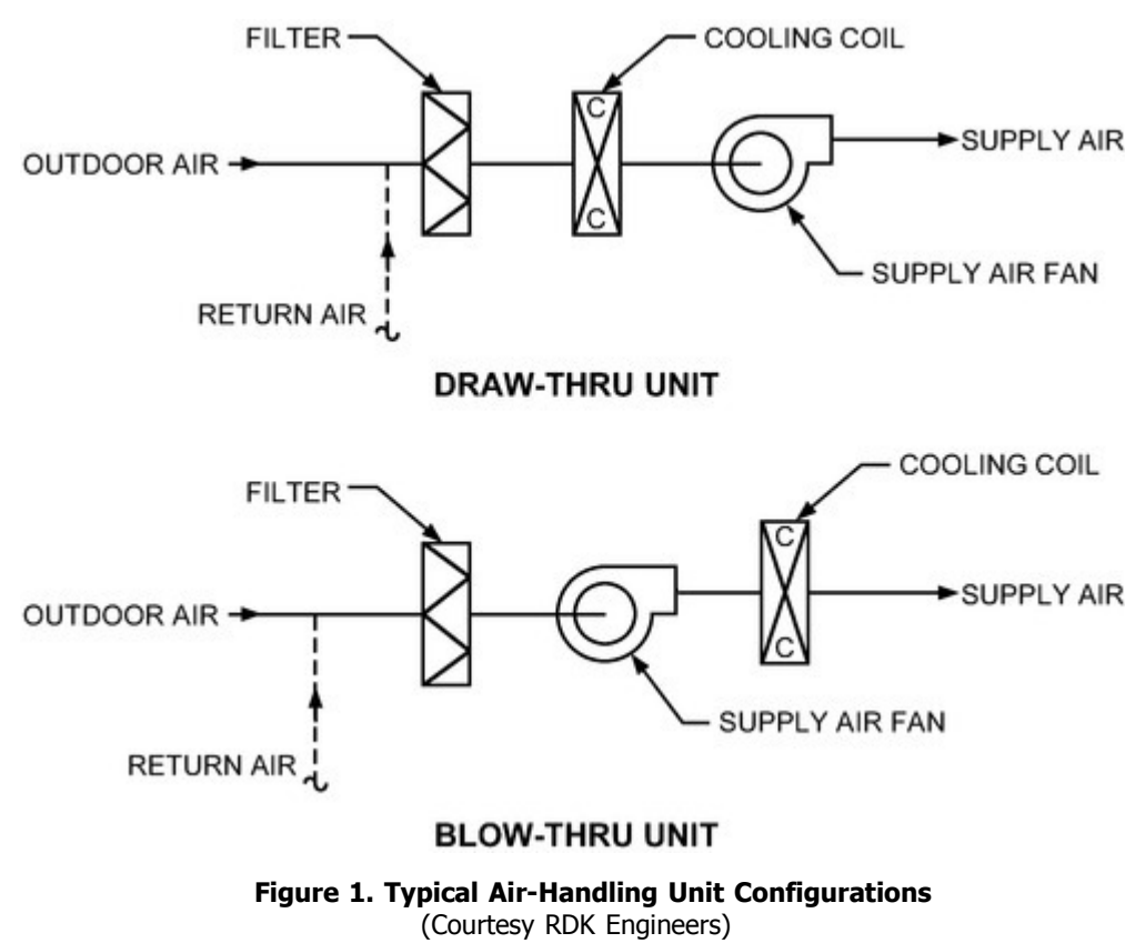
Figure 1. Typical Air-Handling Unit Configurations (Courtesy RDK Engineers)
