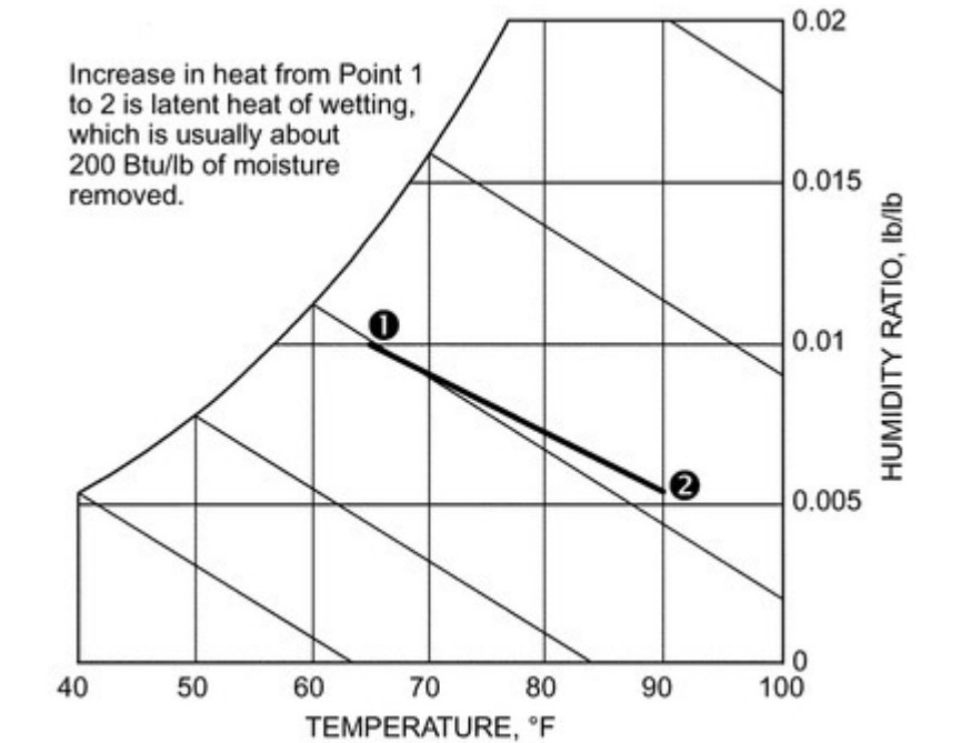
Figure 8. Chemical Dehumidification
