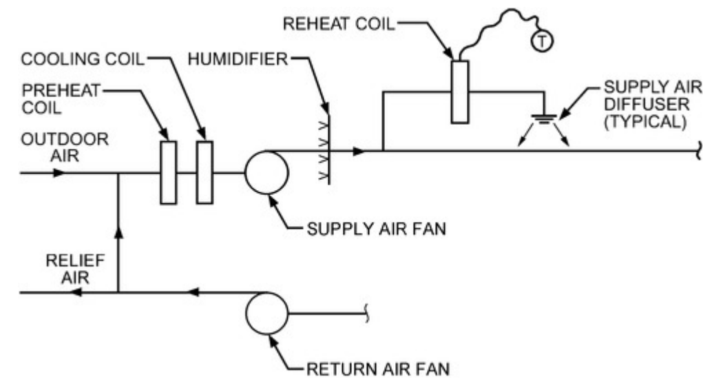
Figure 9. Constant-Volume System with Reheat (Courtesy RDK Engineers)
