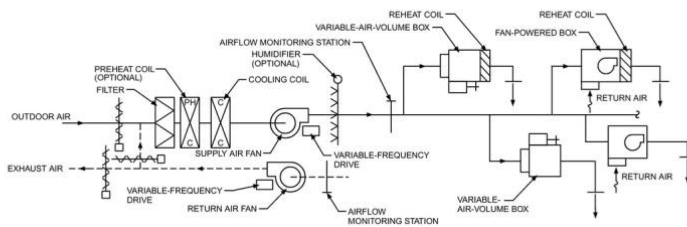
Figure 10. Variable-Air-Volume System with Reheat and Induction and Fan-Powered Devices (Courtesy RDK Engineers)
