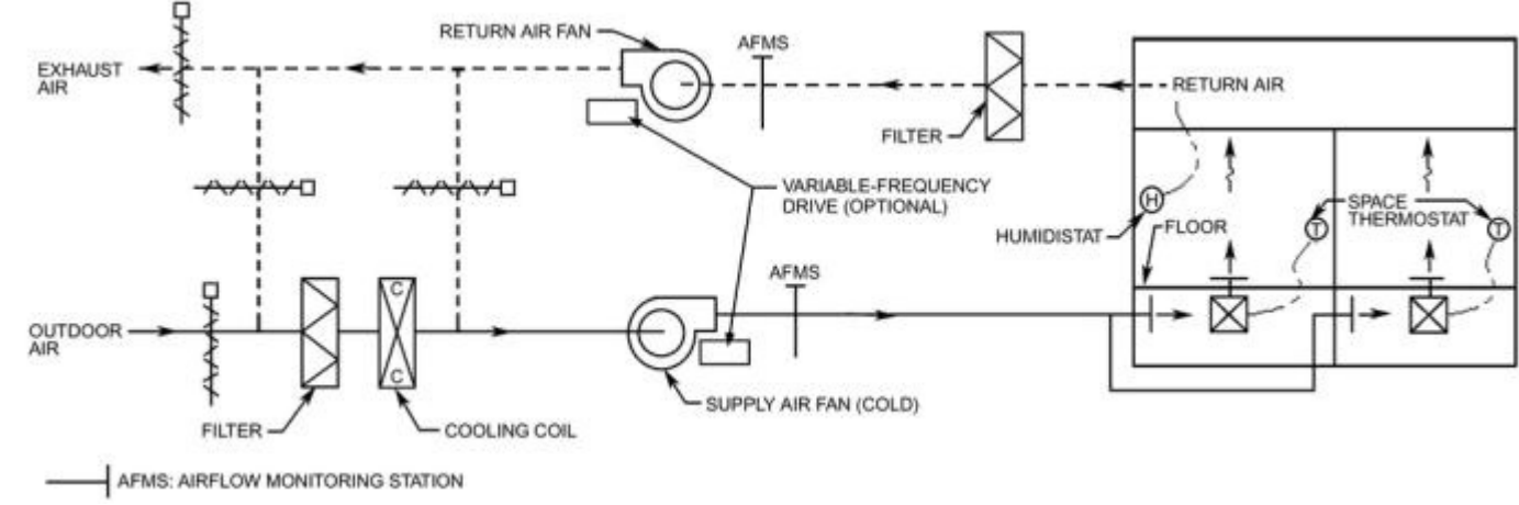
Figure 15. Underfloor Air Distribution (Courtesy RDX Engineers)
