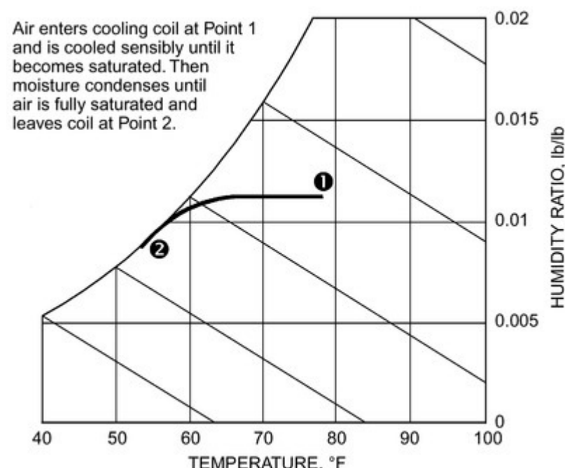
Figure 2. Direct-Expansion or Chilled-Water Cooling and Dehumidification
