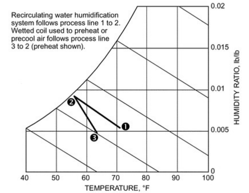
Figure 6. Direct Spray Humidification
