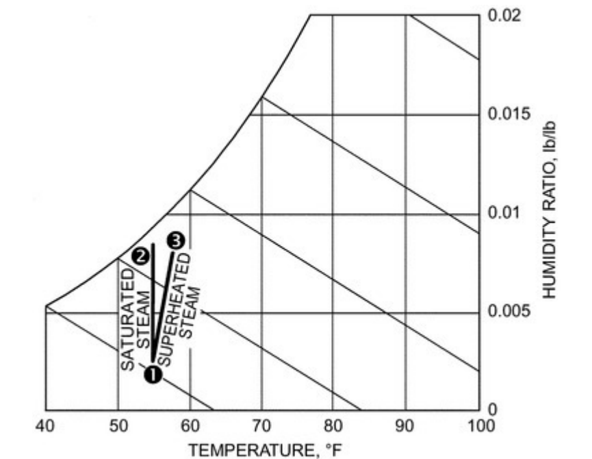
Figure 7. Steam Injection Humidification
