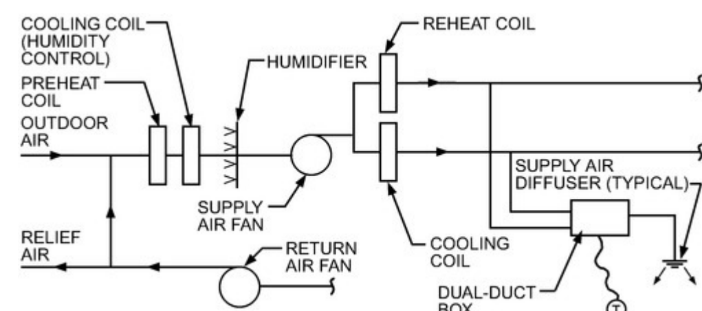
Figure 11. Single-Fan, Dual-Duct System
