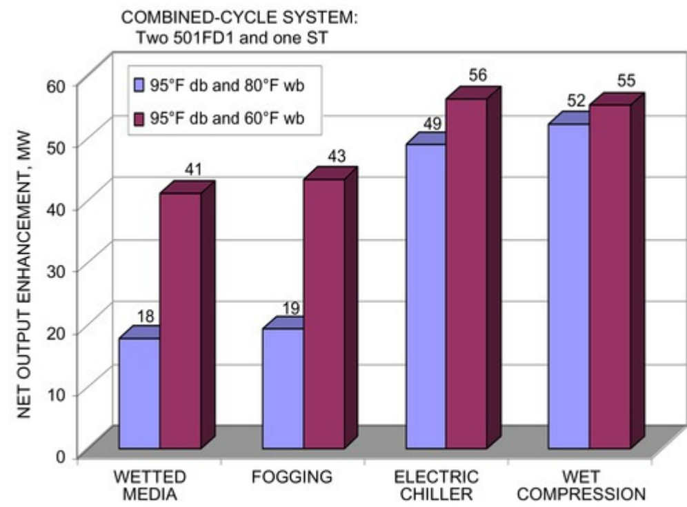
Figure 11. Examples of Effect of CTIC Technology and Ambient Condition on Capacity Enhancement Potential (TICA 2008)
