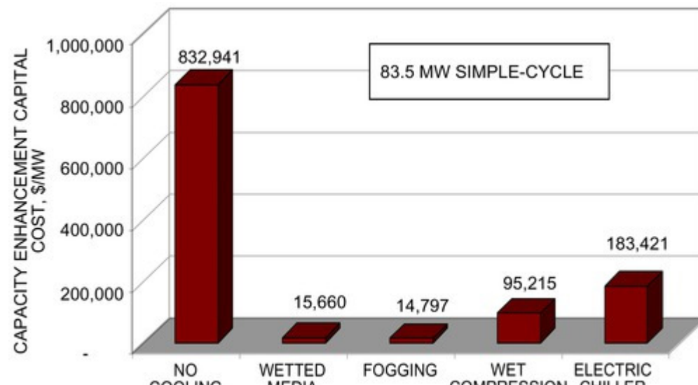
Figure 12. Example of Effects of CTIC Technology and Ambient Condition on Unitized Capital Cost of Capacity Enhancement (TICA 2008)
