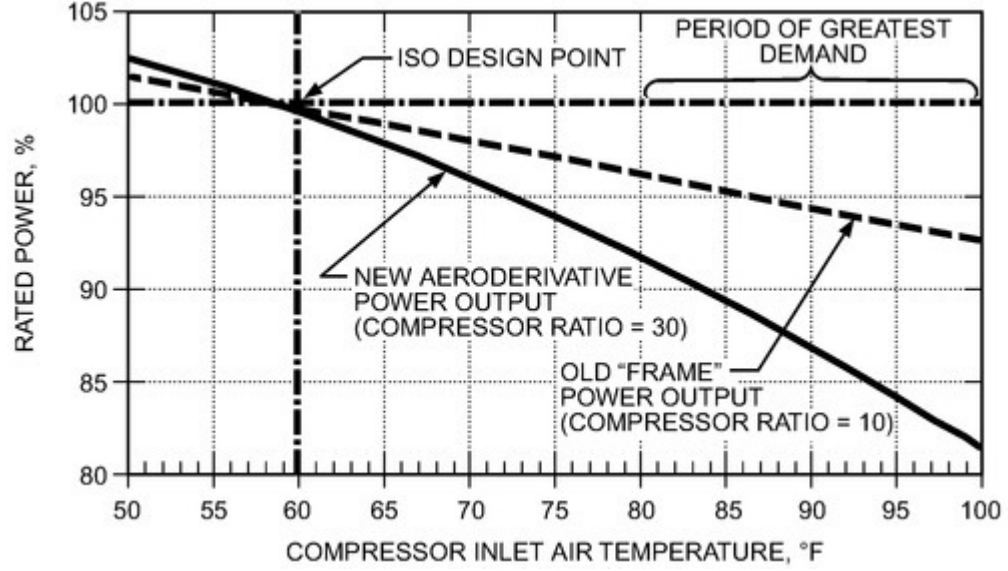
Figure 1. Effect of Ambient Temperature on CT Output (Punwani and Hurlbert 2005)
