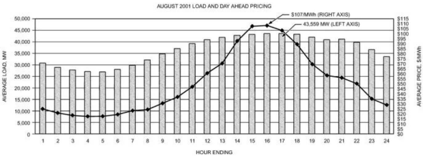
Figure 5. Example of Daily System Load and Electric Energy Pricing Profiles (Hilberg 2006)
