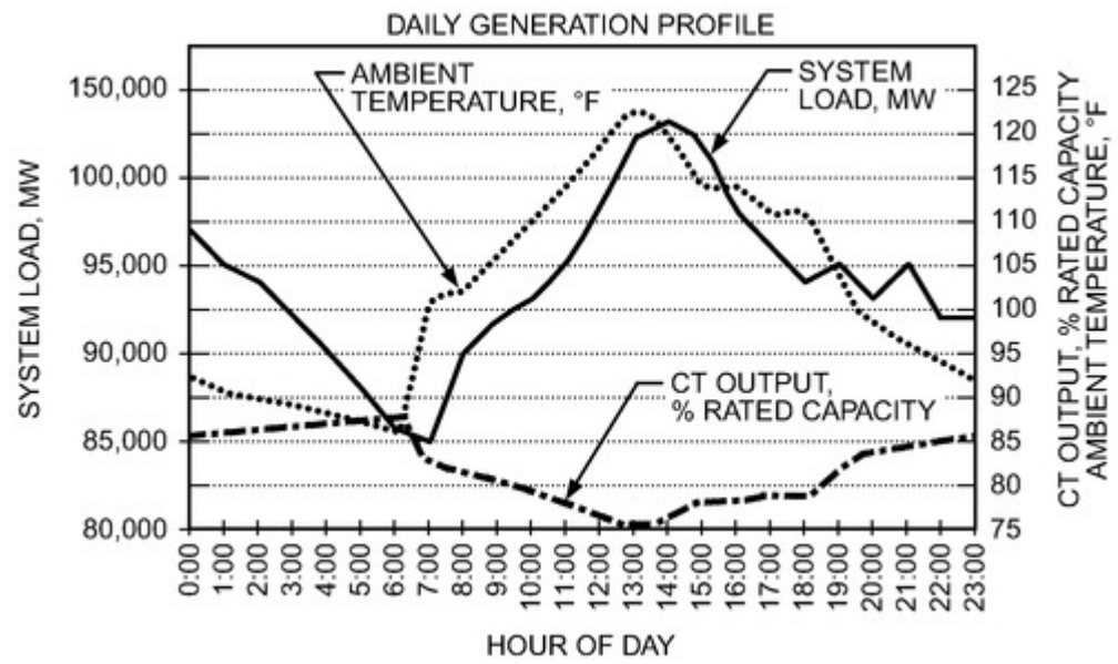
Figure 4. Typical Hourly Power Demand Profile (Punwani and Hurlbert 2005)
