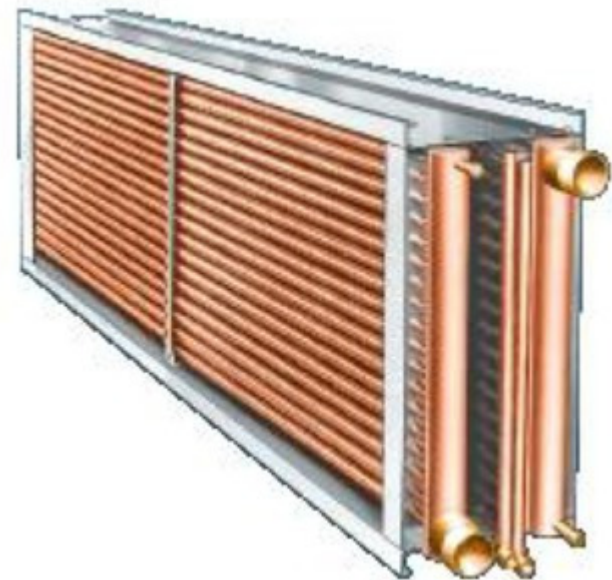
Figure 10. Cooling Coil Used for Indirect Cooling Chiller Systems (Courtesy of Aerotin)
