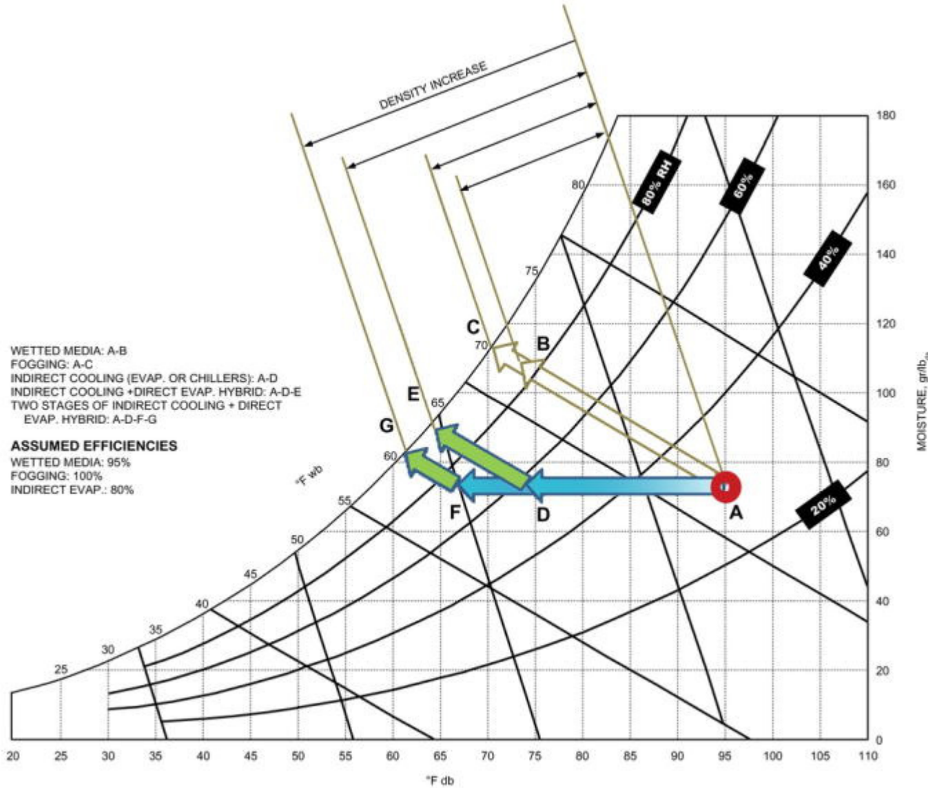
Figure 7. Psychrometric Chart Showing Direct and Indirect Inlet Air Cooling Processes (Schlom and Bastanian 2009)
