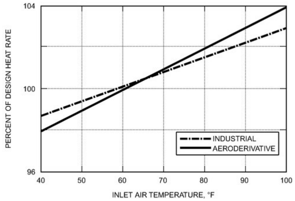
Figure 2. Effect of Ambient Temperature on CT Heat Rate (Punwani 2003)
