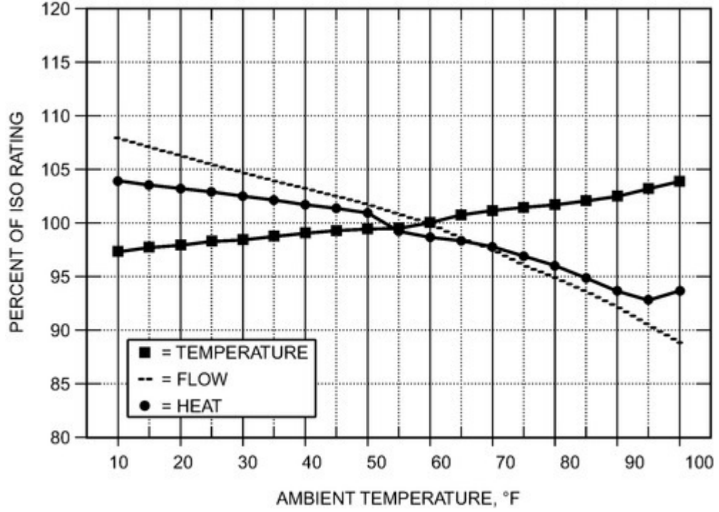
Figure 3. Effects of Ambient Temperature on Thermal Energy, Mass Flow Rate and Temperature of CT Exhaust Gases (Orlando 1996)
