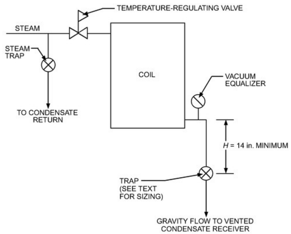
Figure 9. Trapping Temperature-Regulated Coils
