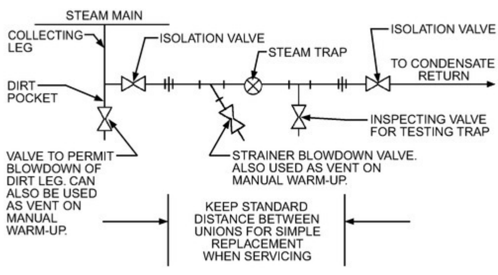
Figure 8. Recommended Steam Trap Piping
