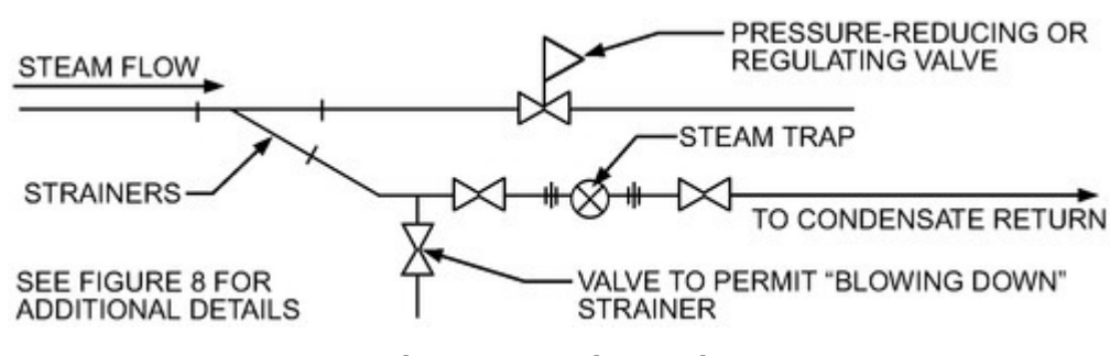
Figure 6. Trapping Strainers
