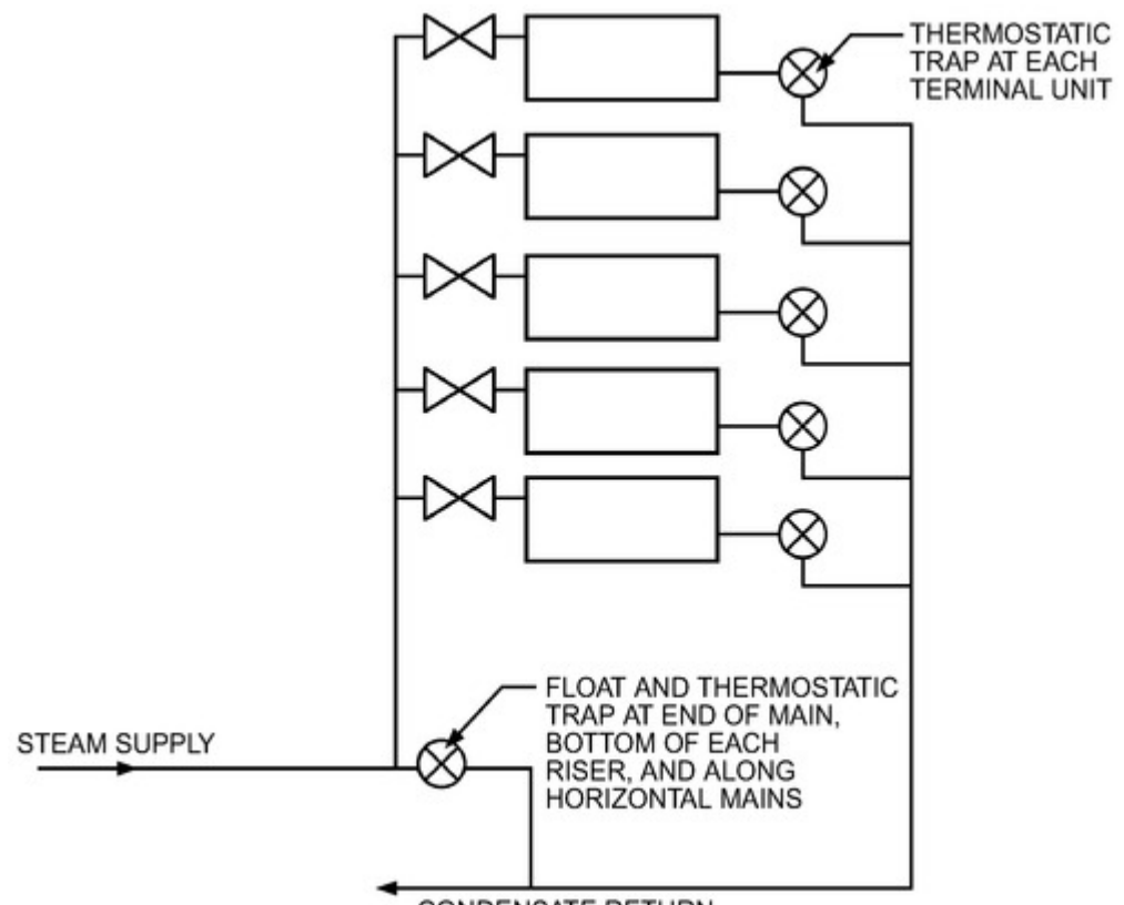
Figure 16. Two-Pipe System
