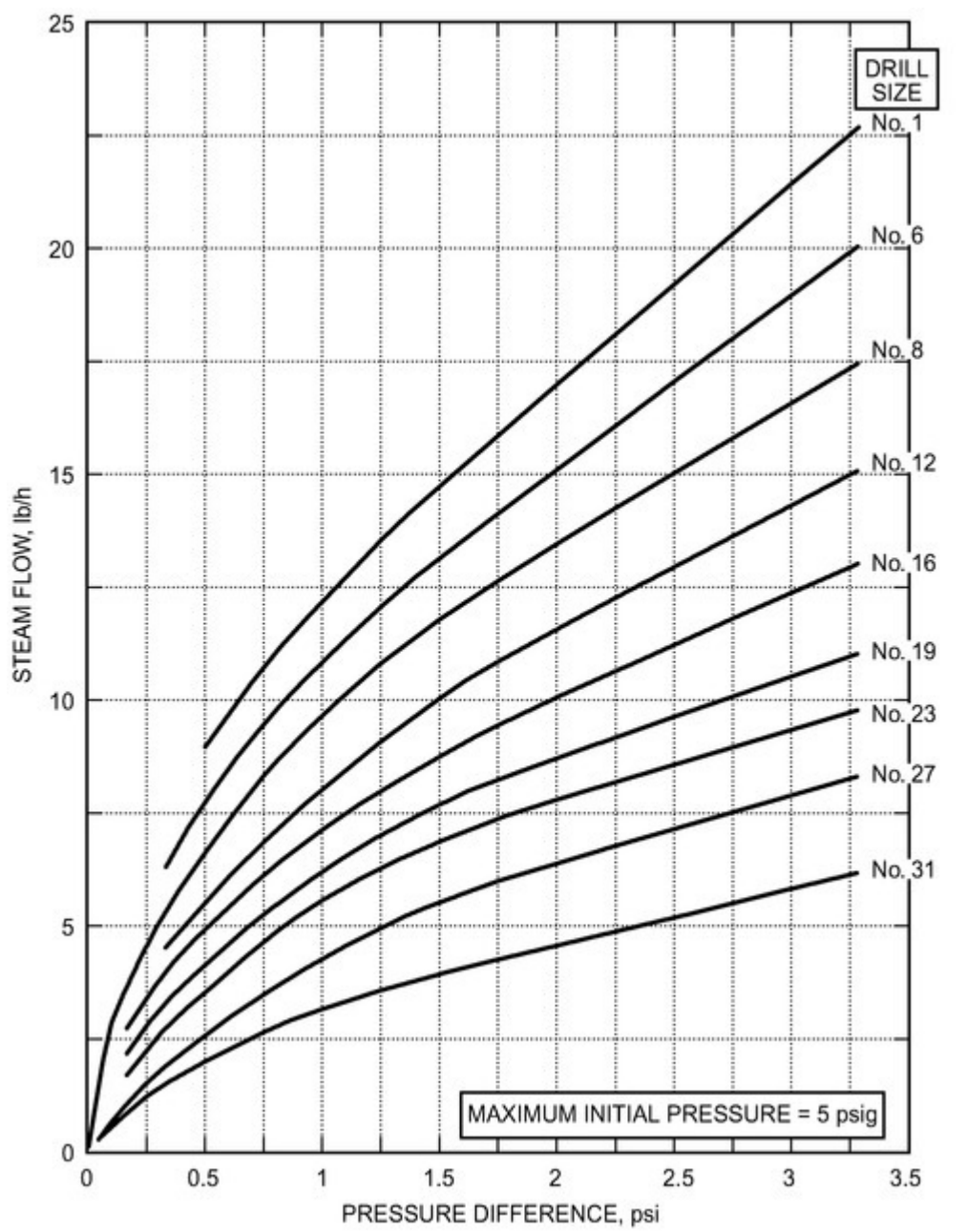
Figure 18. Orifice Capacities for Different Pressure Differentials (Schroeder 1950)
