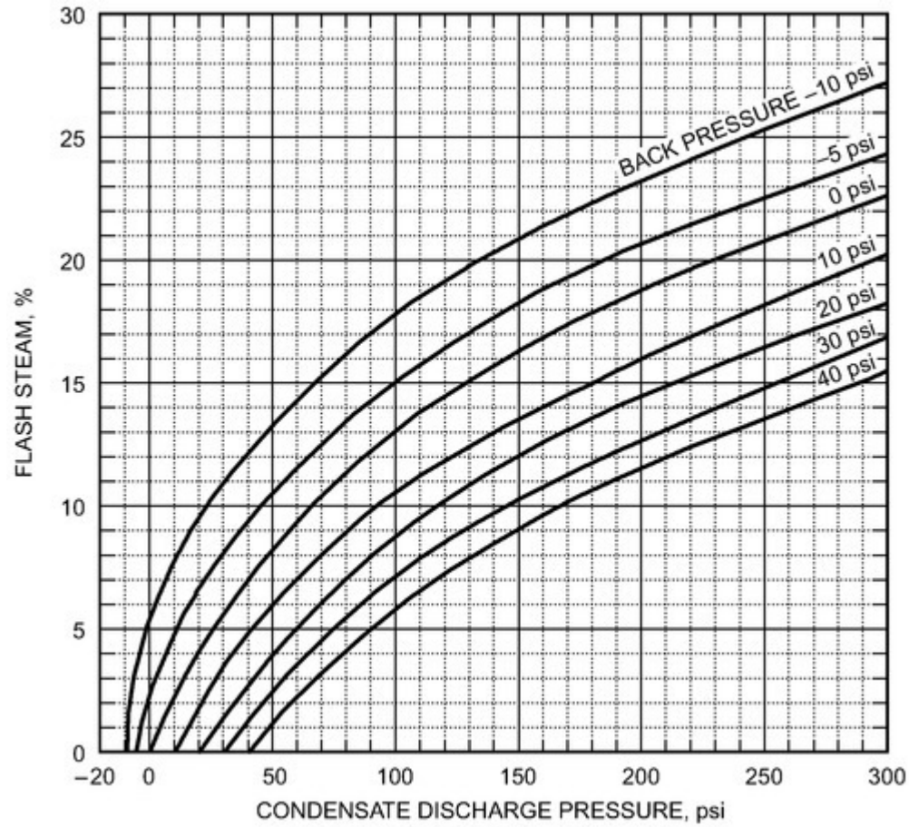
Figure 19. Flash Steam
