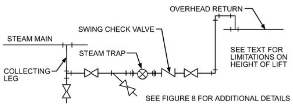
Figure 5. Trap Discharging to Overhead Return
