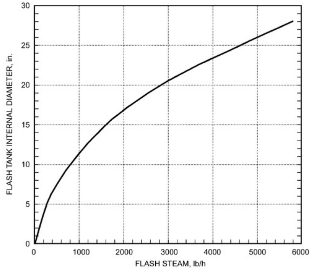
Figure 21. Flash Tank Diameter
