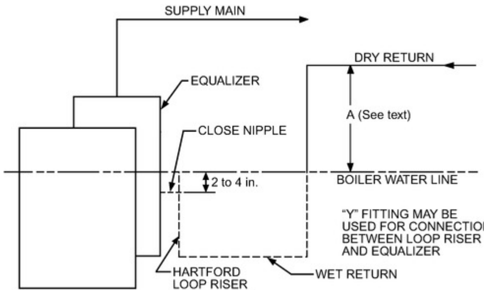
Figure 3. Boiler with Gravity Return
