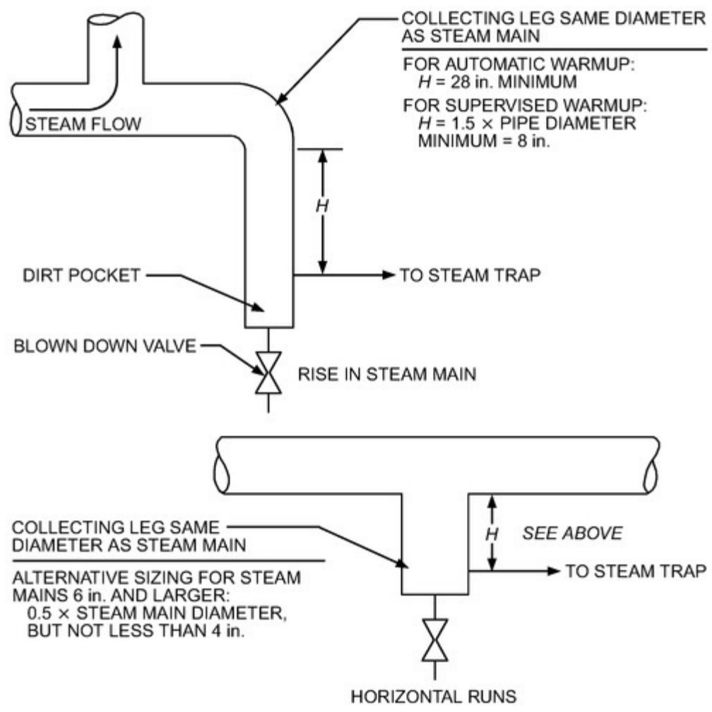
Figure 4. Method of Dripping Steam Mains
