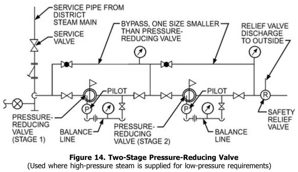
Figure 14. Two-Stage Pressure-Reducing Valve (Used where high-pressure steam is supplied for low-pressure requirements)
