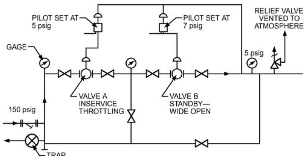
Figure 12. Pressure-Reducing Valve Connections—High Pressure
