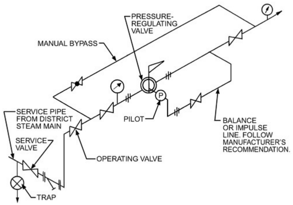
Figure 11. Pressure-Reducing Valve Connections—Low Pressure
