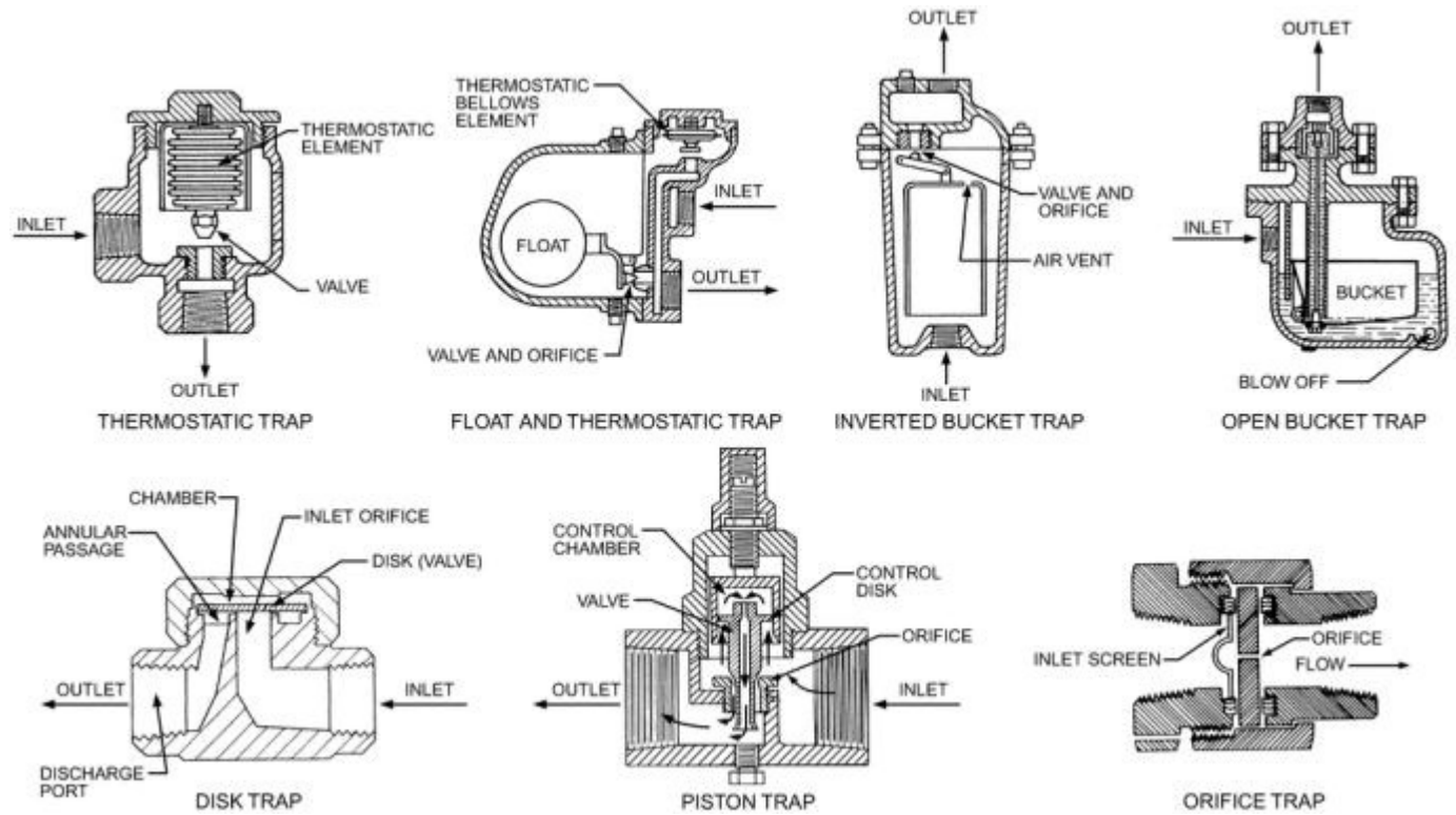
Figure 10. Steam Traps
