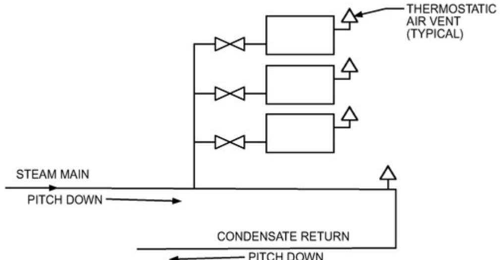
Figure 15. One-Pipe System
