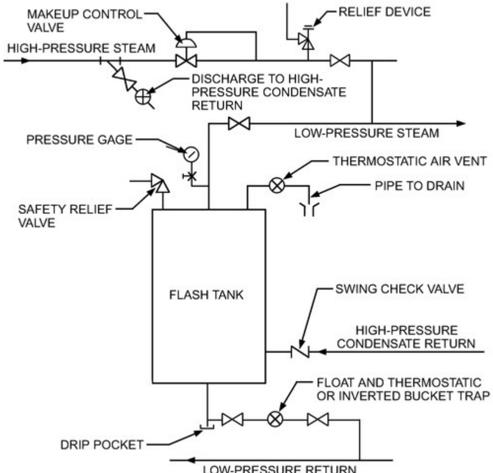
Figure 20. Vertical Flash Tank
