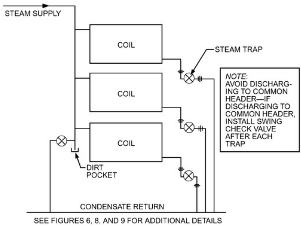
Figure 7. Trapping Multiple Coils
