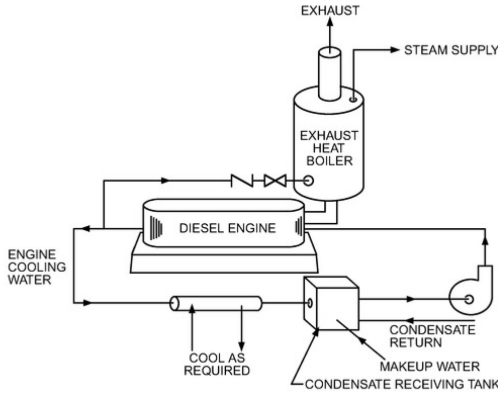
Figure 1. Exhaust Heat Boiler
