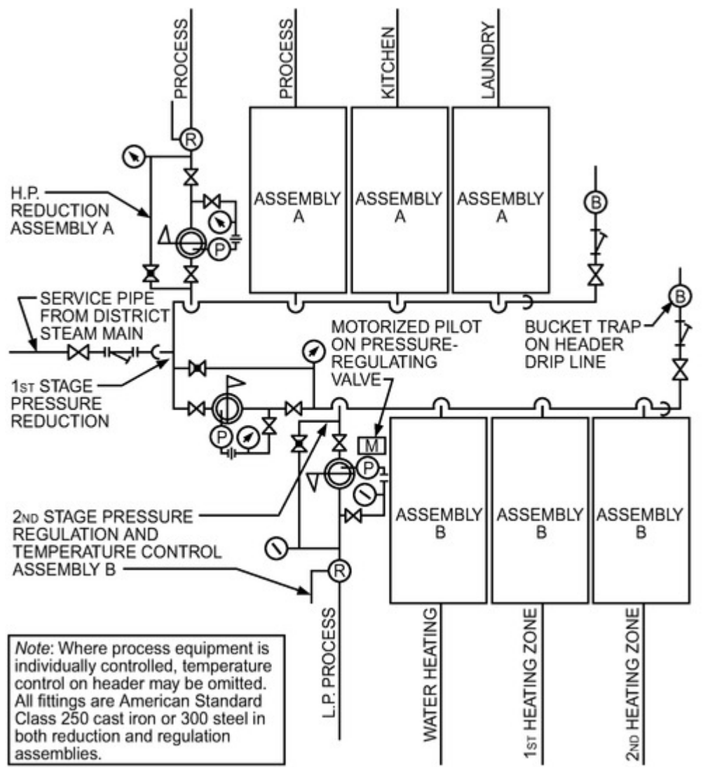
Figure 13. Steam Supply
