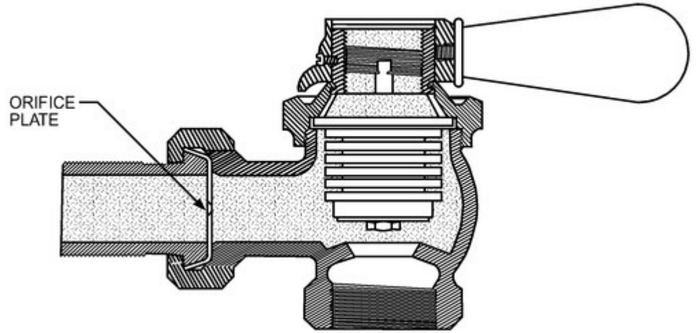
Figure 17. Inlet Orifice
