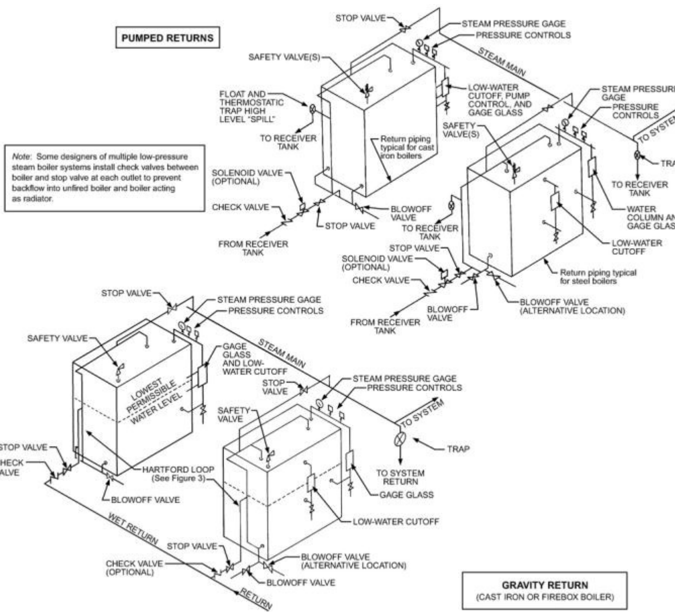
Figure 2. Typical Boiler Connections
