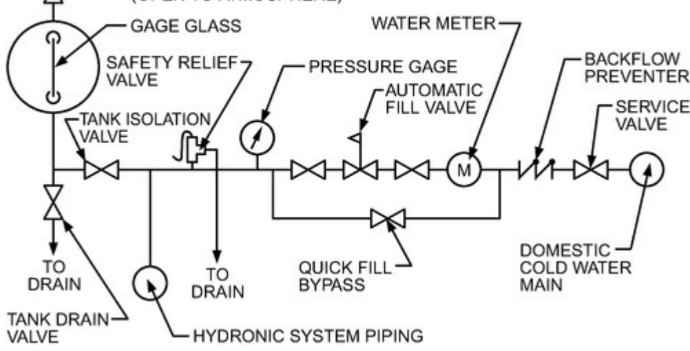
Figure 40. Typical Makeup Water and Expansion Tank Piping Configuration for Plain Steel Expansion Tank
