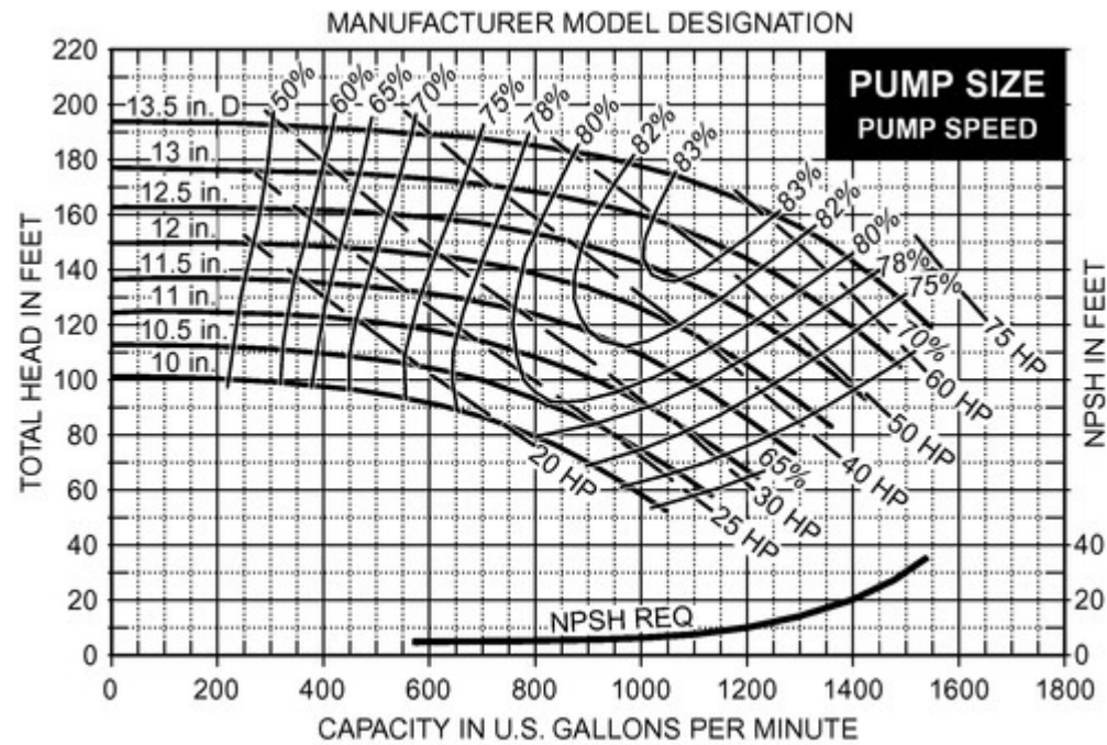
Figure 4. Example of Manufacturer's Published Pump Curve
