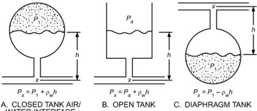
Figure 15. Tank Pressure Related to System Pressure
