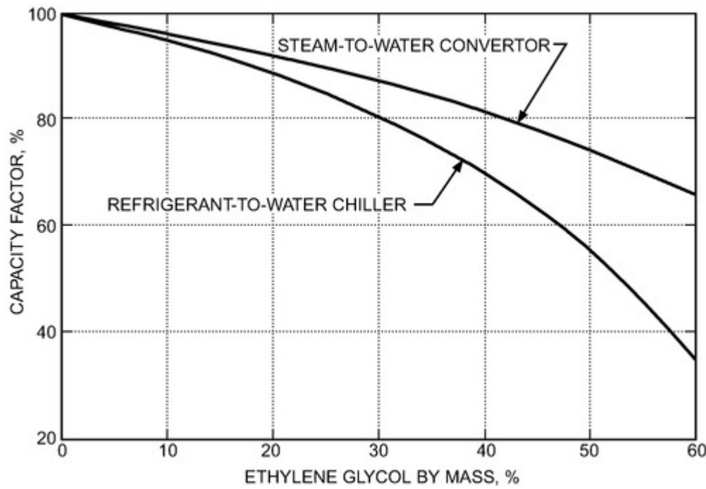
Figure 42. Example of Effect of Aqueous Ethylene Glycol Solutions on Heat Exchanger Output
