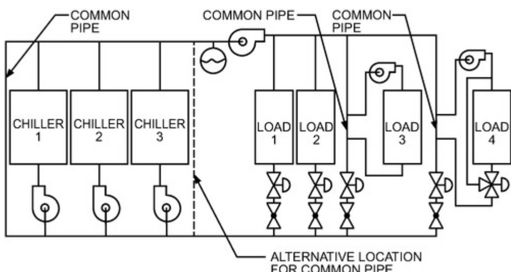
Figure 36. Variable-Flow Chilled-Water System
