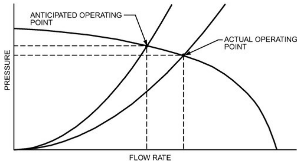
Figure 6. Shift of System Curve Caused by Circuit Unbalance
