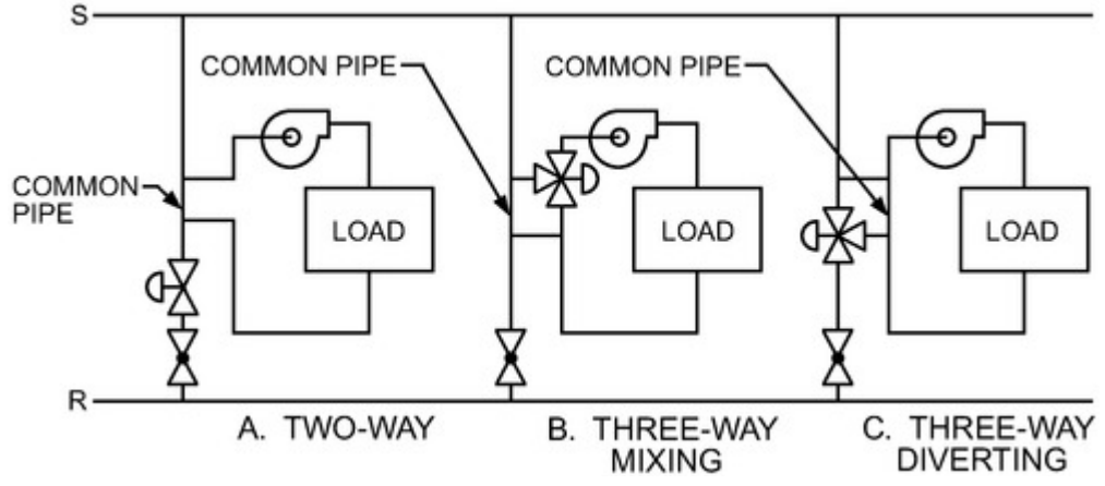
Figure 29. Load Pumps with Valve Control
