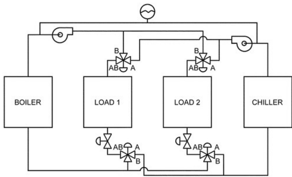
Figure 38. Example Four-Pipe Common Load System
