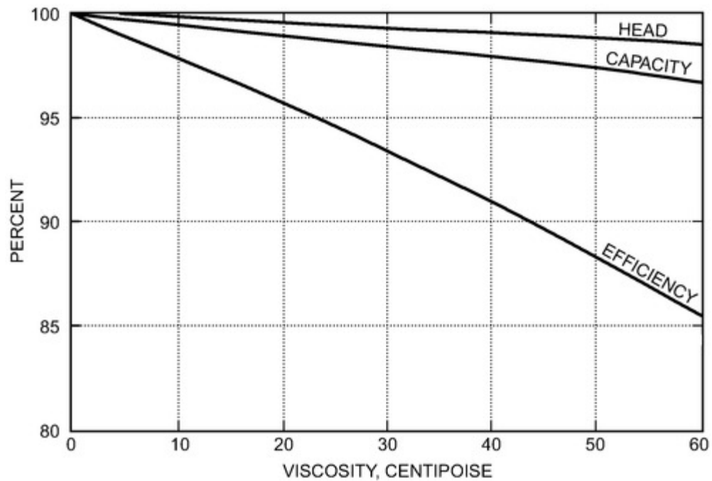
Figure 43. Effect of Viscosity on Pump Characteristics
