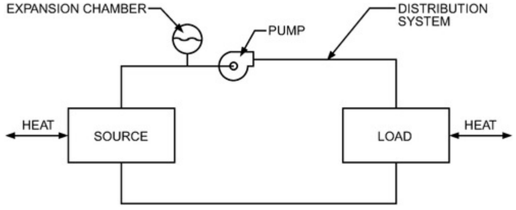
Figure 1. Fundamental Components of Hydronic System
