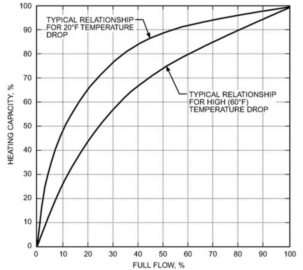
Figure 32. Heat Emission Versus Flow Characteristic of Typical Hot Water Heating Coil
