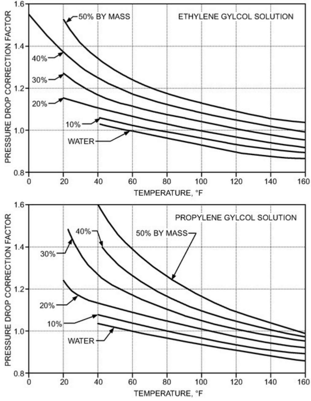
Figure 44. Pressure Drop Correction for Glycol Solutions
