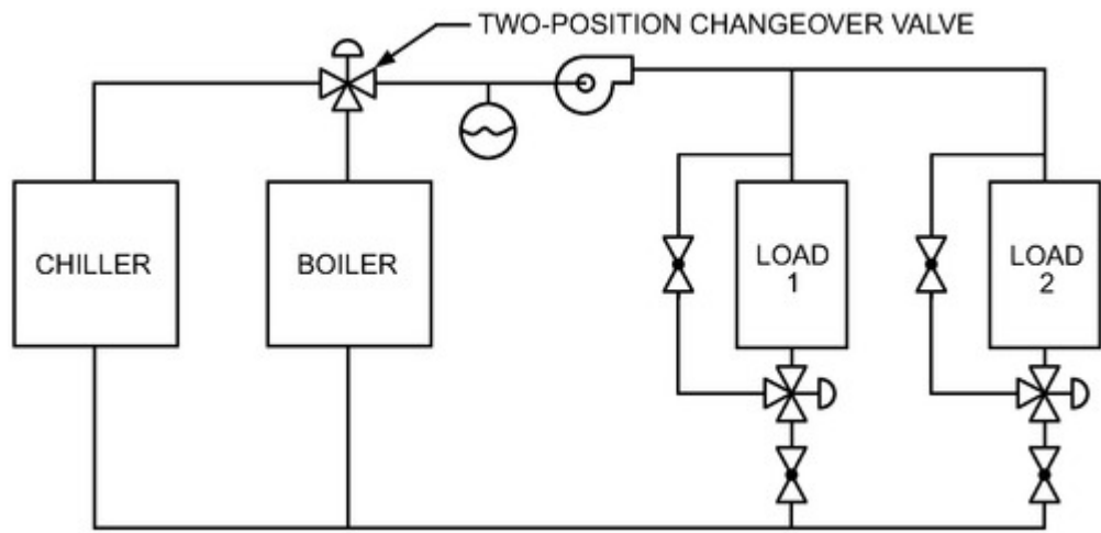
Figure 37. Simplified Diagram of Two-Pipe System
