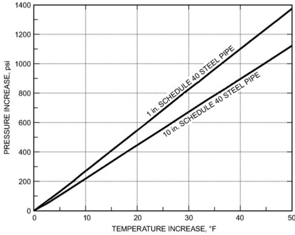
Figure 41. Pressure Increase Resulting from Thermal Expansion as Function of Temperature Increase
