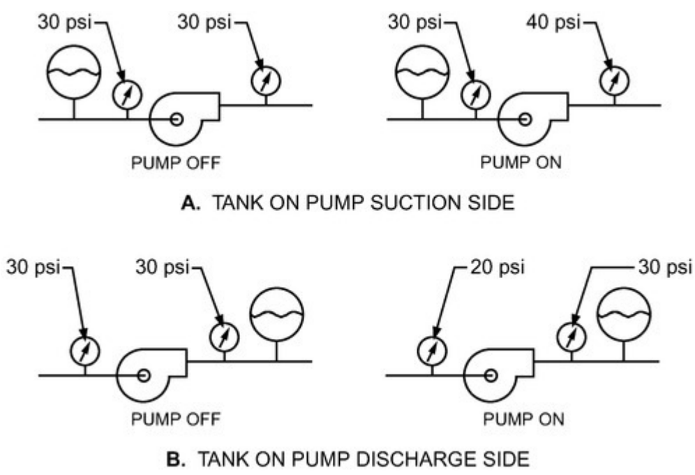
Figure 16. Effect of Expansion Tank Location with Respect to Pump Pressure
