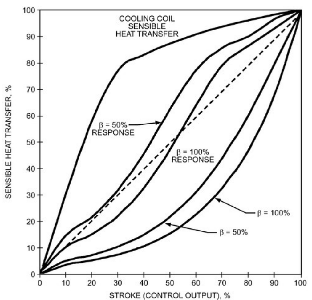
Figure 26. Control Valve and Coil Response, Inherent and 50% Authority
