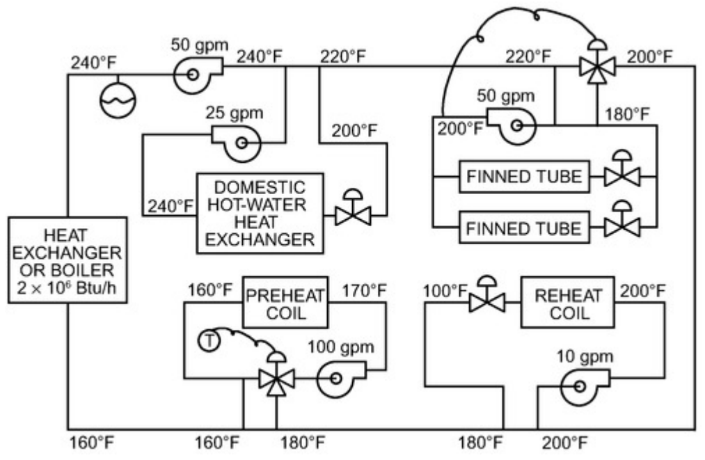
Figure 31. Example of Series-Connected Loading
