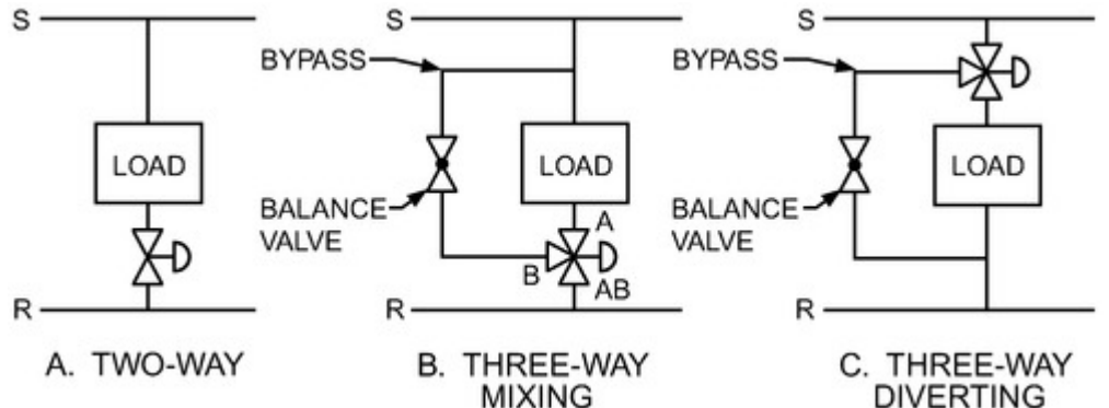
Figure 22. Load Control Valves
