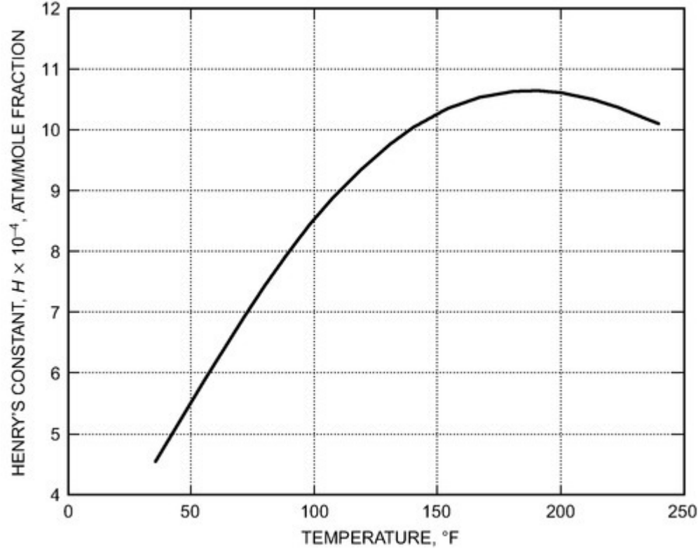
Figure 2. Henry's Constant Versus Temperature for Air and Water (Coad 1980a)
