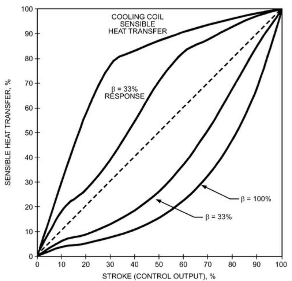
Figure 27. Control Valve and Coil Response, 33% Authority
