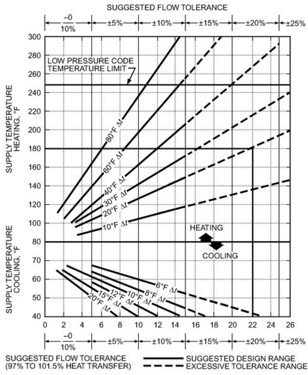
Figure 34. Recommendations for Coil Flow Tolerance to Maintain 97% Design Heat Transfer (Carlson 1981)
