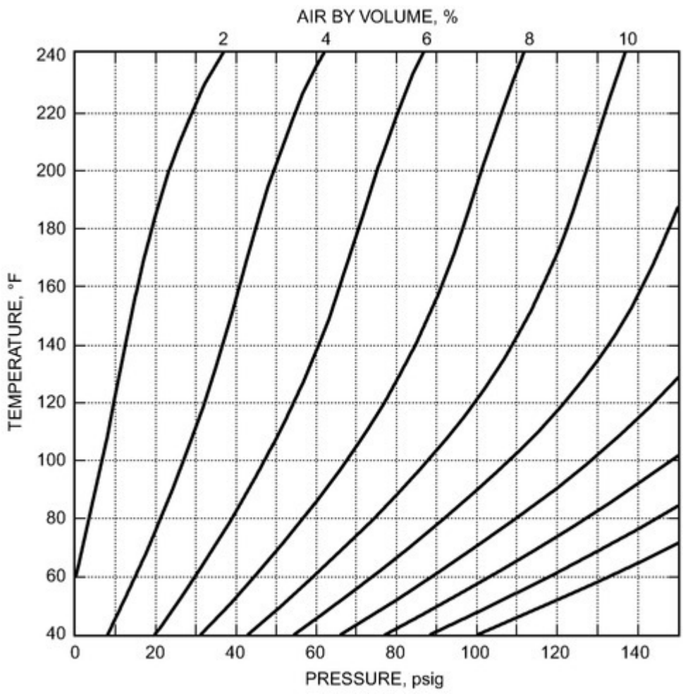
Figure 3. Solubility Versus Temperature and Pressure for Air/Water Solutions (Coad 1980a)
