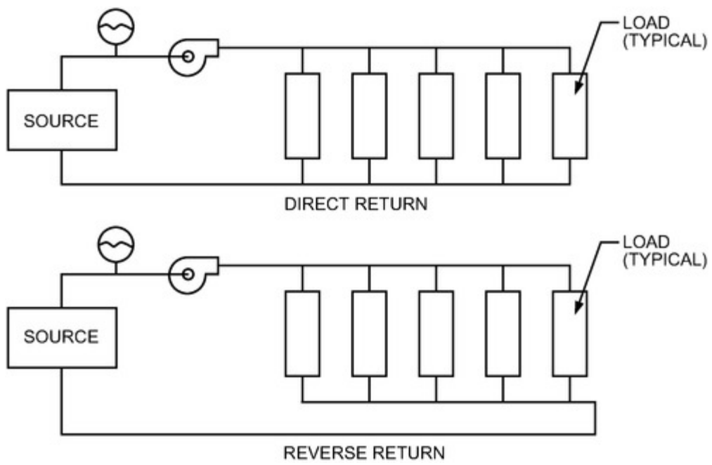
Figure 21. Direct- and Reverse-Return Two-Pipe Systems
