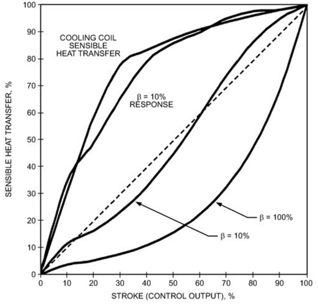
Figure 28. Coil Valve and Coil Response, 10% Authority
