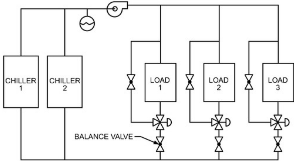
Figure 35. Constant-Flow Chilled-Water System
