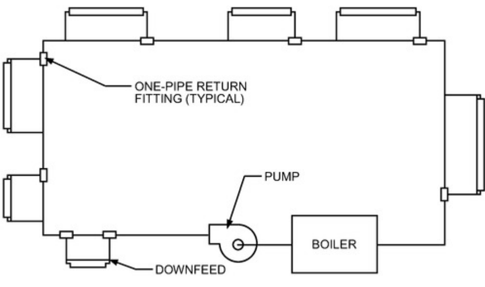
Figure 19. One-Pipe Diverting Tee System
