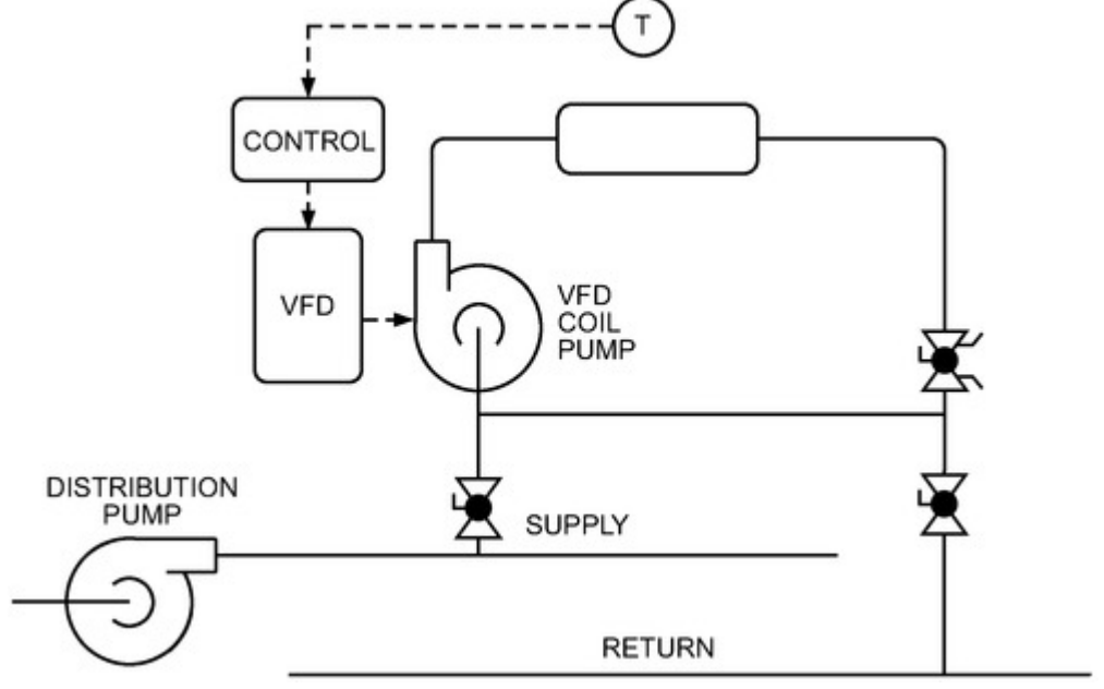
Figure 30. Schematic of Variable-Speed Pump Coil Control
