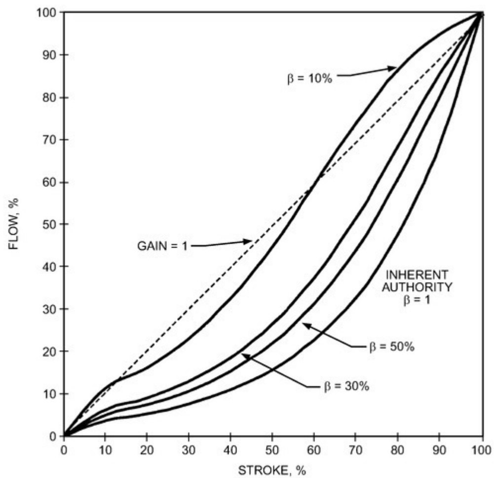
Figure 25. Equal-Percentage Valve Characteristic with Authority
