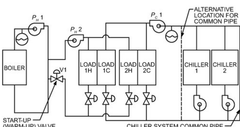
Figure 39. Four-Pipe Independent Load System
