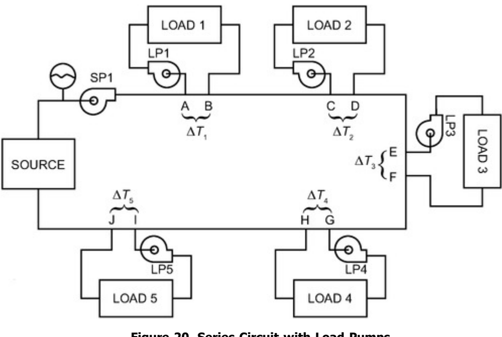
Figure 20. Series Circuit with Load Pumps
