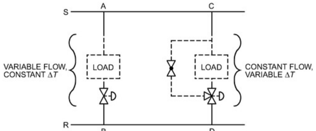
Figure 23. System Flow with Two-Way and Three-Way Valves
