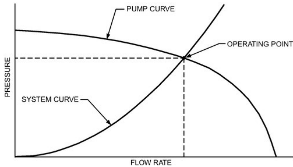
Figure 5. Pump Curve and System Curve
