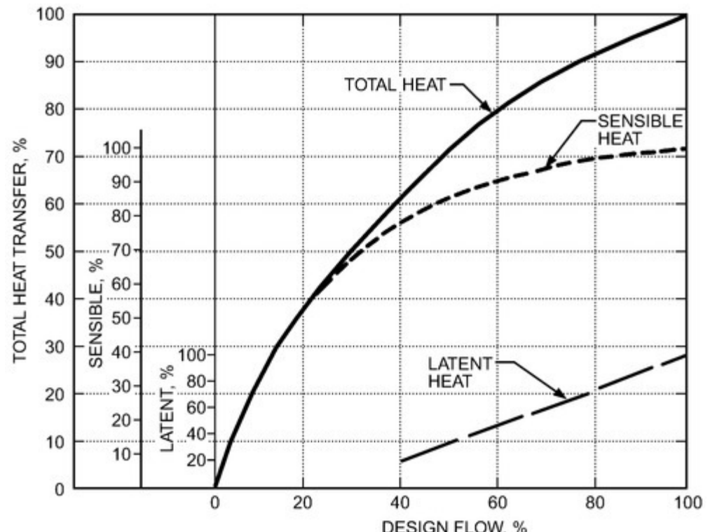
Figure 33. Generic Chilled-Water Coil Heat Transfer Characteristic
