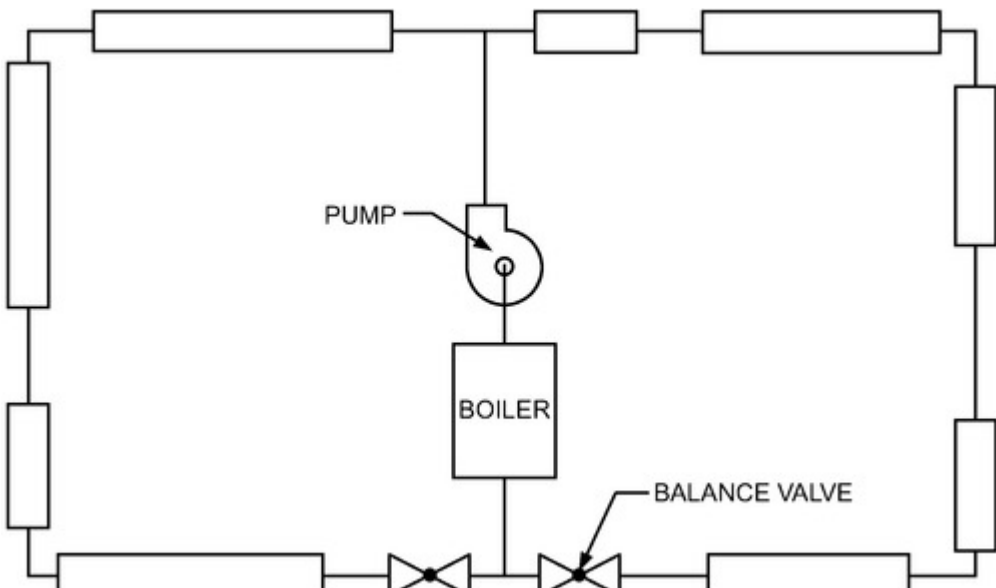
Figure 18. Series Loop System
