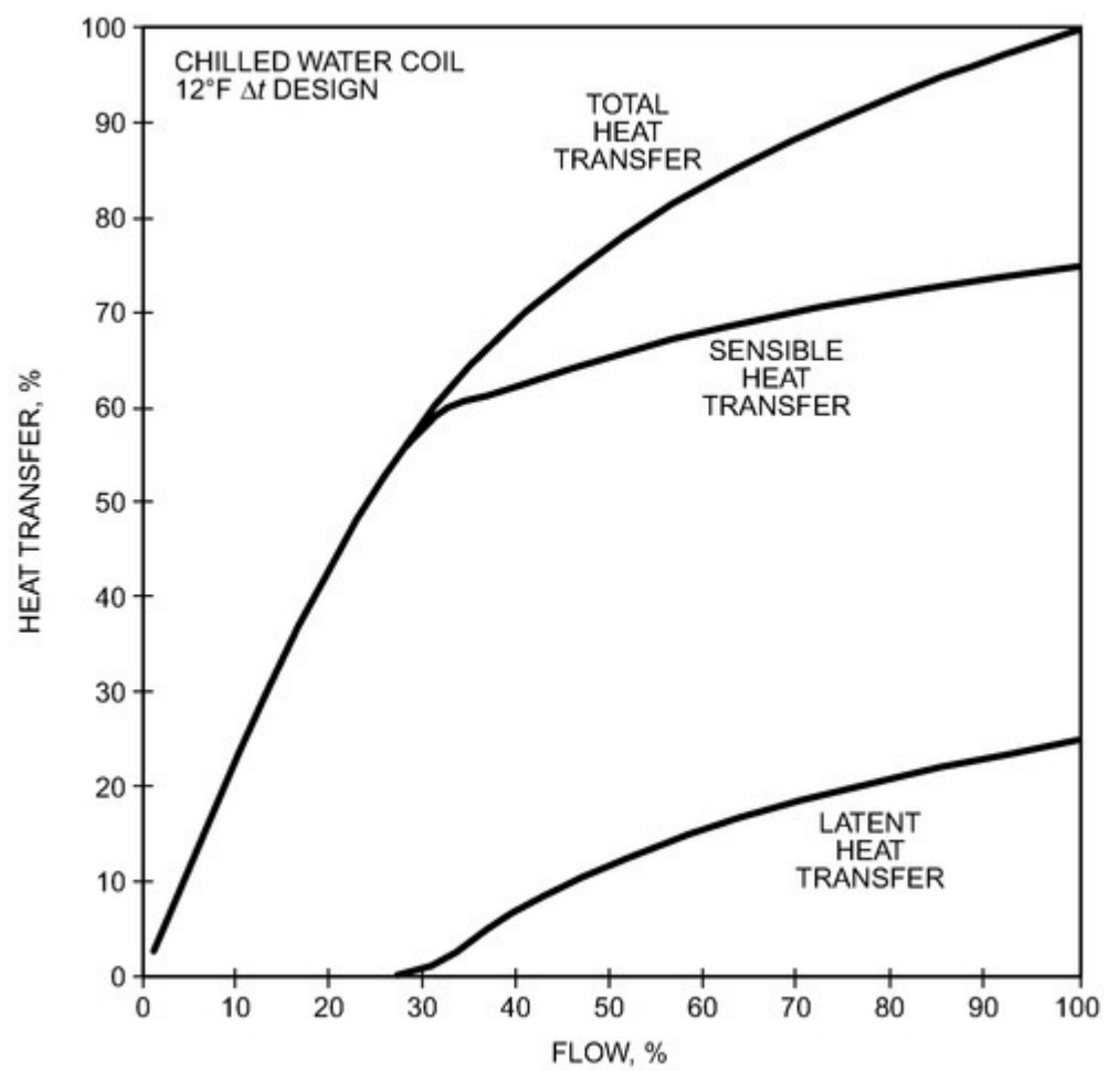
Figure 24. Chilled-Water Coil Heat Transfer Characteristic
