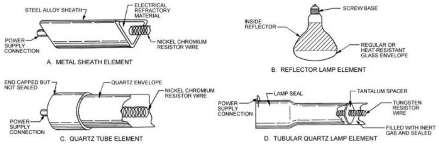
Figure 2. Common Electric Infrared Heaters
