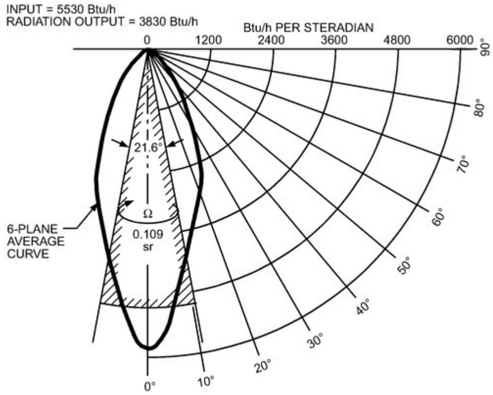
Figure 6. Radiant Heat Flux Distribution Curve of Typical Narrow-Beam High-Intensity Electric Infrared Heaters
