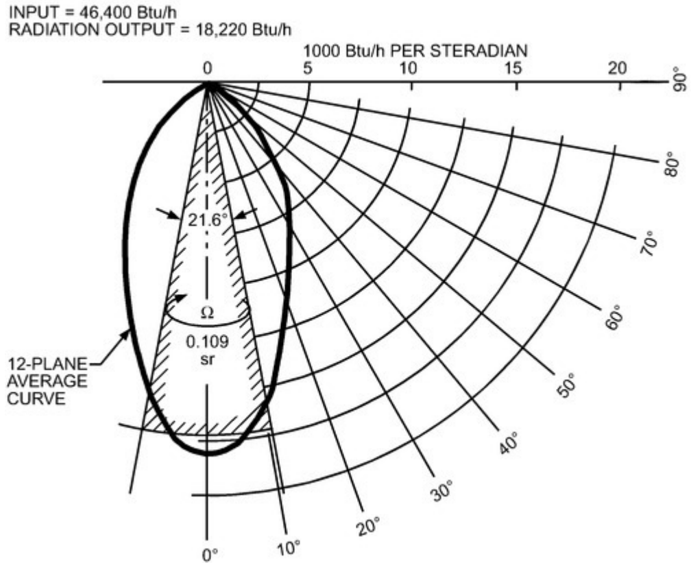
Figure 8. Radiant Heat Flux Distribution Curve of Typical Narrow-Beam High-Intensity Atmospheric Gas-Fired Infrared Heaters
