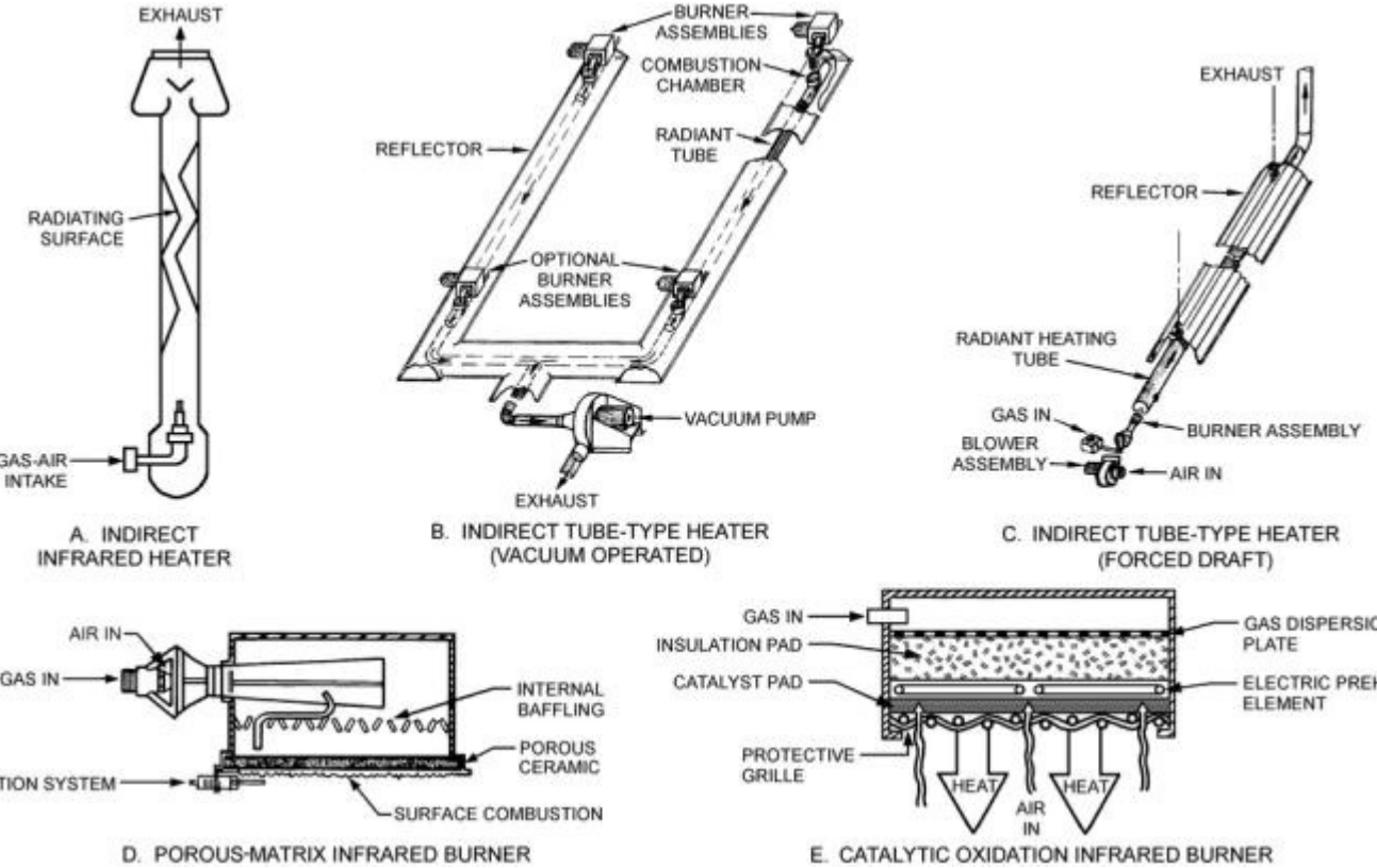
Figure 1. Types of Gas-Fired Infrared Heaters
