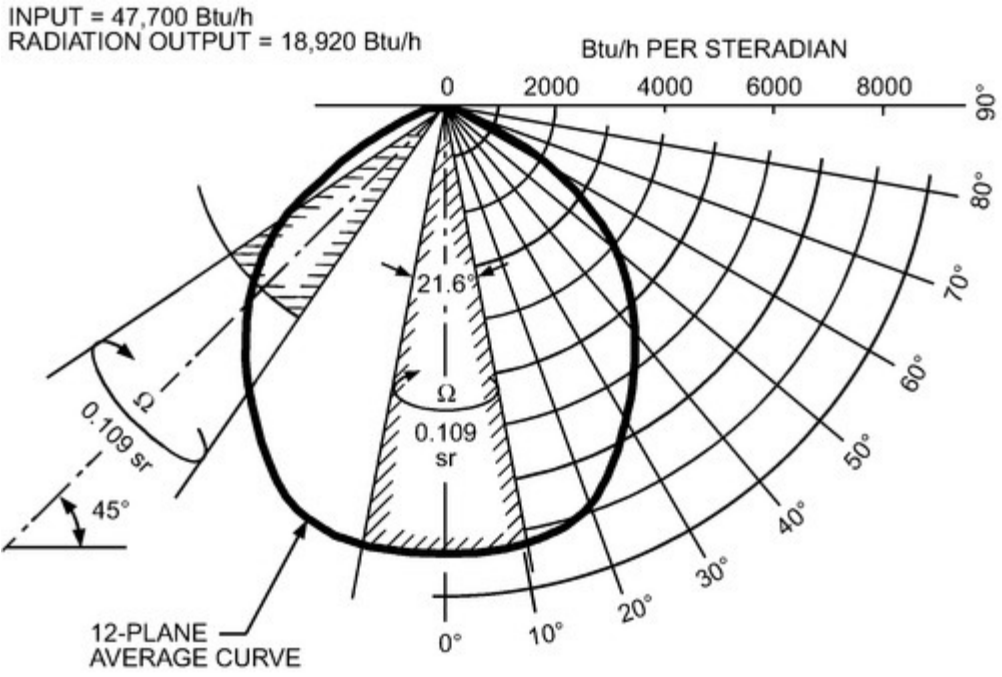
Figure 9. Radiant Heat Flux Distribution Curve of Typical Broad-Beam High-Intensity Atmospheric Gas-Fired Infrared Heaters
