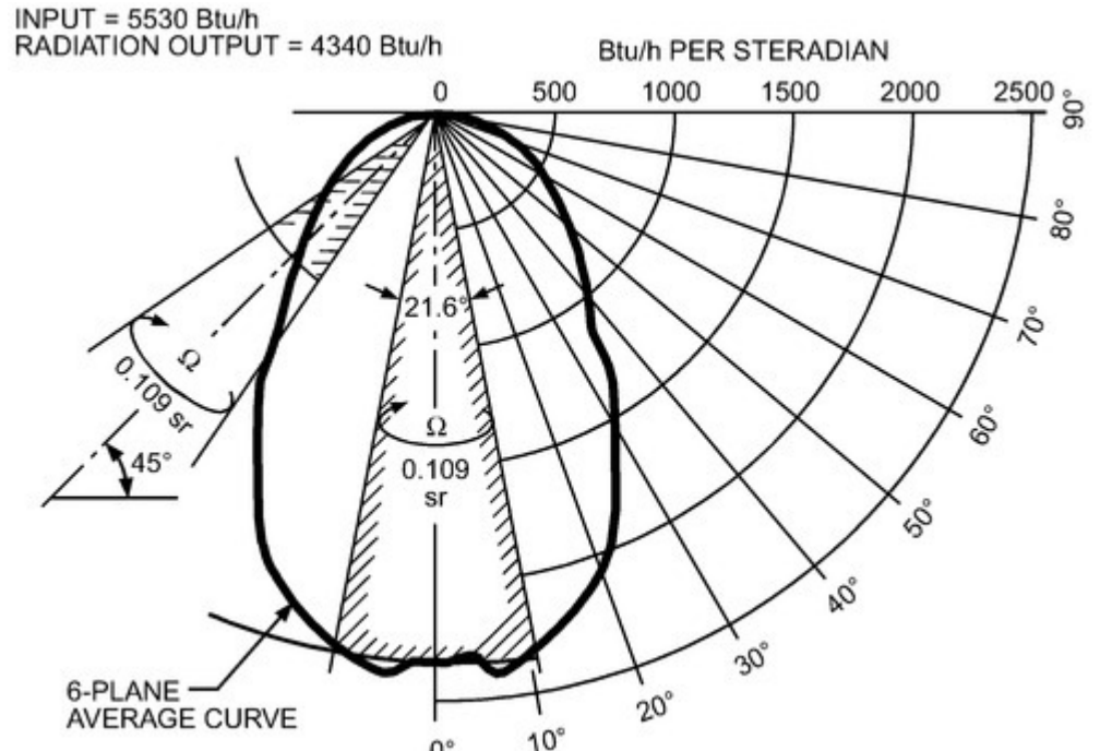
Figure 7. Radiant Heat Flux Distribution Curve of Typical Broad-Beam High-Intensity Electric Infrared Heaters
