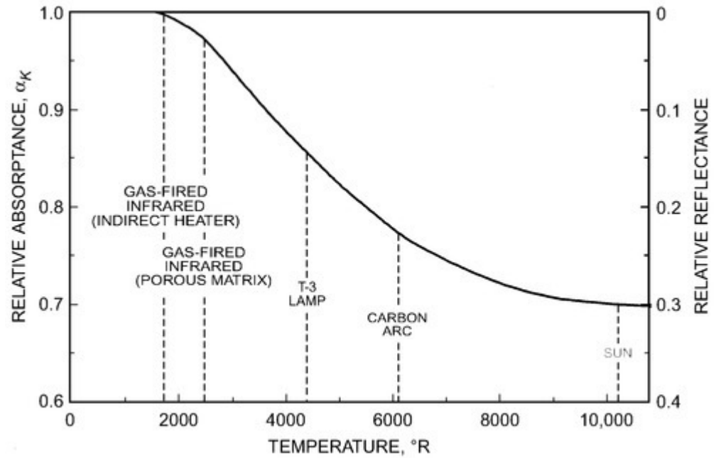
Figure 3. Relative Absorptance and Reflectance of Skin and Typical Clothing Surfaces
